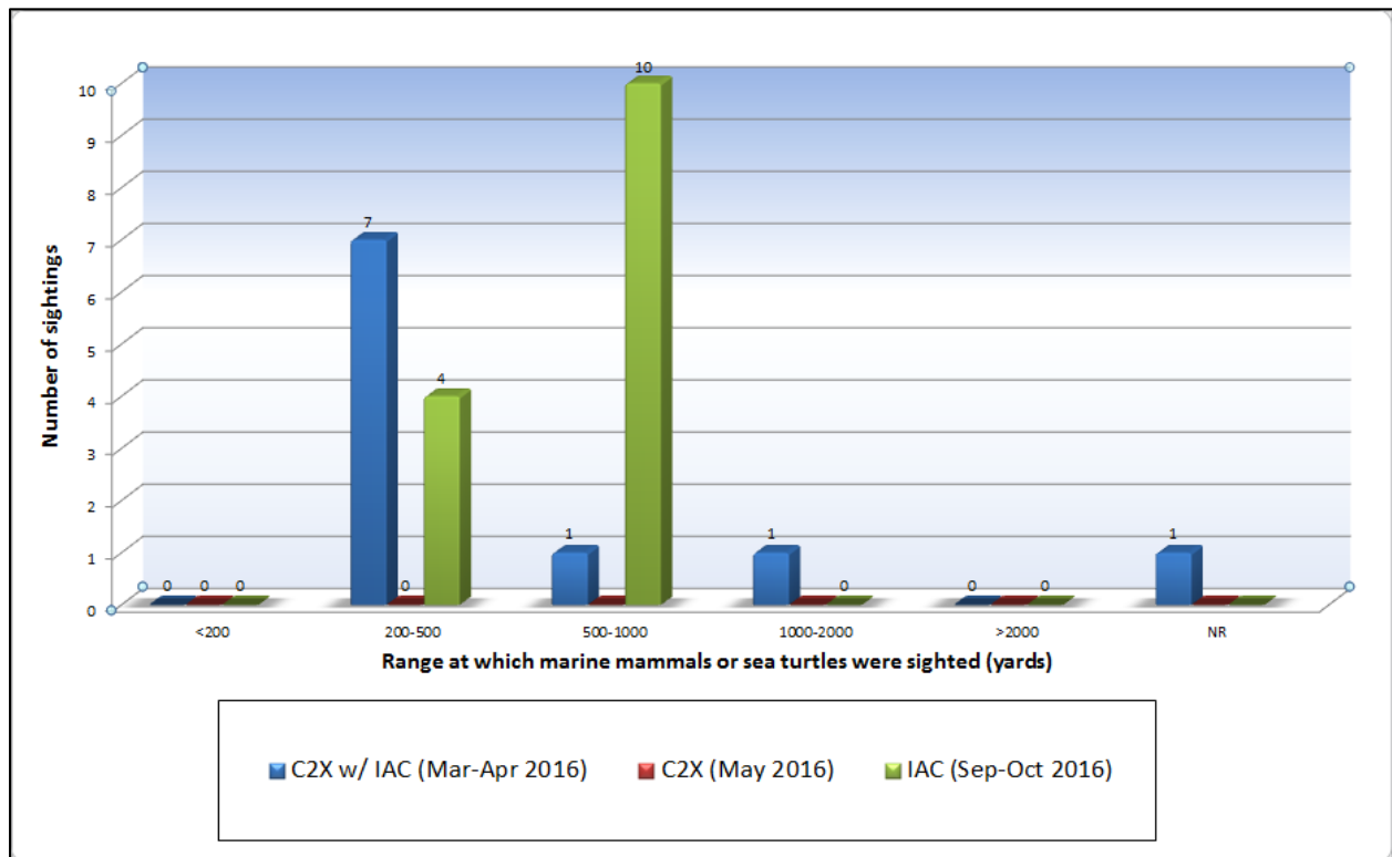
Figure 1-iii-1. Marine mammal and sea turtle mitigation sightings by range and MTE in the AFTT Study Area
