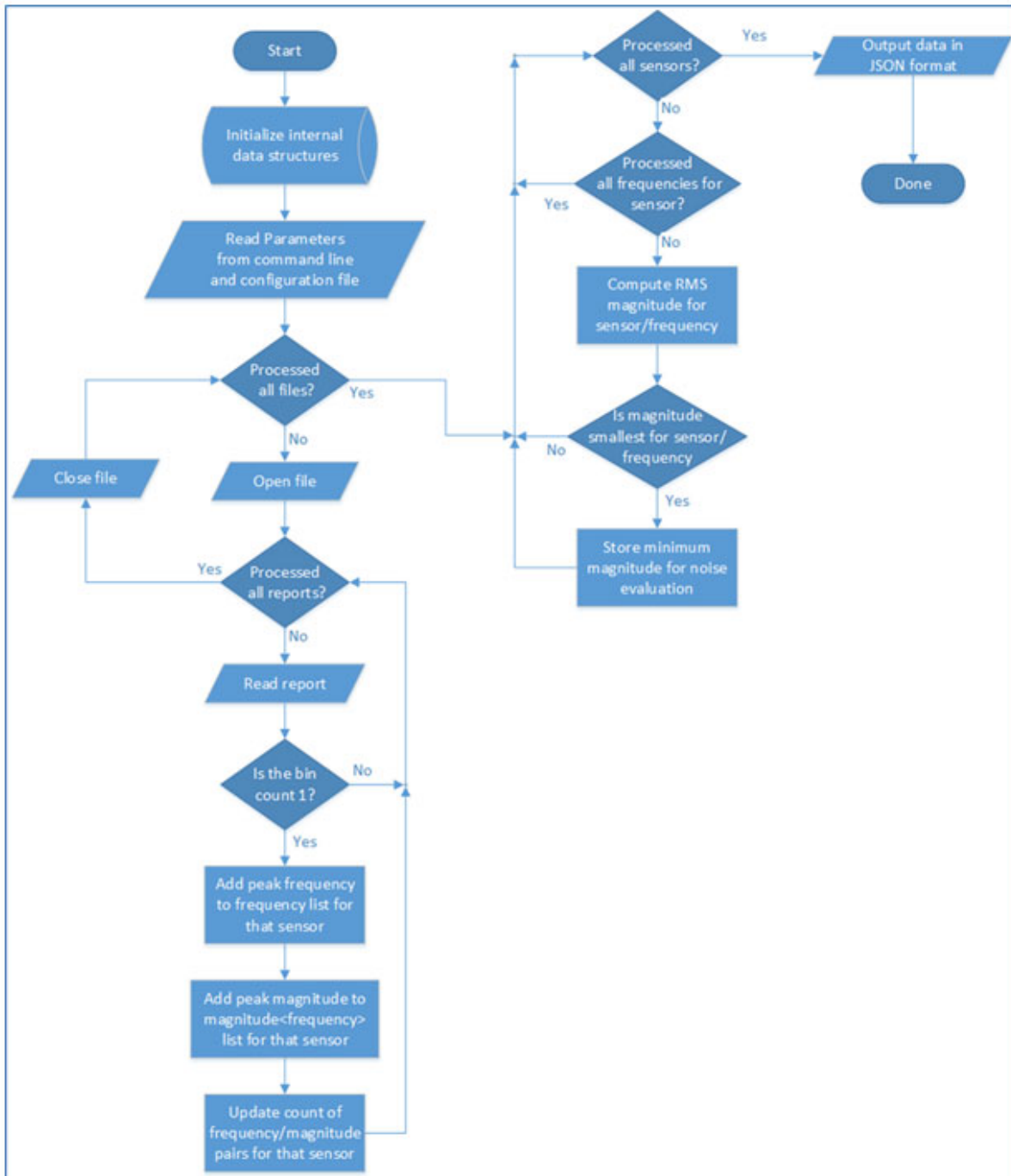
Figure 29. Flowchart for Ambient Noise “Sprinkle” Algorithm (Morrissey, 2021)
