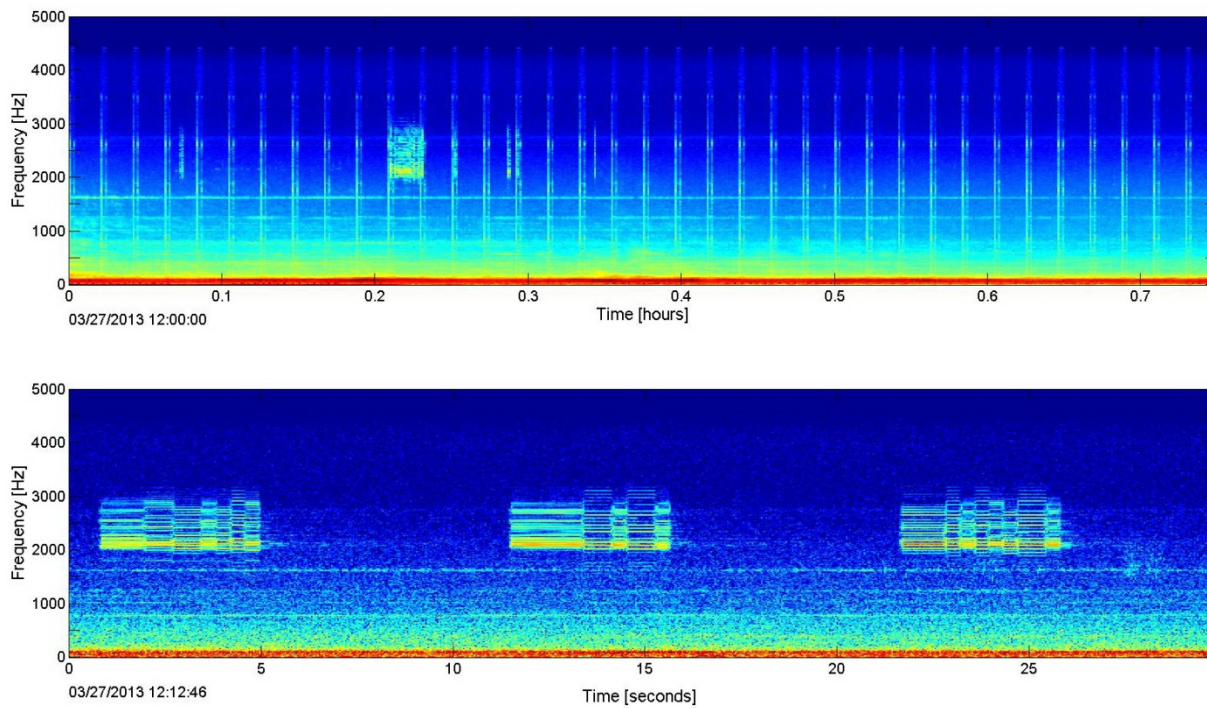
Figure 30. Electronic underwater communications in the LTSA (top) and spectrogram (bottom).
