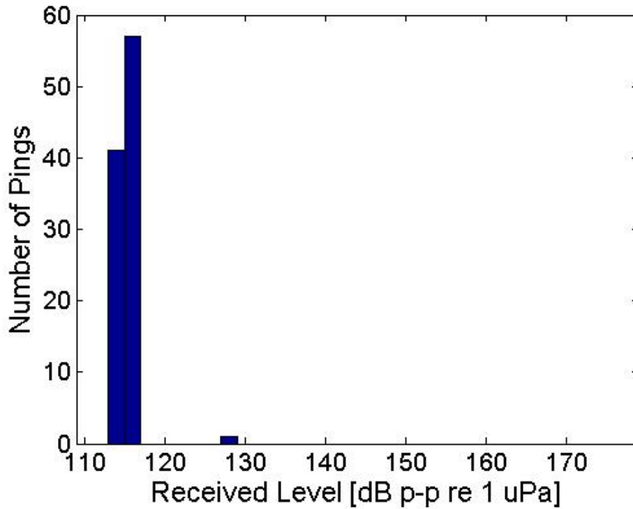
Figure 75. Distribution of the number of MFA sonar pings below 5 kHz by received levels in 1 dB bins.
