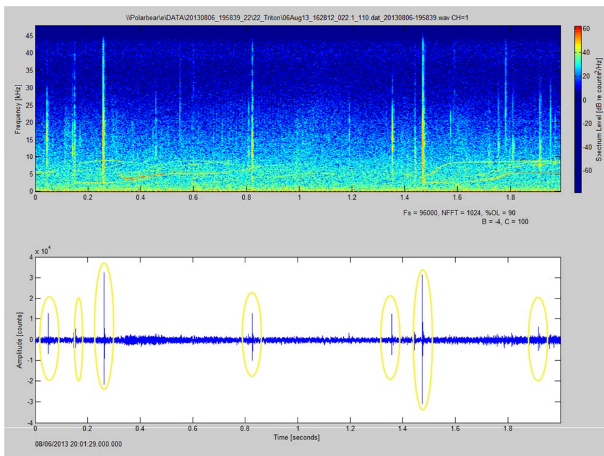
Figure 1. Spectrogram and waveform view of false killer whale echolocation clicks in Triton software. Yellow circles are echolocation clicks that were logged. Clicks that are not circled are faint and/or multipath signals that were not logged.
