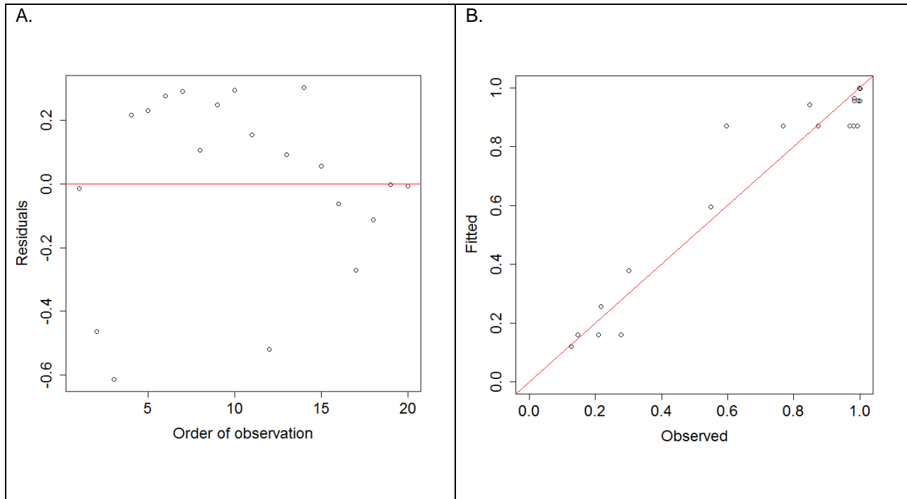
Figure 4. Diagnostics for dolphin PSTGAE model 2 – whistle model with Site, Type 1 Long, Buzzes and Clicks as the predictors (PSTGAE model 2). (A.) the means of binned fitted values the means of corresponding residuals. Binning occurred by splitting the fitted values into 20 equally sized bins in ascending order of observation. (B.) mean observed versus mean fitted values from presence/absence of cetacean acoustic detections. No trend in the pattern of the residuals is desired in A, and most of the points lying close to the line is desired in B.
