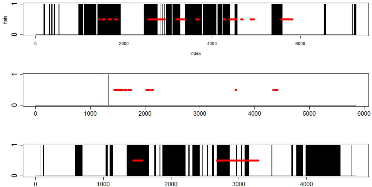
Figure 7: HARP time series of of 1-minute segments where black bars indicate sperm whale acoustic detections and white indicates absence of acoustic signal. Data include NAs (i.e. time points where data are missing). The Y-axis gives the value the binary variable takes for a given observation (0 or 1); the X-axis indexes the observations in the time series. From top to bottom – HAT01A, USWTR05A and USWTR06E. Red dots signify occurrence of sonar events.
