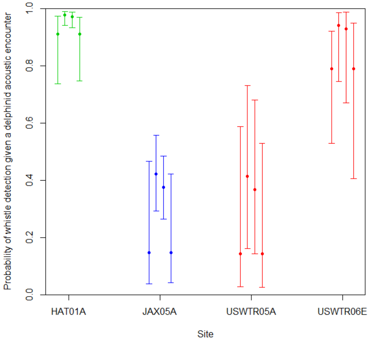
Figure 18. Predicted probability of whistle detection given delphinid acoustic activity from a model with Site, Sonar, Buzzes and Clicks as predictors (from PSTGAE model 1). Predictions assume Clicks = 1 (presence) Buzzes = 1 (presence). Vertical bars indicate 99% confidence intervals. For each site, predictions are shown here (from left to right) for “before,” “during,” “between,” and “after” sonar activity, respectively.
