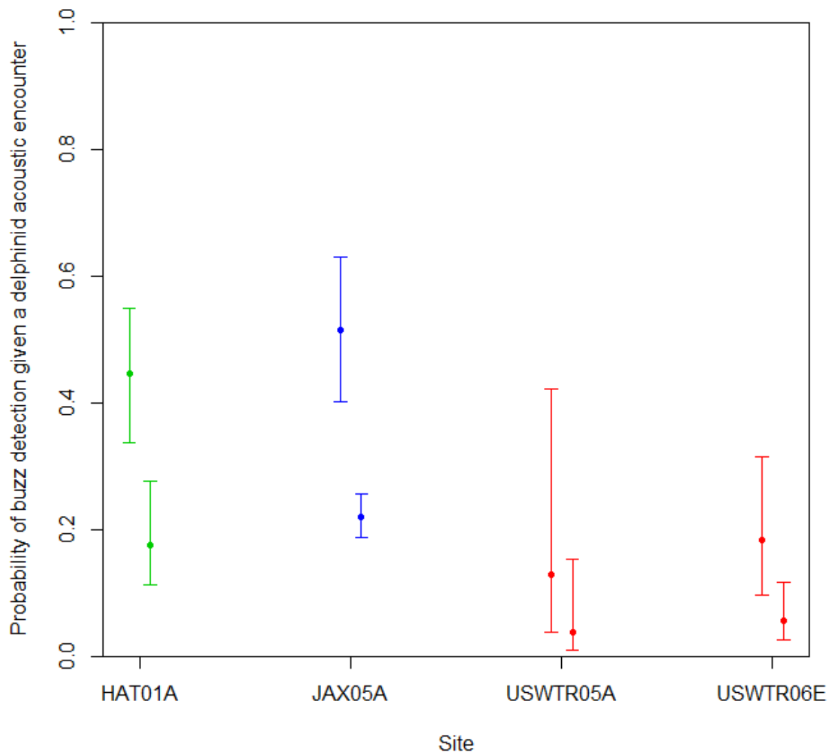
Figure 26. Predicted probability of buzz detection given delphinid acoustic activity in a model (PSTGAE model 6) with Site , Clicks , Whistles , Type 3 med sonar signals . Vertical bars indicate 99% confidence intervals. For each site, predictions are shown for Whistles and Clicks = 1 (assumed present).
