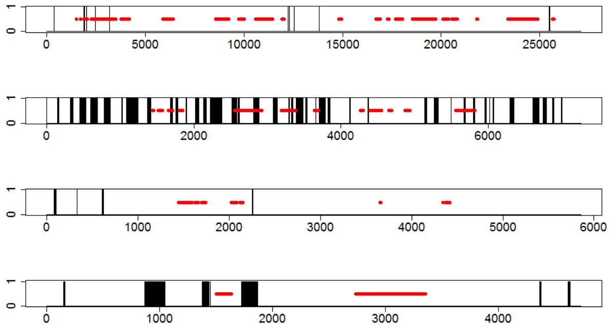
Figure 5. HARP time series of 1-minute segments where black bars indicate occurrence of beaked whale acoustic signals and white indicates absence of acoustic signals. Data include NAs (i.e., time points where data are missing). The Y-axis gives the value the binary variable takes for a given observation (0 or 1); the X-axis indexes the observations in the time series. From top to bottom – JAX05A, HAT01A, USWTR05A and USWTR06E. Red dots signify occurrence of sonar events.
