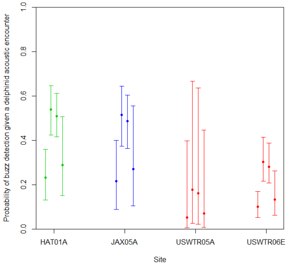
Figure 25. Predicted probability of buzz detection given delphinid acoustic activity with Site, whistles, Clicks and Sonar as predictors (PSTGAE model 5). Vertical bars indicate 99% confidence intervals. For each site, predictions are shown for “before,” “during,” “between” and “after” MFA sonar events, respectively, with Whistles and Clicks = 1 (assumed present).
