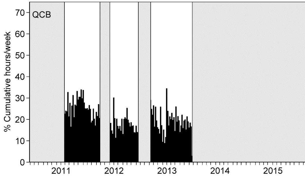
Figure 11. NWTRC percent cumulative hours per week of broadband (nearby) ship sound detections over the deployment periods. Early CE and QCA were not analyzed for broadband ship sounds (Table 2).
