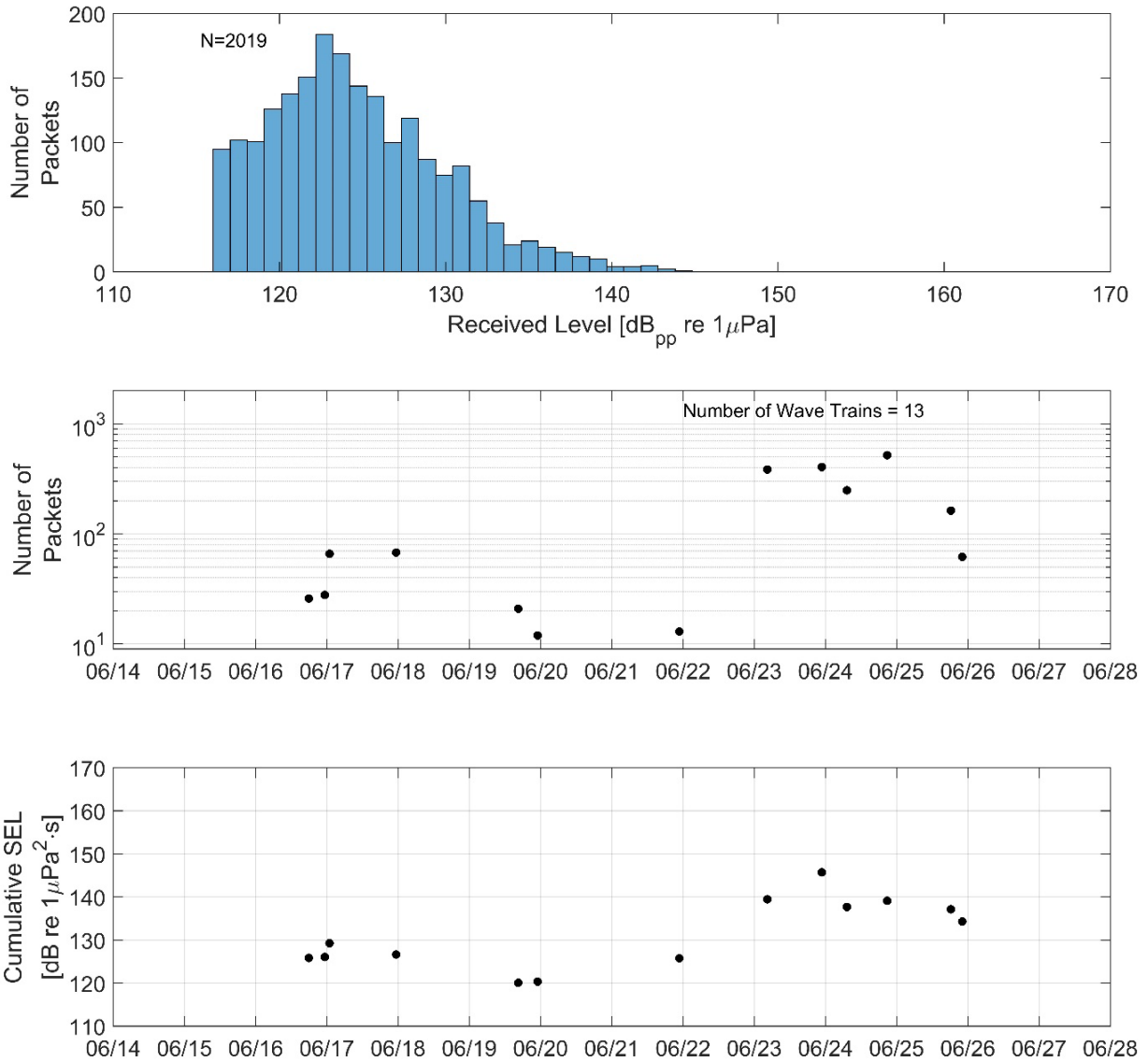
Figure 12. GATMAA site CB MFA metrics. Top: Distribution of received peak-to-peak sound pressure levels of detected MFA packets. Center: Number of MFA packets detected in each wave train exceeding 116 dB re 1 μPa. Bottom: Cumulative sound exposure levels (CSEL) of each wave train event.
