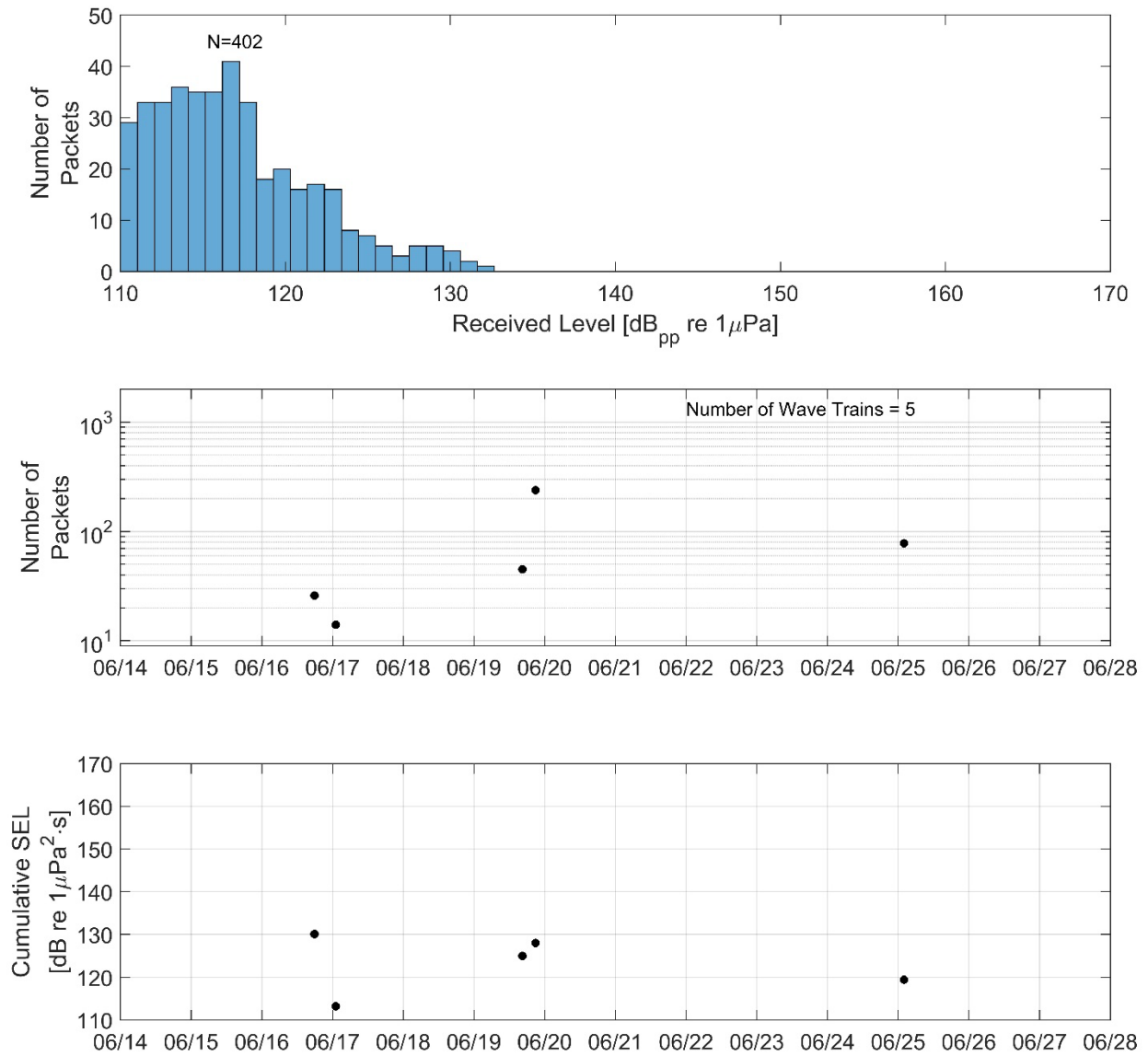
Figure 13. GATMAA site QN MFA metrics. Top: Distribution of received peak-to-peak sound pressure levels of detected MFA packets. Center: Number of MFA packets detected in each wave train exceeding 110 dB re 1 μPa. Bottom: Cumulative sound exposure levels (CSEL) of each wave train event.
