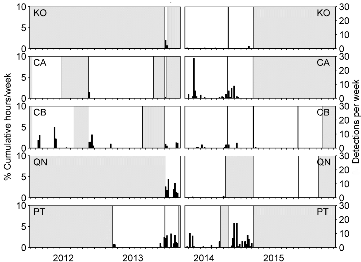
Figure 15. GATMAA explosion detections. Analyst manual visual detections on left, automatic computer algorithm detections on right.
