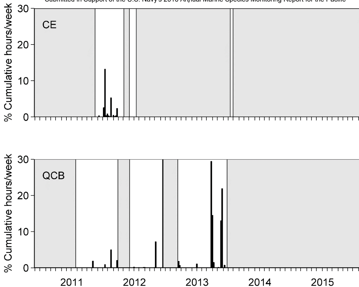
Figure 16. NWTRC explosion detection via analyst visual method. Not shown are the results from the automatic computer algorithm method used for CE during 2013 which detected 200 – 500 detections per week as the metrics were different and were over a very short duration. Early CE and QCA were not analyzed for explosions (Table 2).
