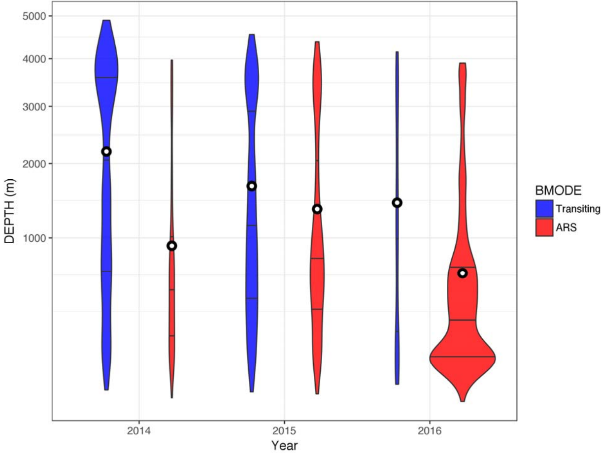
Figure 54. Paired violin plots of seafloor depth (DEPTH, m) values in CCAL for blue whale locations classified as transiting and ARS for each year in the study. Horizontal lines inside each violin indicate the quartiles of the data distribution and white circle with black outline indicates the mean. Data were square-root-transformed to improve visualization.
