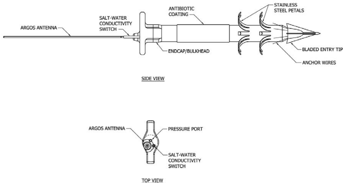
Figure 2. Schematic diagram of the Telonics RDW-665 DM tag showing the main body, the distal endcap with the antenna and saltwater conductivity switch endcap, as well as the penetrating tip and anchoring system.
