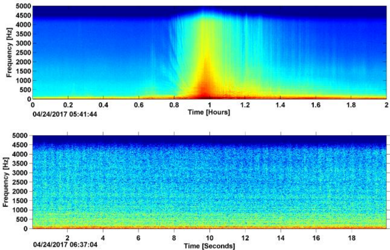
Figure 29. Broadband ships in LTSA (top) and spectrogram (bottom) recorded at NFC Site A, May 2017.
