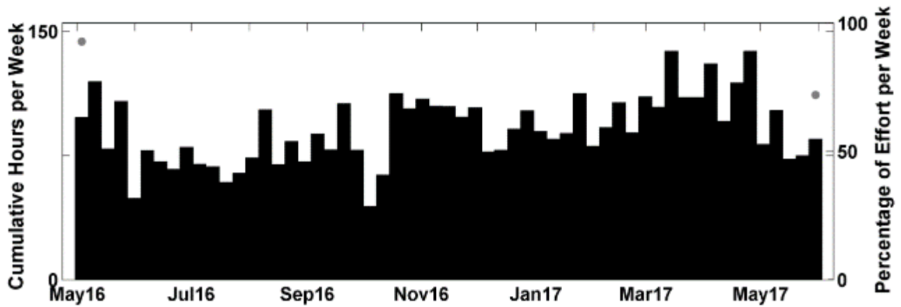
Figure 62. Weekly presence of CT 1 between April 2016 and June 2017 at NFC Site A. Effort markings are described in Figure 39.
