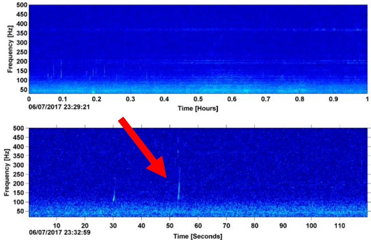
Figure 10. Right whale up-calls in the LTSA (top) and spectrogram (bottom) recorded at NFC Site A, June 2017.
