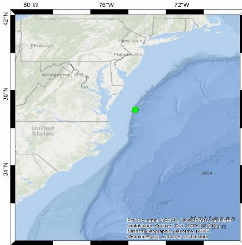
Figure 1: Location of High-Frequency Acoustic Recording Package (HARP) at NFC Site A (37° 09.991 N, 74° 27.996 W, depth 968 m) deployed offshore from Norfolk Canyon study area from April 2016 to June 2017.
