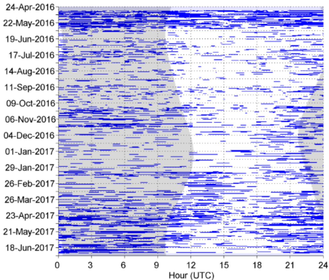
Figure 71. Unidentified odontocete whistles greater than 10 kHz in five-minute bins between April 2016 and June 2017 at NFC Site A. Gray vertical shading denotes nighttime.
