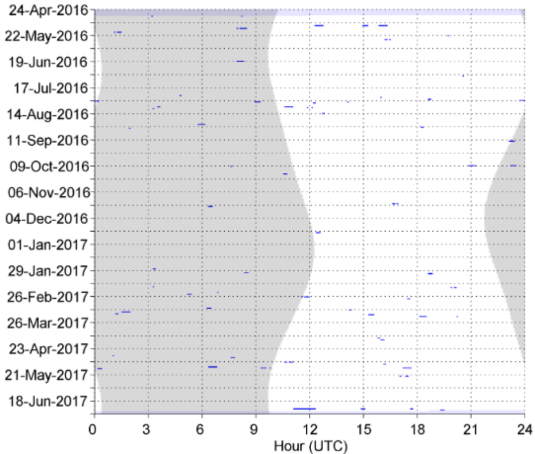
Figure 53. Cuvier's beaked whale echolocation clicks in one-minute bins between April 2016 and June 2017 at NFC Site A. Gray vertical shading denotes nighttime.
