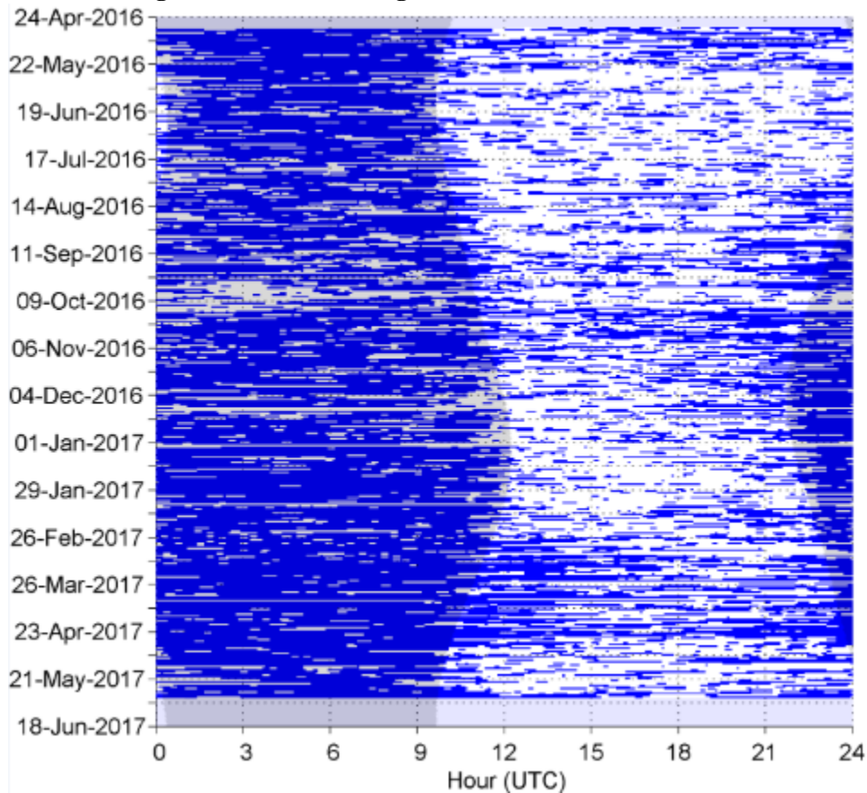
Figure 61. Unidentified odontocete clicks in five-minute bins between April 2016 and June 2017 at NFC Site A. Gray vertical shading denotes nighttime.
