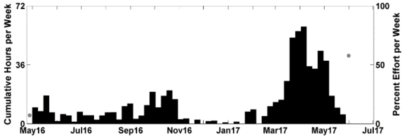
Figure 58. Weekly presence of Risso's dolphin echolocation clicks between April 2016 and June 2017 at NFC Site A. Effort markings are described in Figure 39.
