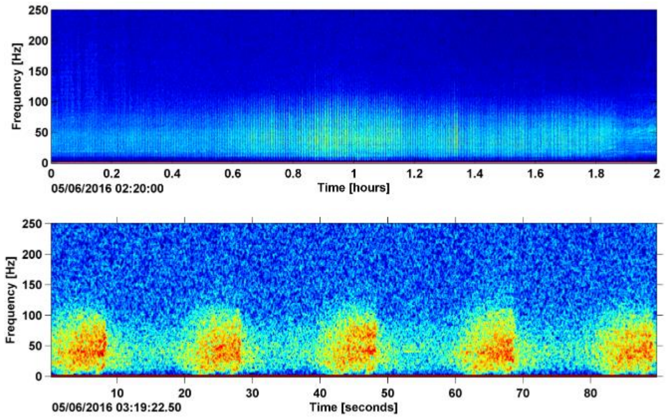
Figure 36. Airguns in LTSA (top) and spectrogram (bottom) recorded at NFC Site A, May 2016.
