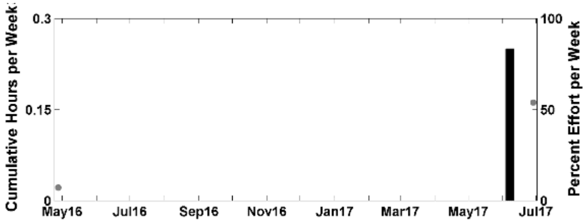
Figure 48. Weekly presence of Northern Atlantic right whale up calls between April 2016 and June 2017 at NFC Site A. Effort markings are described in Figure 39.
