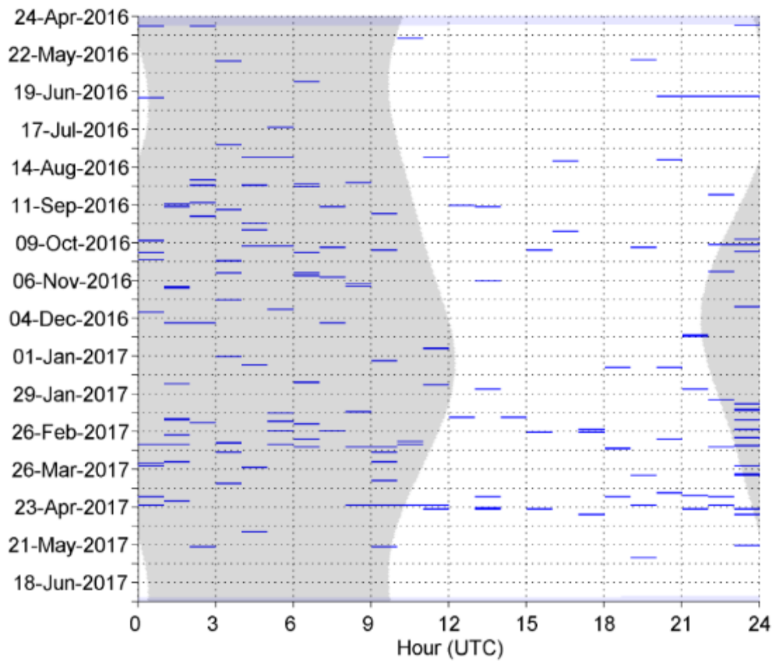
Figure 43. Fin whale 40 Hz calls in hourly bins at NFC Site A. Gray vertical shading denotes nighttime.
