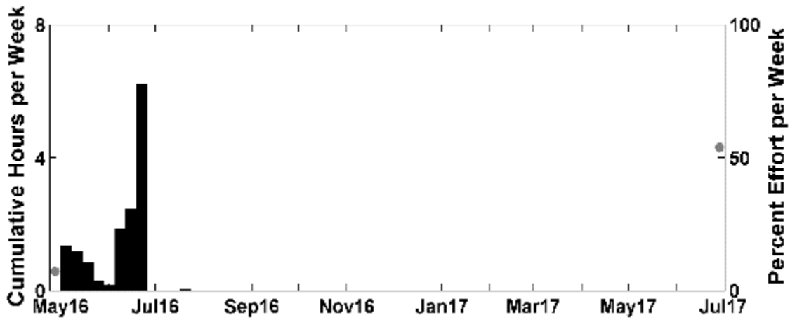
Figure 91. Weekly presence of airguns detected between April 2016 and June 2017 at NFC Site A. Effort markings are described in Figure 39.
