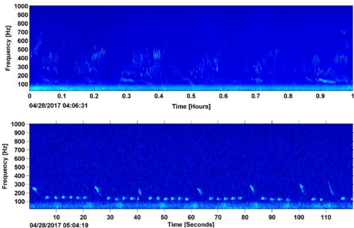
Figure 11. Humpback whale calls in the LTSA (top) and spectrogram (bottom) recorded at NFC Site A, April 2017.
