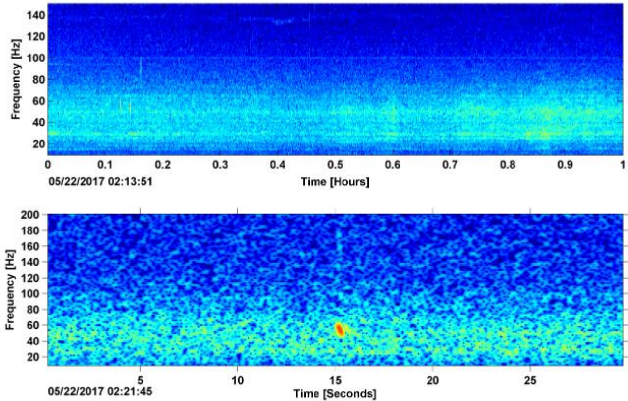
Figure 7. Fin whale 40 Hz call in LTSA (top) and spectrogram (bottom) at NFC Site A, May 2017.
