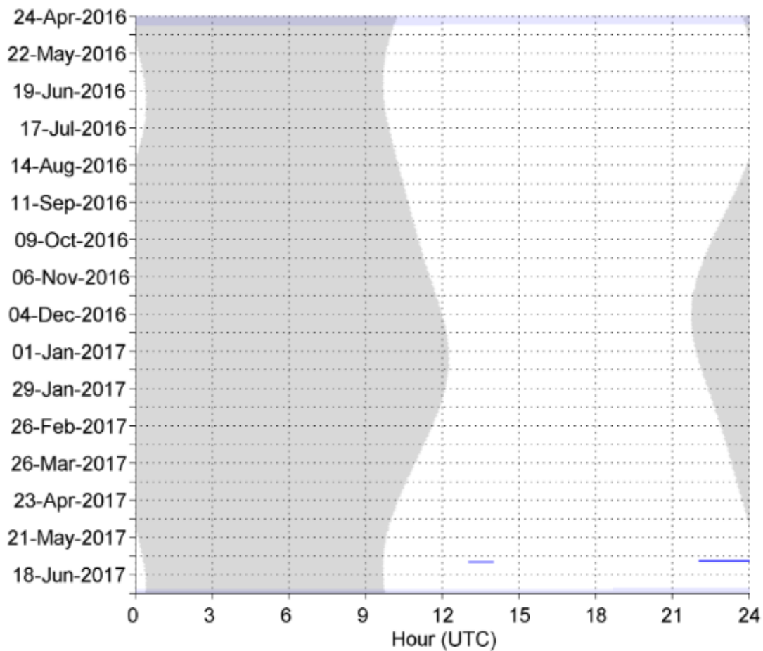
Figure 48. Weekly presence of Northern Atlantic right whale up calls between April 2016 and June 2017 at NFC Site A. Effort markings are described in Figure 39.
