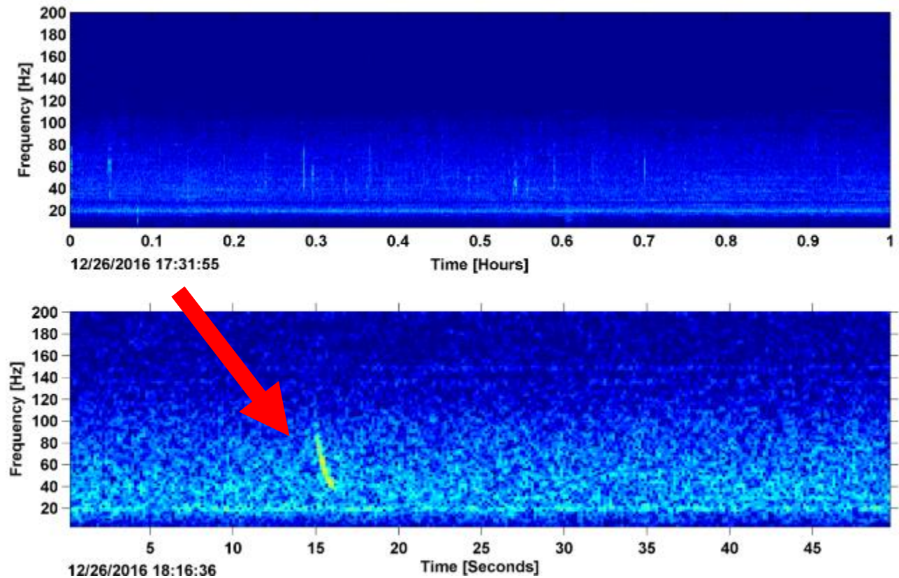
Figure 9. Downsweep calls from sei whales in the LTSA (top) and spectrogram (bottom) from NFC Site A, November 2016.
