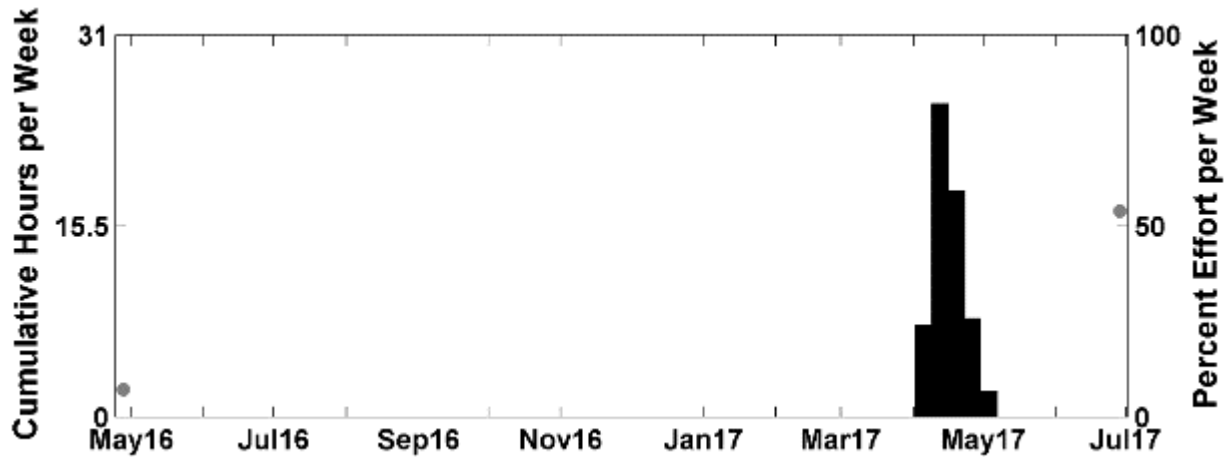
Figure 39. Weekly presence of Humpback whale calls between April 2016 and June 2017 at NFC Site A. Grey dots represent percent of effort per week in weeks with less than 100% recording effort. Where grey dots are absent, full recording effort occurred for the entire week. X-axis labels refer to month and year of recording.
