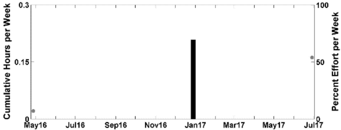
Figure 50. Weekly presence of Blainville's beaked whale echolocation clicks between April 2016 and June 2017 at NFC Site A. Effort markings are described in Figure 39.
