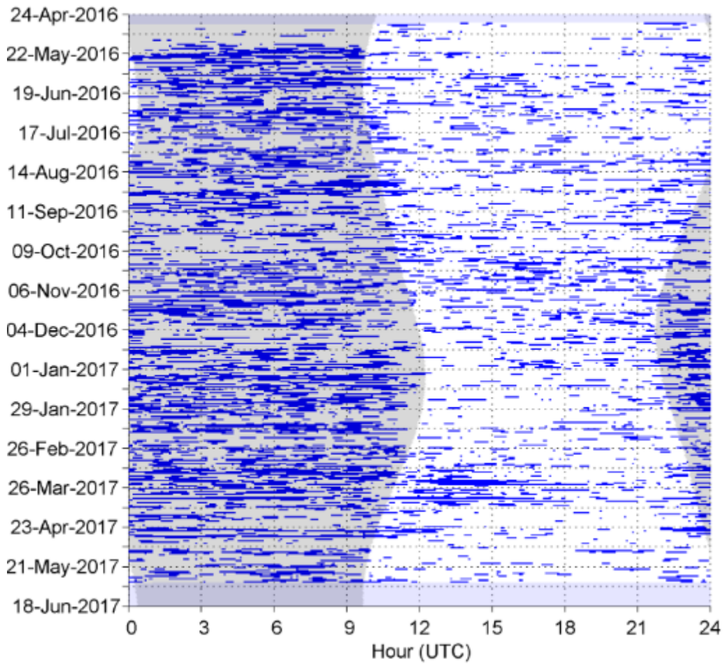
Figure 65. CT 4 in five-minute bins between April 2015 and June 2017 at NFC Site A. Gray vertical shading denotes nighttime.
