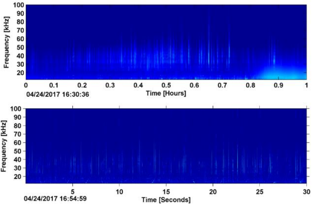
Figure 17). Studies show that spectral properties of Risso's dolphin echolocation clicks vary based on geographic region (Soldevilla et al., 2017), although the multiple sharp frequency peaks and average inter-click interval (ICI) found at these North-Western Atlantic sites are similar to what has been found elsewhere. Risso's dolphin clicks detected in this recording period had peaks at 23, 26, and 33 kHz ( Figure 18 ). Modal inter-click interval (ICI) was 165 ms.
