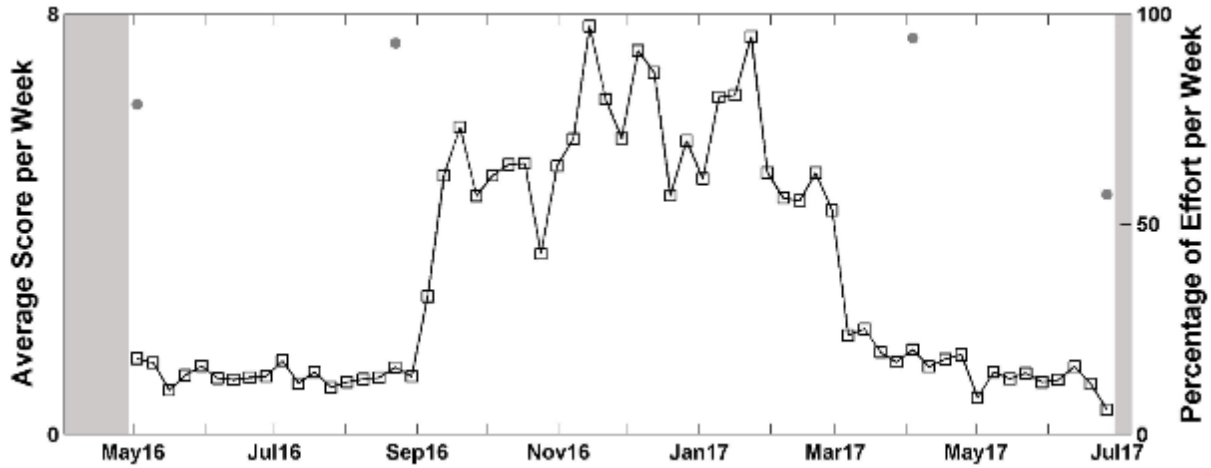
Figure 41. Weekly value of fin whale acoustic index (proxy for 20 Hz calls) detected between April 2016 and June 2017 at NFC Site A. Effort markings are described in Figure 39.
