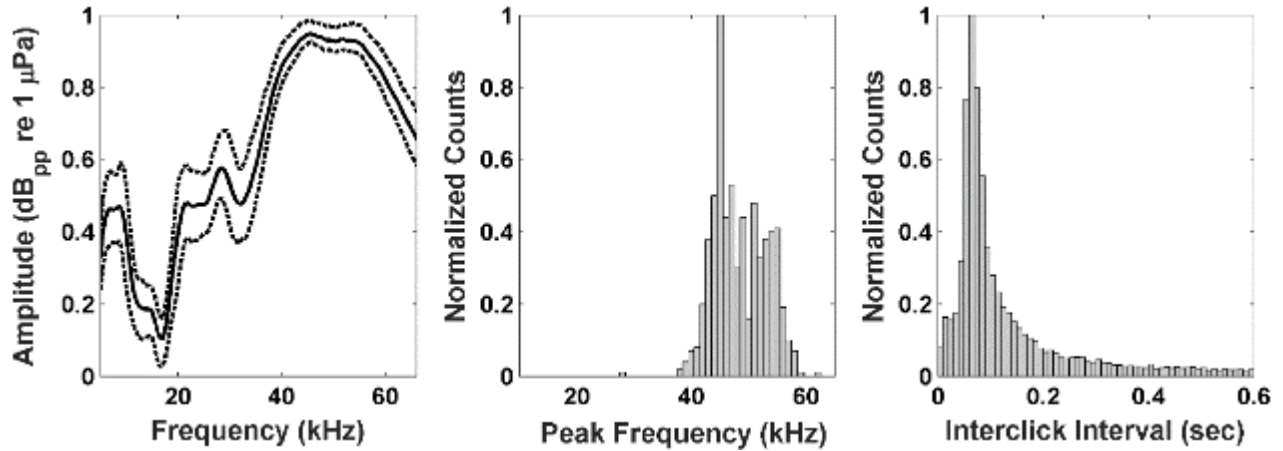
Figure 21. Click type CT 4 detected at NFC Site A from April 2016 to June 2017. Left: Mean frequency spectrum of click cluster (solid line) and 25th and 75th percentiles (dashed lines); Center: Distribution of click cluster peak frequencies; Right: Distribution of inter-click intervals (ICI) within cluster.
