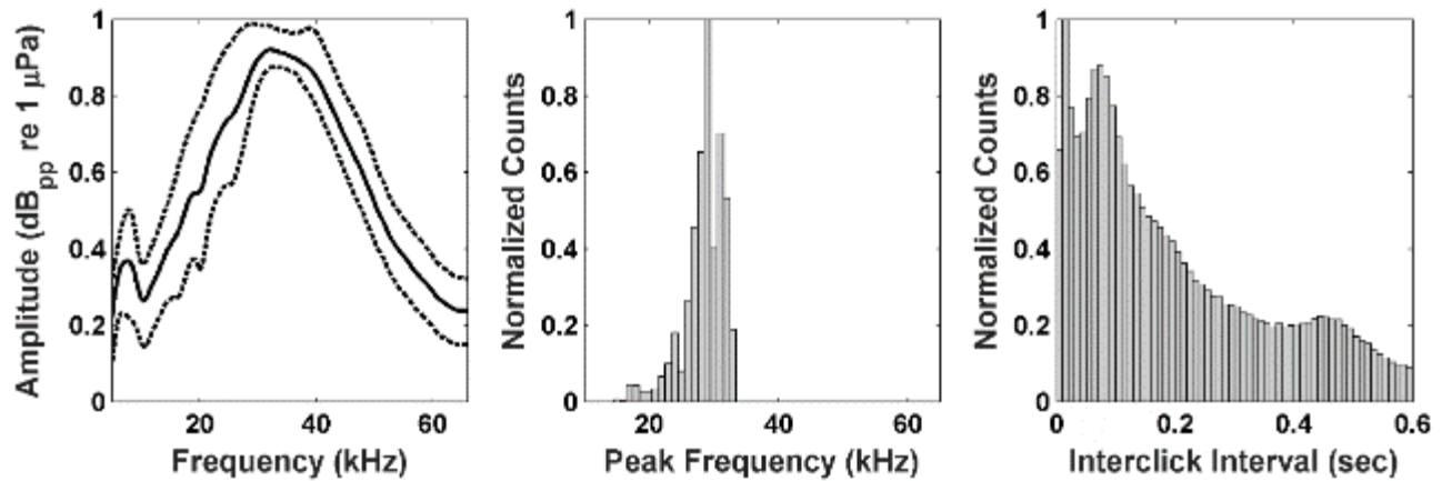
Figure 19. Click type CT 1 detected at NFC Site A from April 2016 to June 2017. Left: Mean frequency spectrum of click cluster (solid line) and 25th and 75th percentiles (dashed lines); Center: Distribution of click cluster peak frequencies; Right: Distribution of inter-click intervals (ICI) within cluster.
