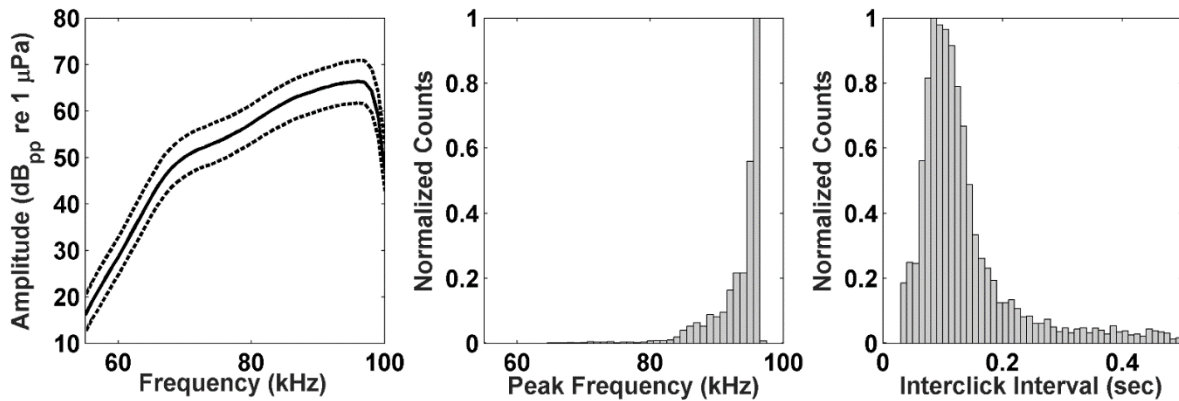
Figure 28. Kogia spp. detected at NFC Site A from April 2016 to June 2017. Left: Mean frequency spectrum of click cluster (solid line) and 25th and 75th percentiles (dashed lines); Center: Distribution of click cluster peak frequencies; Right: Distribution of inter-click intervals (ICI) within cluster.
