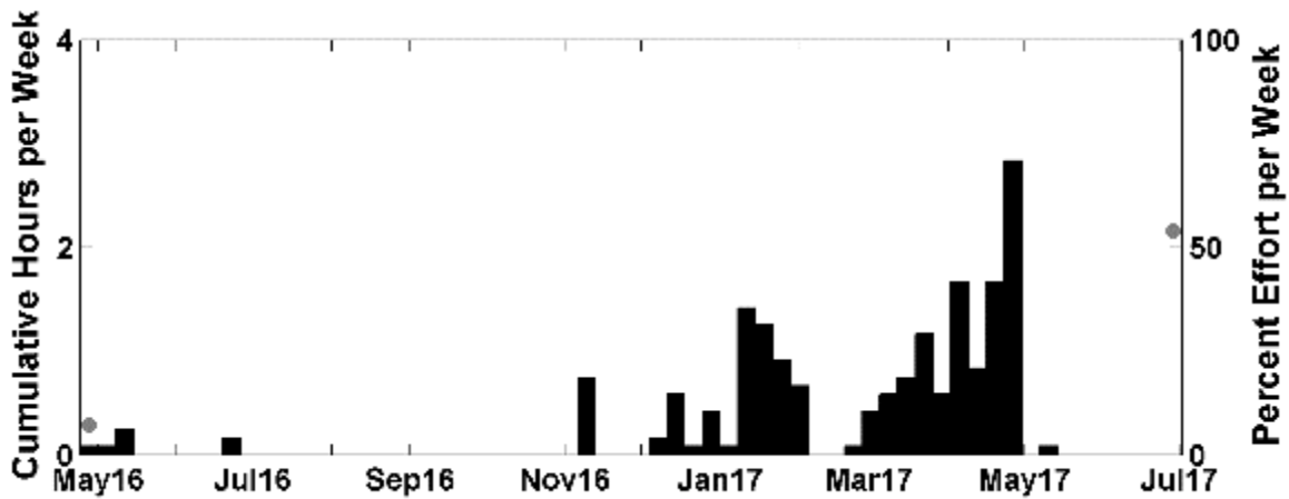
Figure 46. Weekly presence of Sei whale downsweep calls between April 2016 and June 2017 at NFC Site A. Effort markings described in Figure 39.
