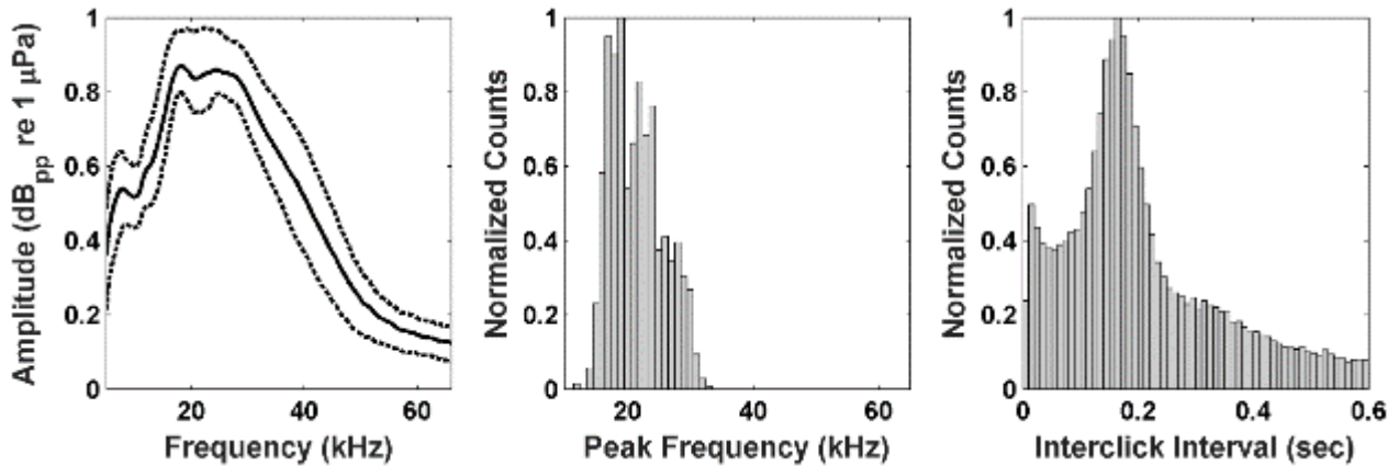
Figure 23. Click type CT 6 detected at NFC Site A from April 2016 to June 2017. Left: Mean frequency spectrum of click cluster (solid line) and 25th and 75th percentiles (dashed lines); Center: Distribution of click cluster peak frequencies; Right: Distribution of inter-click intervals (ICI) within cluster.
