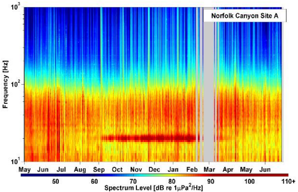
Figure 38. Long-term spectrograms using daily-averaged spectra for NFC Site A from May 2016 to June 2017.
