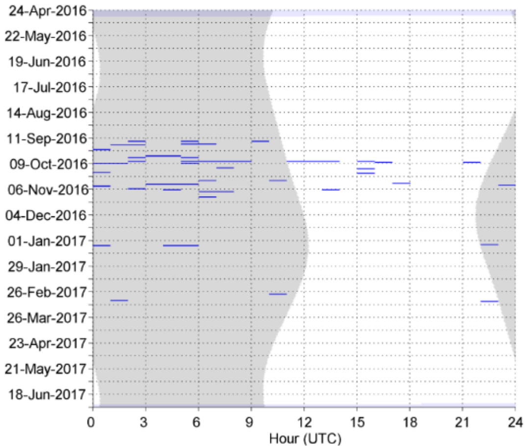
Figure 45. Minke whale pulse trains in hourly bins at NFC Site A. Gray vertical shading denotes nighttime.
