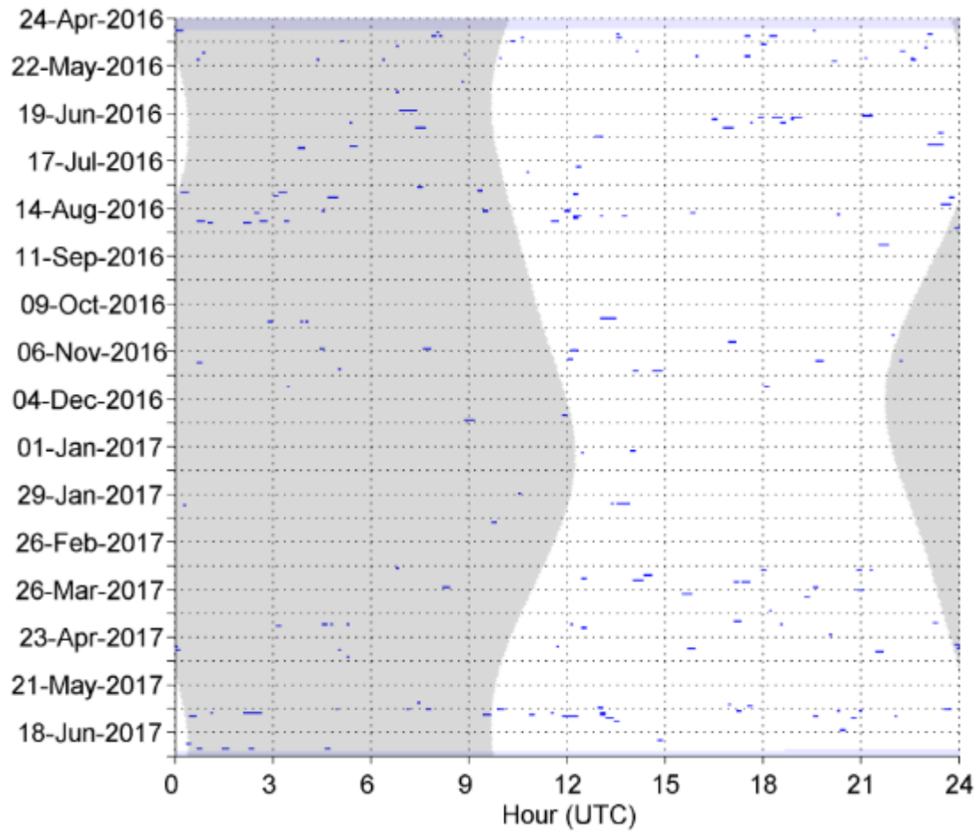
Figure 57. Sowerby's beaked whale echolocation clicks in one-minute bins between April 2016 and June 2017 at NFC Site A. Gray vertical shading denotes nighttime.
