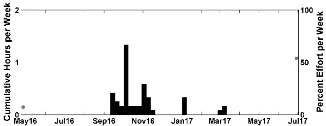
Figure 44. Weekly presence of minke whale pulse trains between April 2016 and June 2017 at NFC Site A. Effort markings are described in Figure 39.
