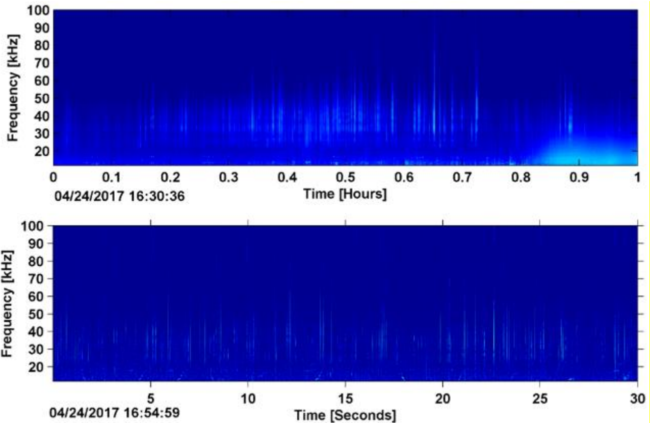
Figure 17. Risso's dolphin acoustic encounter in LTSA (top) and spectrogram (bottom) from HARP recording at NFC Site A, April 2017.
