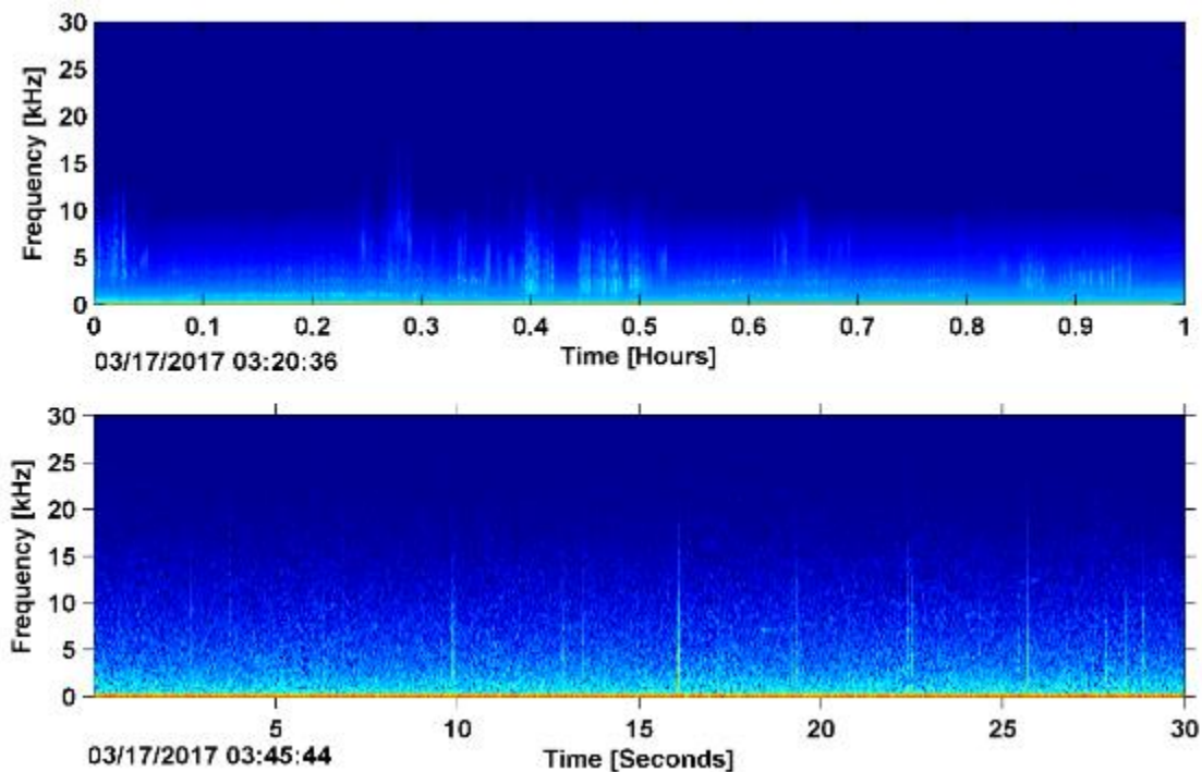
Figure 25. Sperm whale echolocation clicks in LTSA (top) and spectrogram (bottom) recorded at NFC Site A in March 2017.
