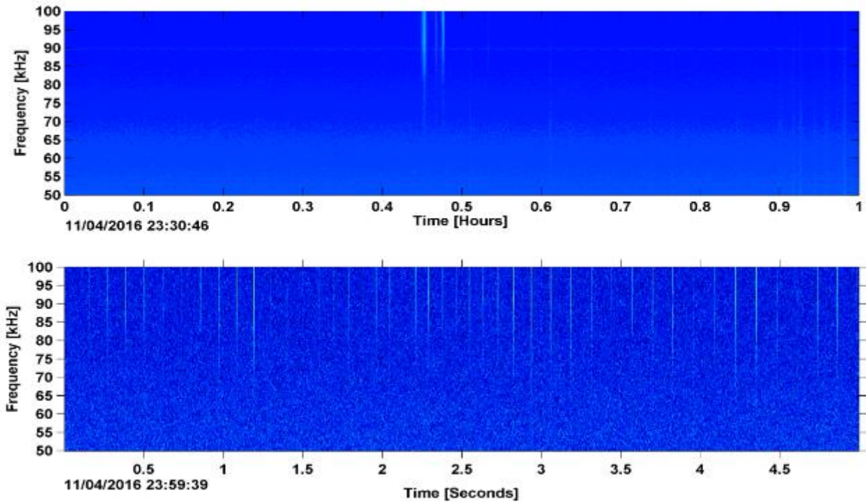
Figure 27. Kogia spp. echolocation clicks in LTSA (top) and spectrogram (bottom) recorded at NFC Site A, November 2016.
