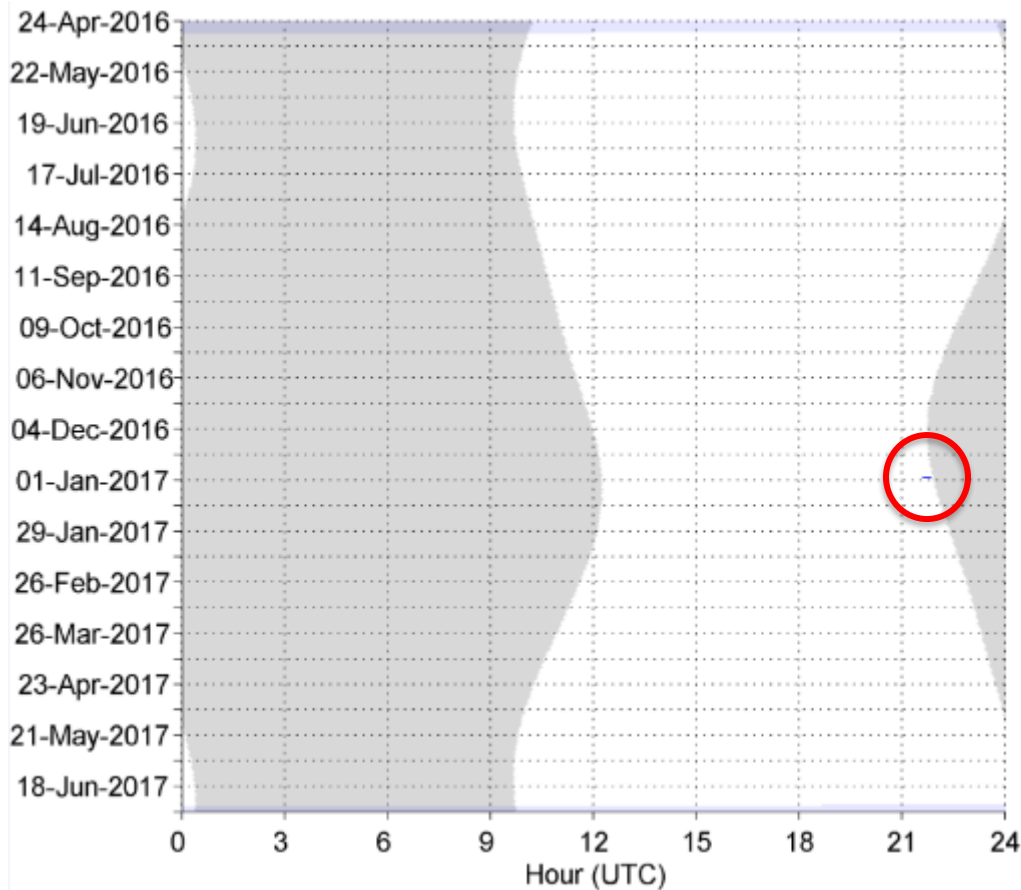
Figure 51. Blainville's beaked whale echolocation clicks in one-minute bins between April 2016 and June 2017 at NFC Site A. Gray vertical shading denotes nighttime.
