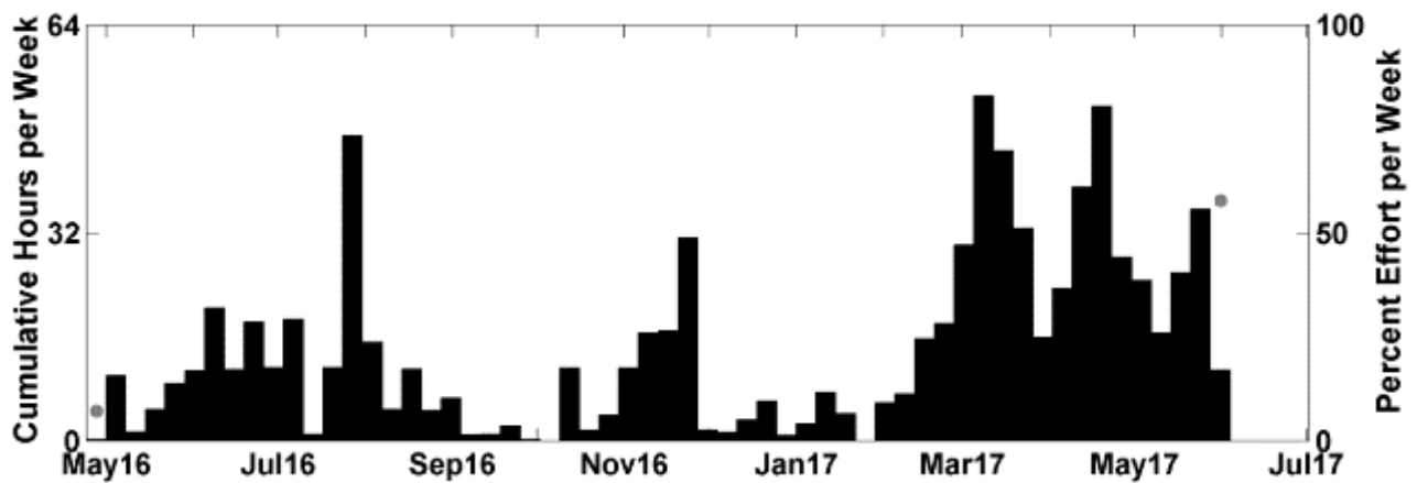
Figure 72. Weekly presence of sperm whale clicks between April 2016 and June 2017 at NFC Site A. Effort markings are described in Figure 39.
