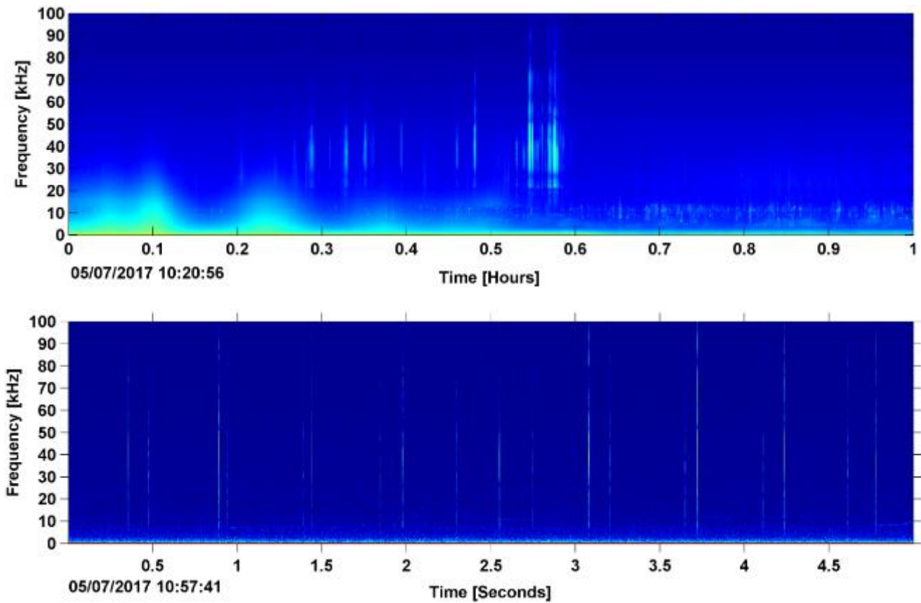
Figure 14. Cuvier's beaked whale signals in LTSA (top) and spectrogram (bottom) from HARP recording at NFC Site A, May 2017.
