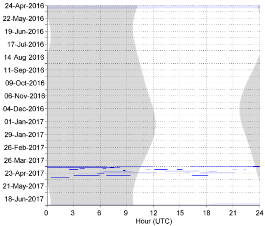
Figure 40. Humpback whale calls in hourly bins at NFC Site A. Gray vertical shading denotes nighttime.
