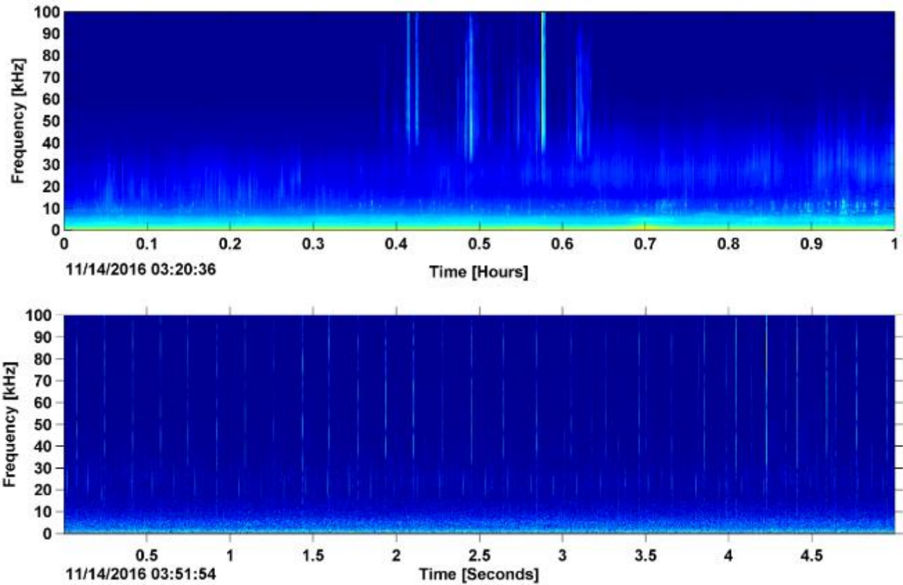
Figure 15. Gervais' beaked whale signals in LTSA (top) and spectrogram (bottom) from HARP recording at NFC Site A, November 2016.
