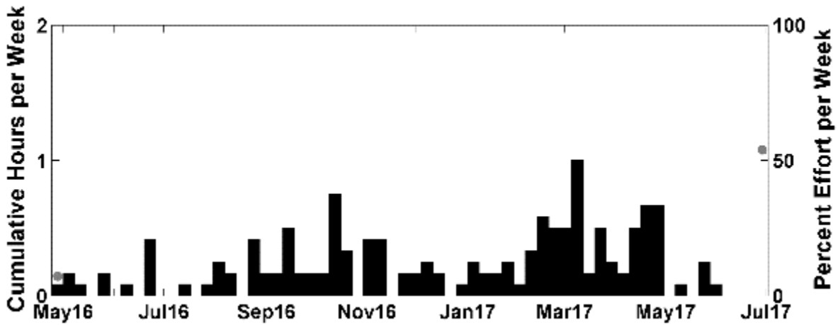
Figure 42. Fin whale 40 Hz calls detected between April 2016 and June 2017 at NFC Site A. Effort markings are described in Figure 39.
