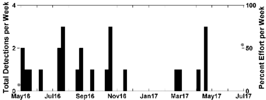
Figure 89. Weekly presence of explosions detected between April 2016 and June 2017 at NFC Site A. Effort markings are described in Figure 39.
