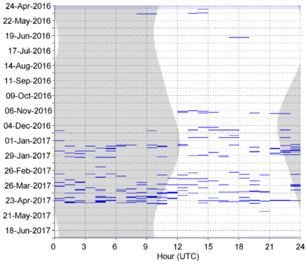
Figure 47. Sei whale downsweep calls in hourly bins at NFC Site A. Gray vertical shading denotes nighttime.
