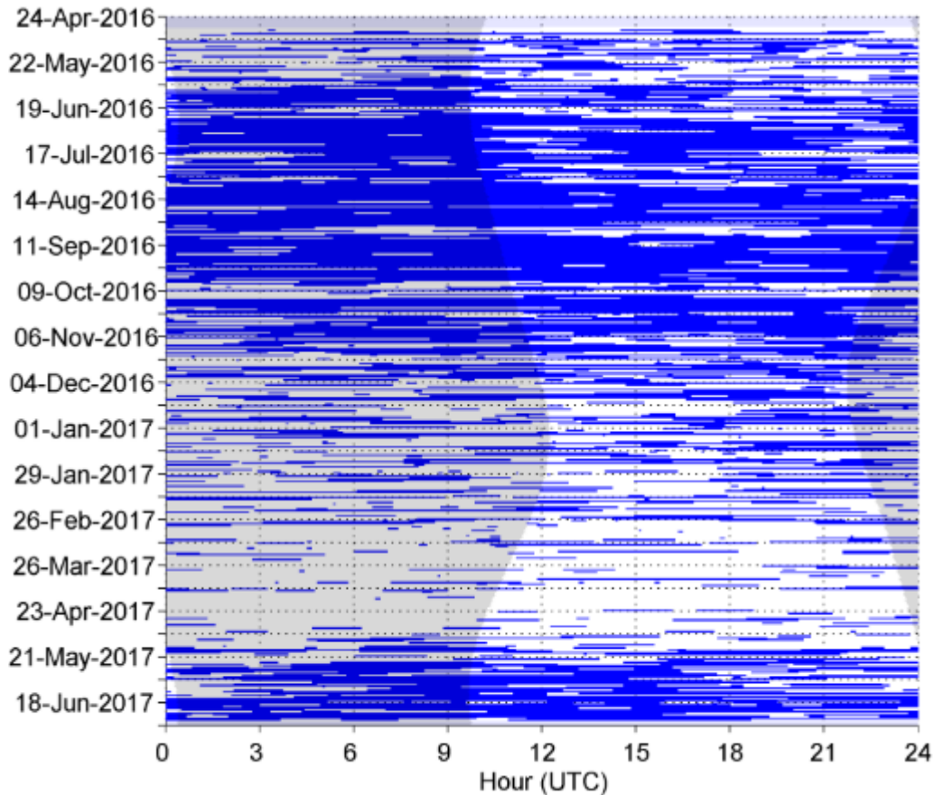
Figure 69. Unidentified odontocete whistles less than 5 kHz in five-minute bins between April 2016 and June 2017 at NFC Site A. Gray vertical shading denotes nighttime.
