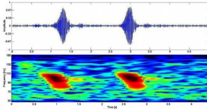
Figure 5. Waveform (top) and spectrogram (bottom) of Bryde's whale Be9 call from the Gulf of Mexico (Širović et al., 2014).
