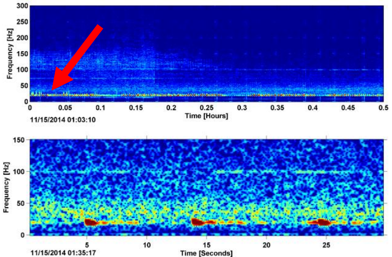
Figure 6. Fin whale 20 Hz call in LTSA (top) and spectrogram (bottom) at NFC Site A, November 2014.
