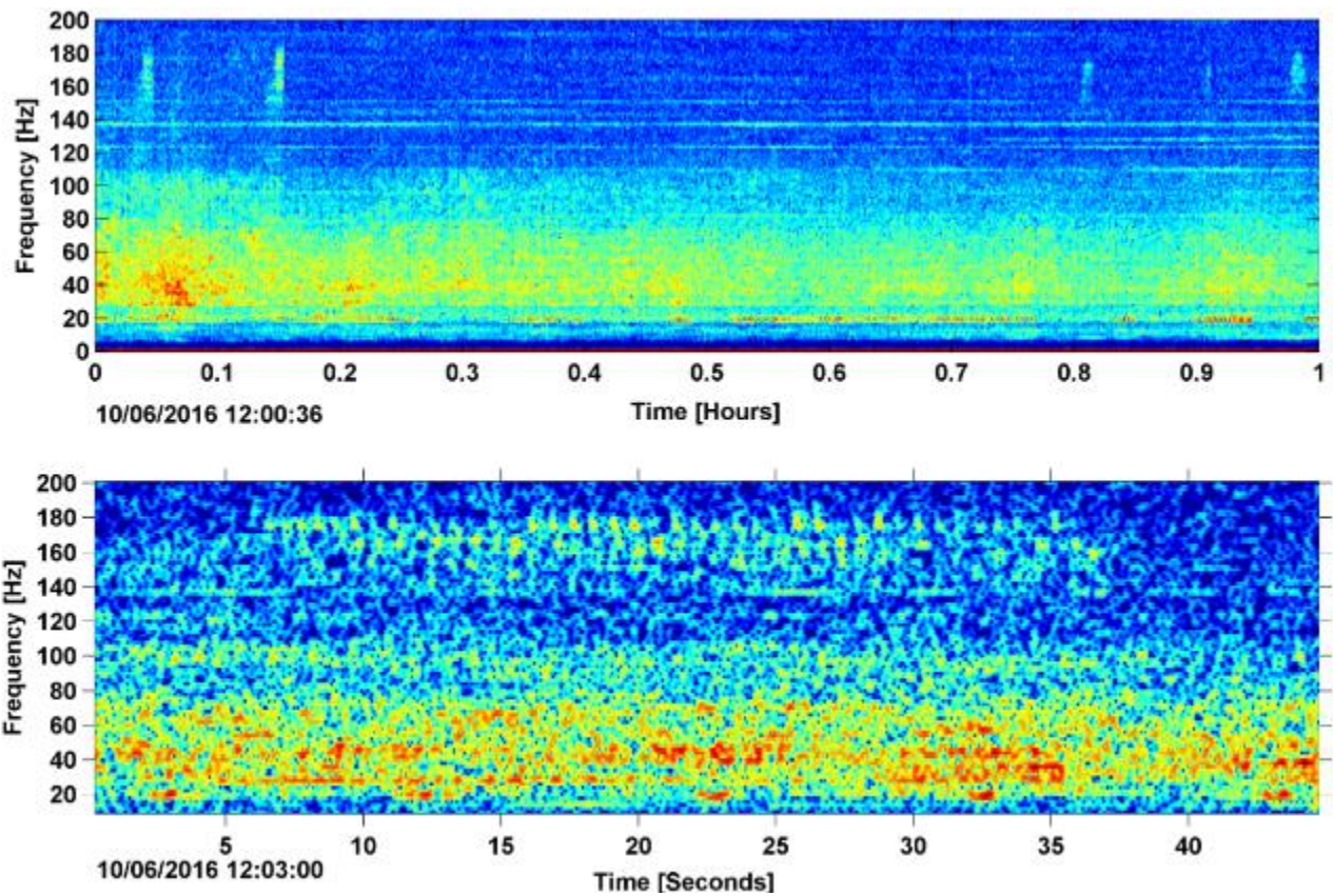
Figure 8. Minke whale pulse train in the LTSA (top) and spectrogram (bottom) recorded at NFC Site A, October 2016.
