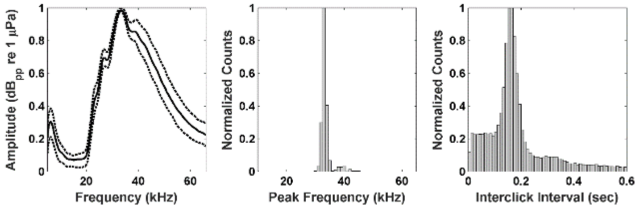
Figure 18. Risso's dolphin click type detected at NFC Site A from April 2016 to June 2017. Left: Mean frequency spectrum of click cluster (solid line) and 25th and 75th percentiles (dashed lines); Center: Distribution of click cluster peak frequencies; Right: Distribution of inter-click intervals (ICI) within cluster.
