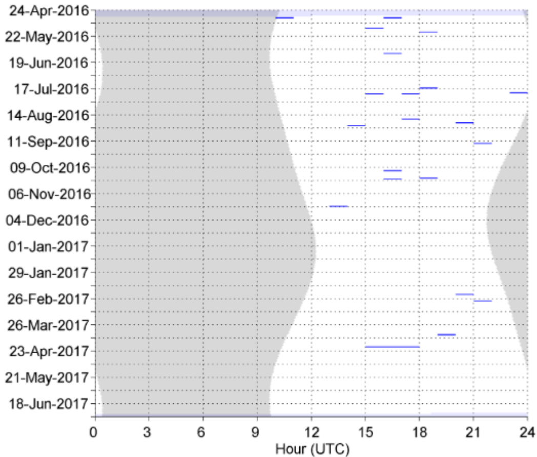
Figure 90. Explosions in one-minute bins between April 2016 and June 2017 at NFC Site A. Gray vertical shading denotes nighttime.
