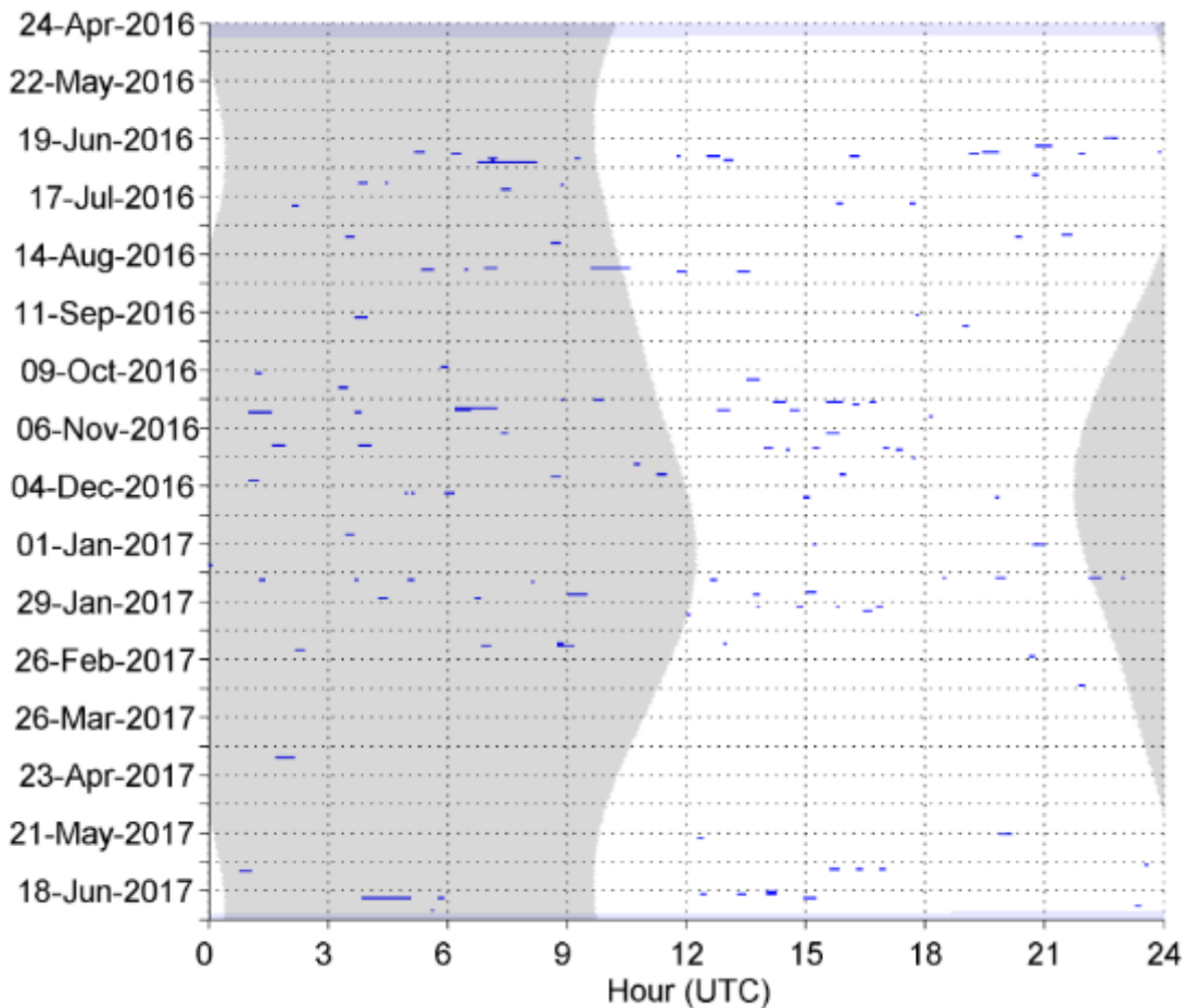
Figure 55. Gervais' beaked whale echolocation clicks in one-minute bins between April 2016 and June 2017 at NFC Site A. Gray vertical shading denotes nighttime.
