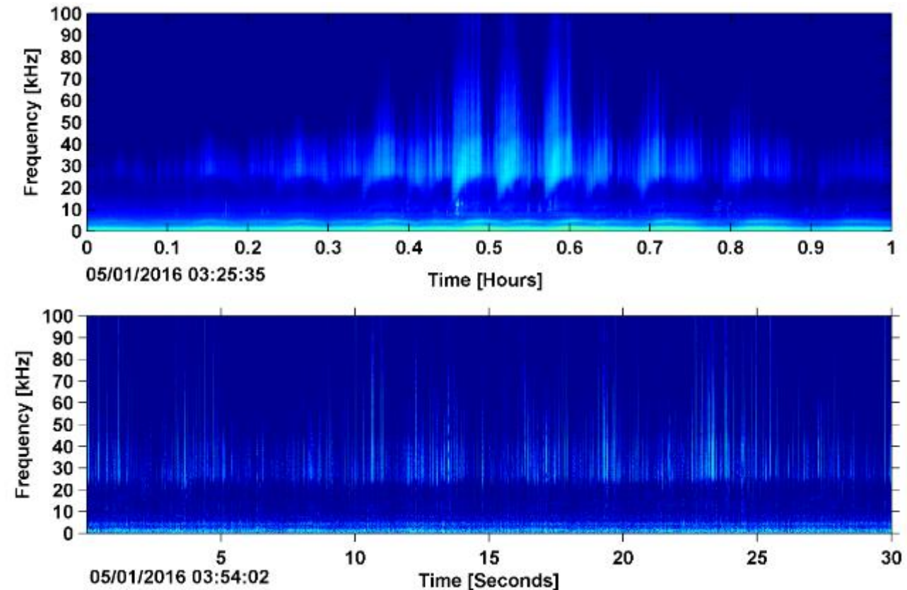
Figure 20. Click type CT 1 acoustic encounter in LTSA (top) and spectrogram (bottom) recorded at NFC Site A in May 2016.
