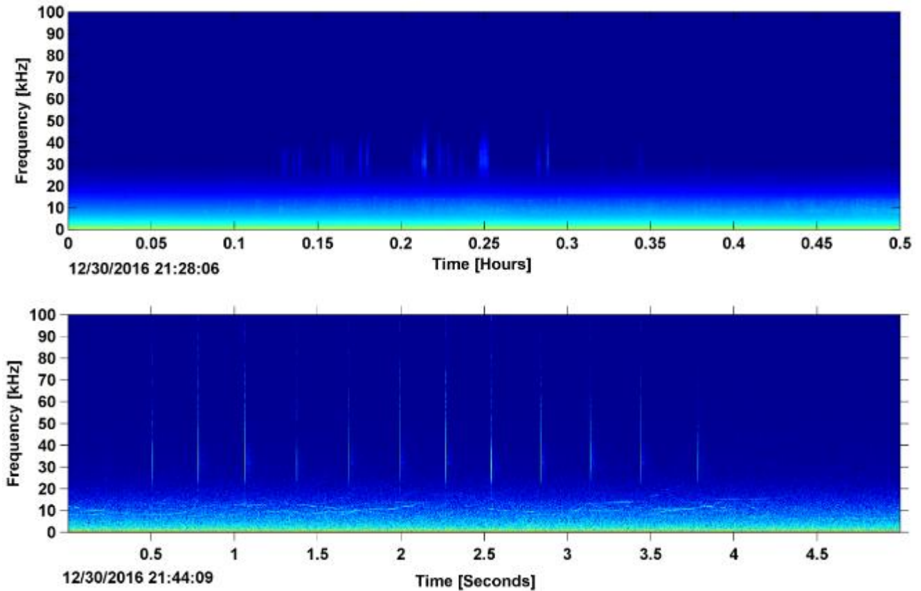
Figure 13. Blainville's beaked whale echolocation clicks in the LTSA (top) and spectrogram (bottom) from HARP recording at NFC Site A, December 2016.
