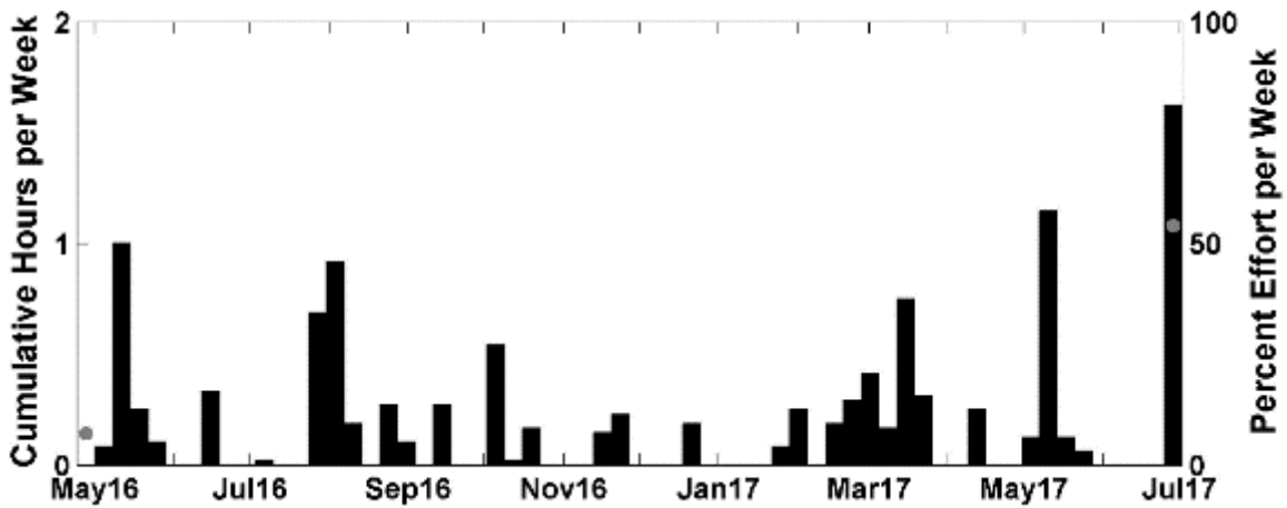
Figure 52. Weekly presence of Cuvier's beaked whale echolocation clicks between April 2016 and June 2017 at NFC Site A. Effort markings are described in Figure 39.
