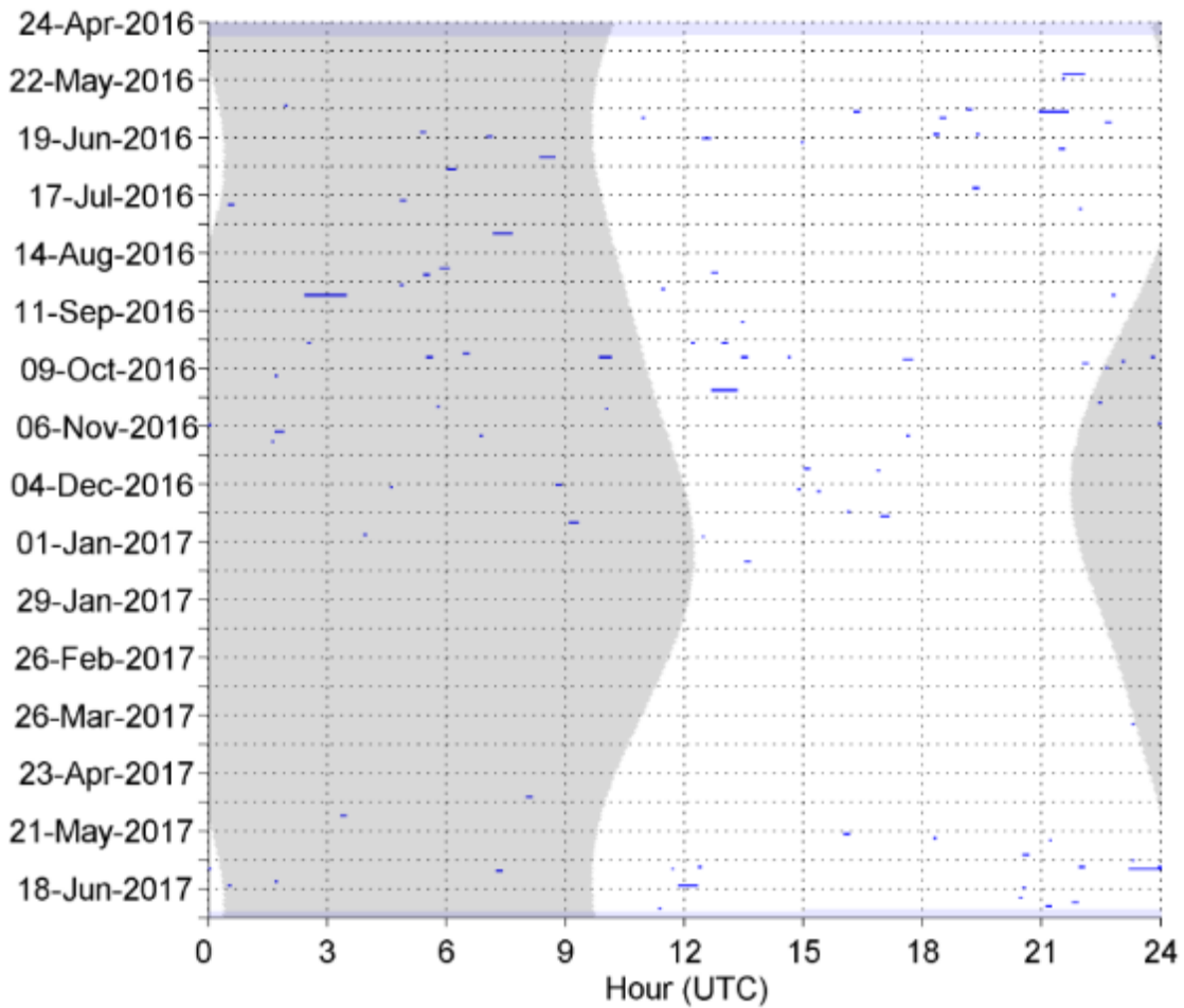
Figure 75. Kogia spp. clicks in one-minute bins between April 2016 and June 2017 at NFC Site A. Gray vertical shading denotes nighttime.
