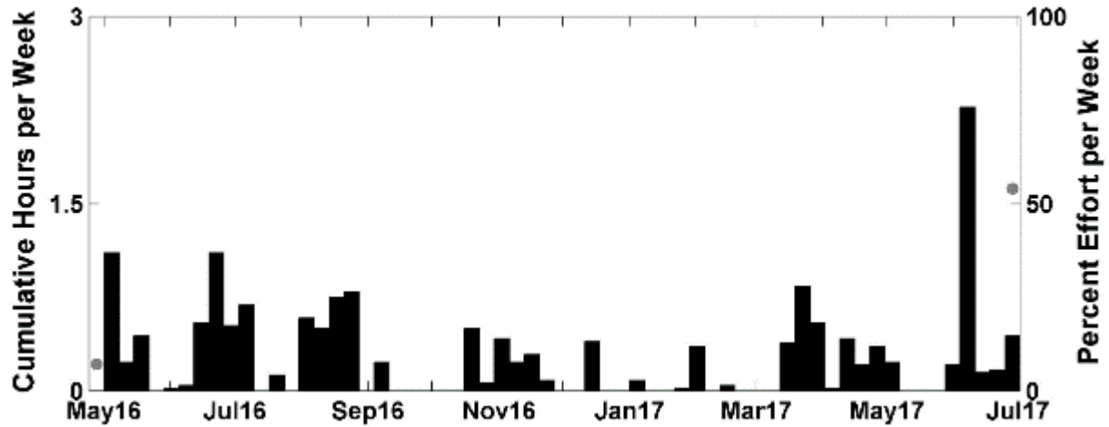
Figure 56. Weekly presence of Sowerby's beaked whale echolocation clicks between April 2016 and June 2017 at NFC Site A. Effort markings are described in Figure 39.
