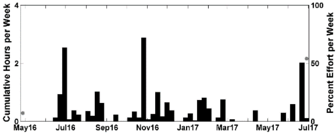
Figure 54. Weekly presence of Gervais' beaked whale echolocation clicks between April 2016 and June 2017 at NFC Site A. Effort markings are described in Figure 39.
