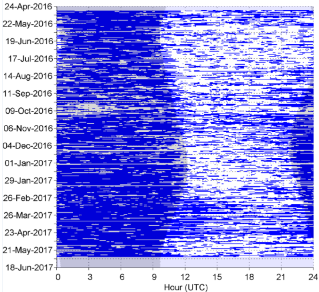
Figure 63. CT 1 in five-minute bins between April 2016 and June 2017 at NFC Site A. Gray vertical shading denotes nighttime.
