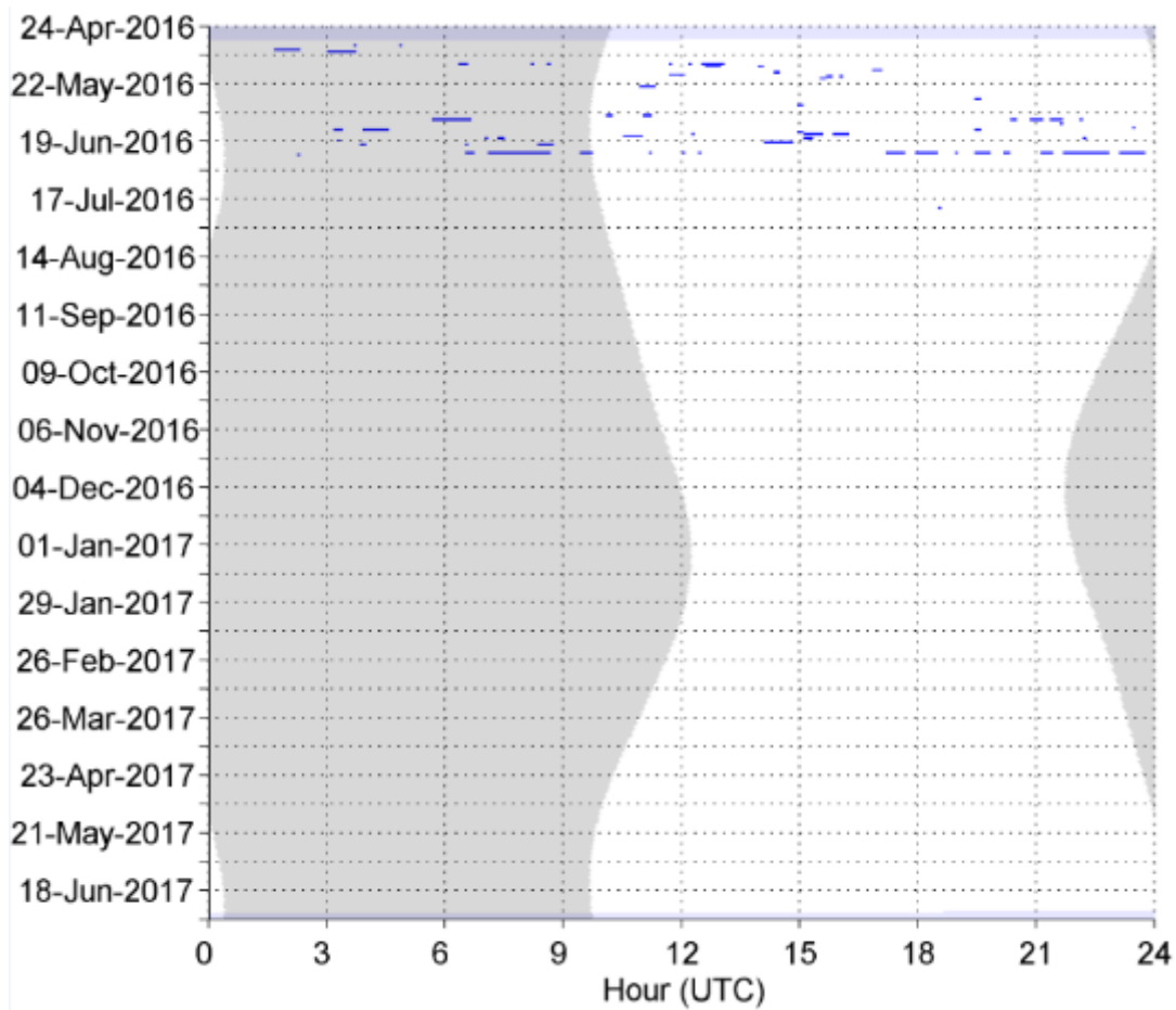
Figure 92. Airguns in one-minute bins between April 2016 and June 2017 at NFC Site A. Gray vertical shading denotes nighttime.
