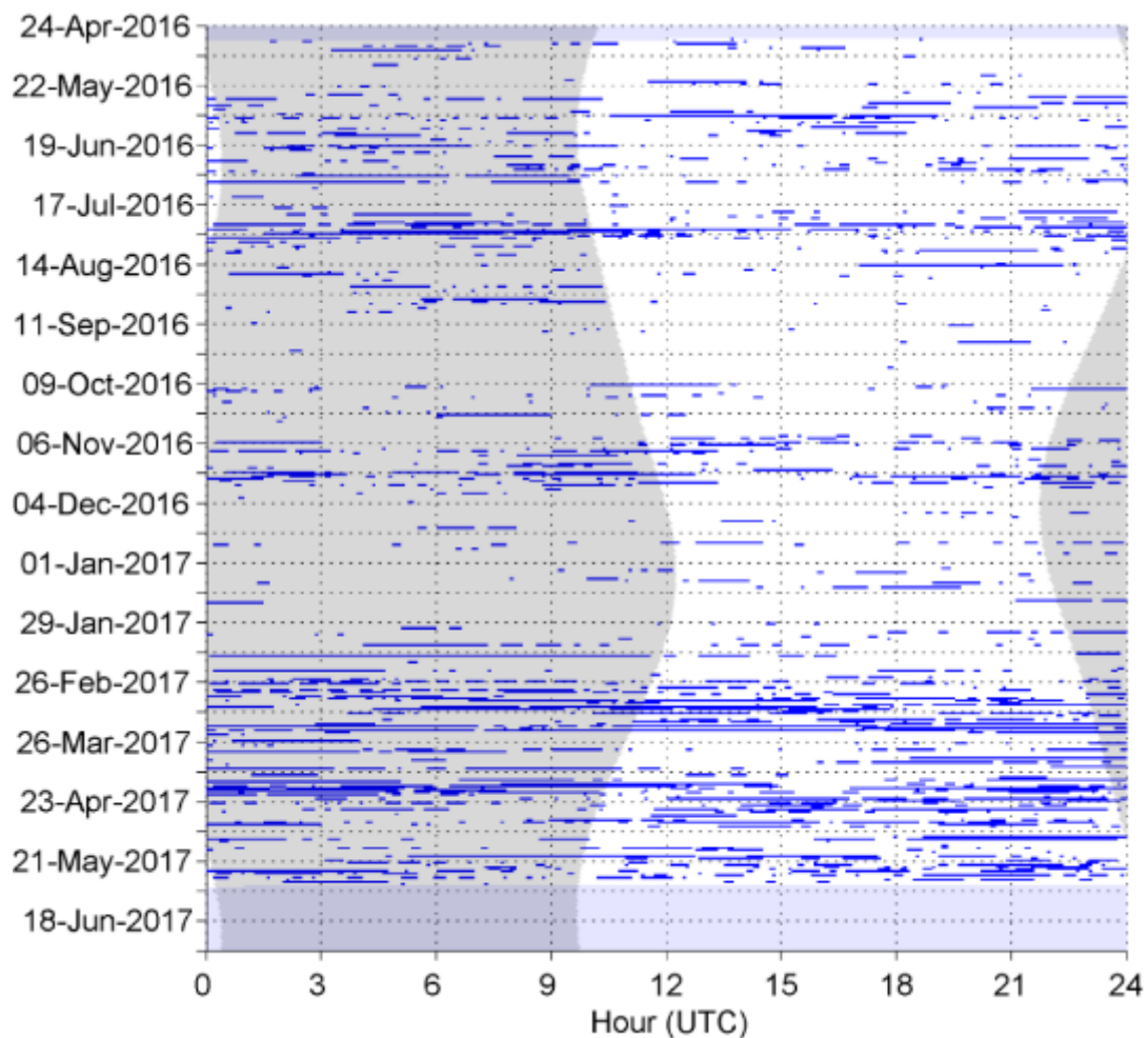
Figure 73. Sperm whale clicks in one-minute bins between April 2016 and June 2017 at NFC Site A. Gray vertical shading denotes nighttime.
