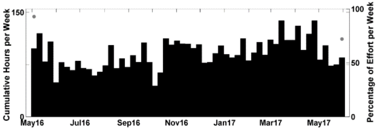
Figure 60. Weekly presence of unidentified odontocete clicks between April 2016 and June 2017 at NFC Site A. Effort markings are described in Figure 39.
