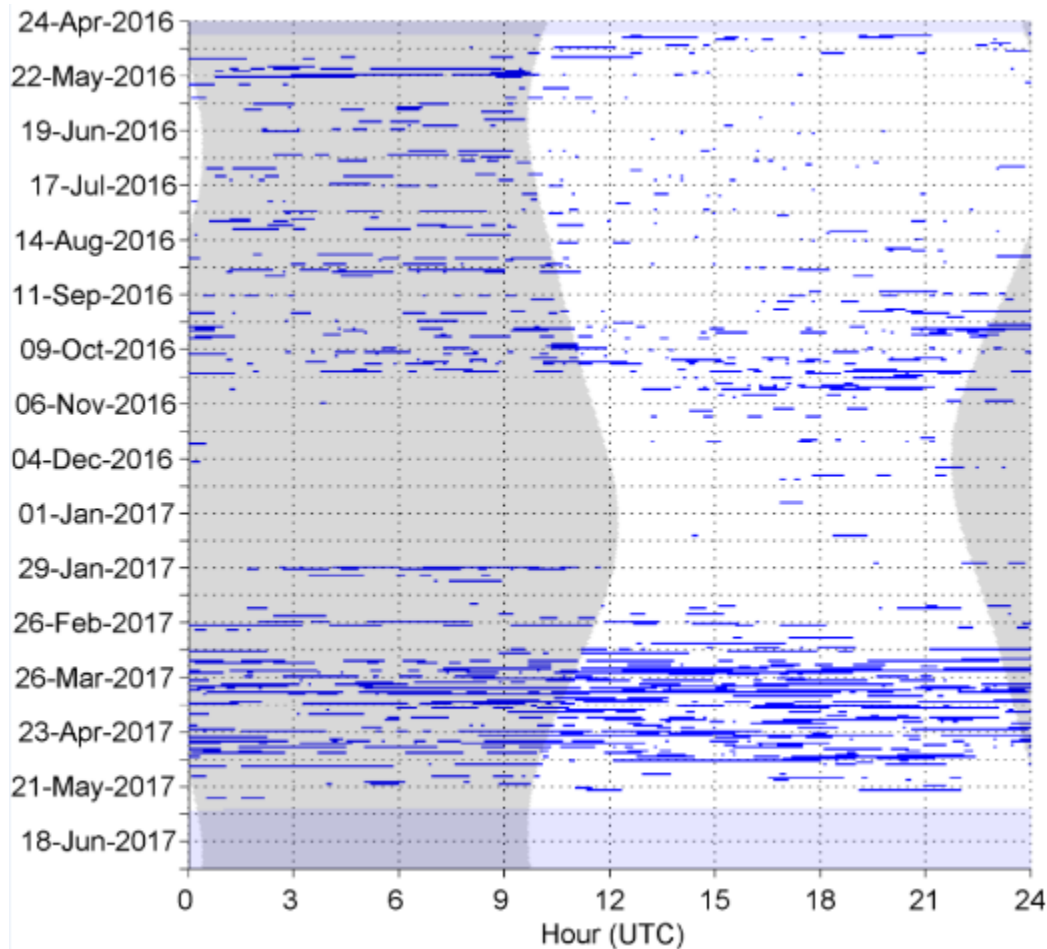
Figure 59. Risso's dolphin echolocation clicks in five-minute bins between April 2016 and June 2017 at NFC Site A. Gray vertical shading denotes nighttime.
