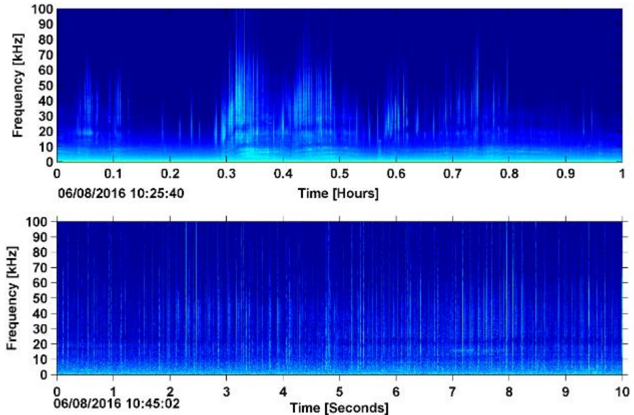
Figure 22. Click type CT 4 acoustic encounter in LTSA (top) and spectrogram (bottom) recorded at NFC Site A in June 2016.
