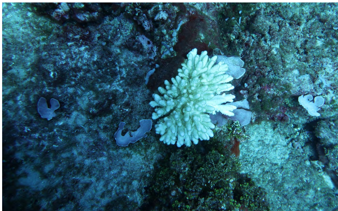
Figure 19: Acropora new species #1, originally thought to be A. humilis , a species that often looks similar to the ESA-listed A. globiceps . This specimen does not have characteristics consistent with A. globiceps , either.
