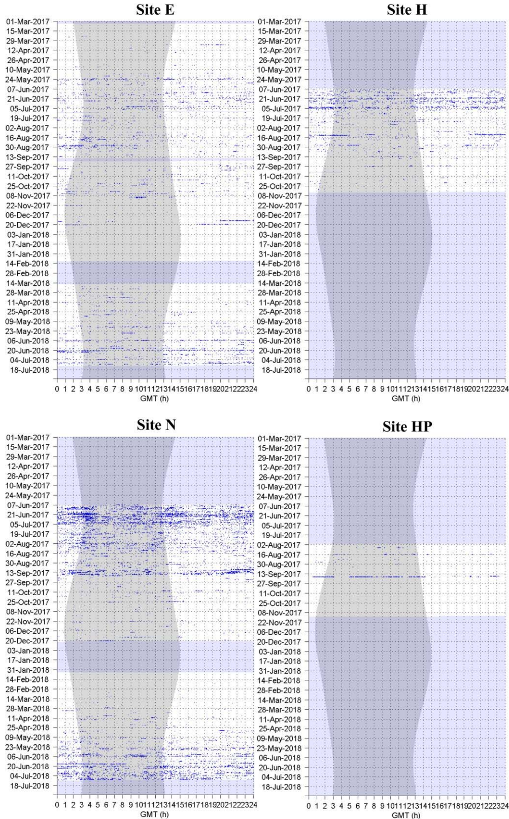
Figure 16. Diel presence of NE Pacific blue whale D calls, indicated by blue dots, in one-minute bins at sites E, H, N and HP. Gray vertical shading denotes nighttime and light purple horizontal shading denotes absence of acoustic data.
