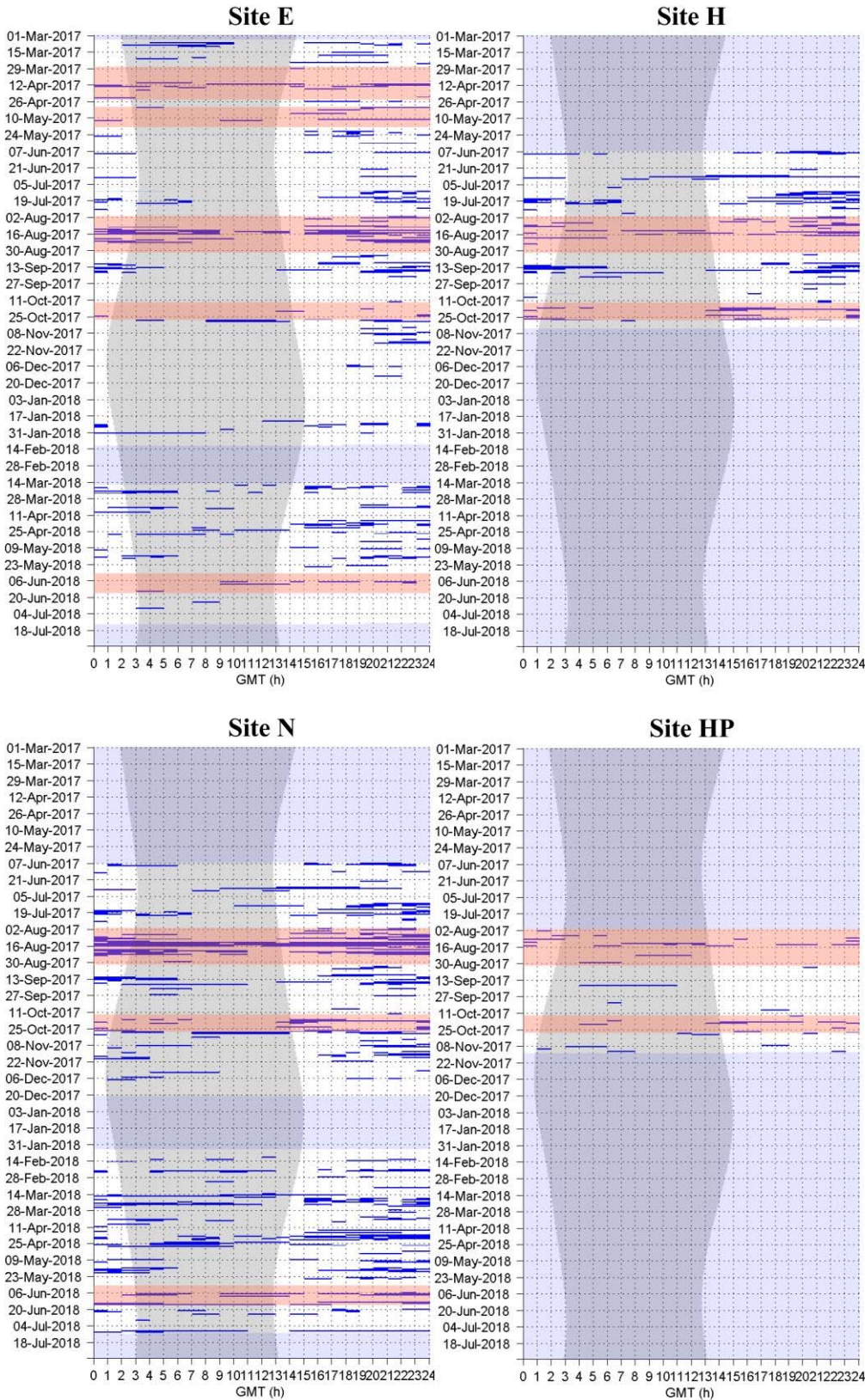
Figure 25. Major naval training events (shaded orange, from Table 3) overlaid on MFA sonar <5kHz signals, indicated by blue dots, in one-hour bins at sites E, H, N, and HP. Gray vertical shading denotes nighttime and light purple horizontal shading denotes absence of acoustic data.
