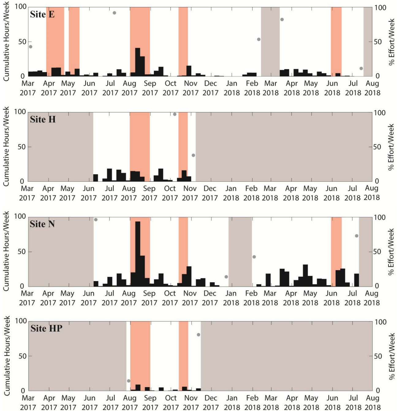
Figure 24. Major naval training events (shaded orange, from Table 3) overlaid on weekly presence of MFA sonar <5kHz between March 2017 and July 2018 at sites E, H, N, and HP.
