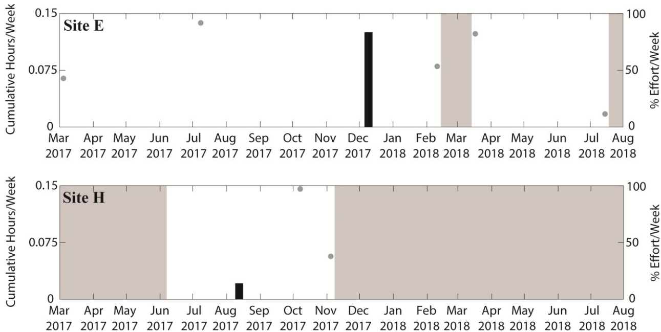
Figure 20. Weekly presence of BW35 FM pulses between March 2017 and July 2018 at sites E and H. There were no detections at site N.
