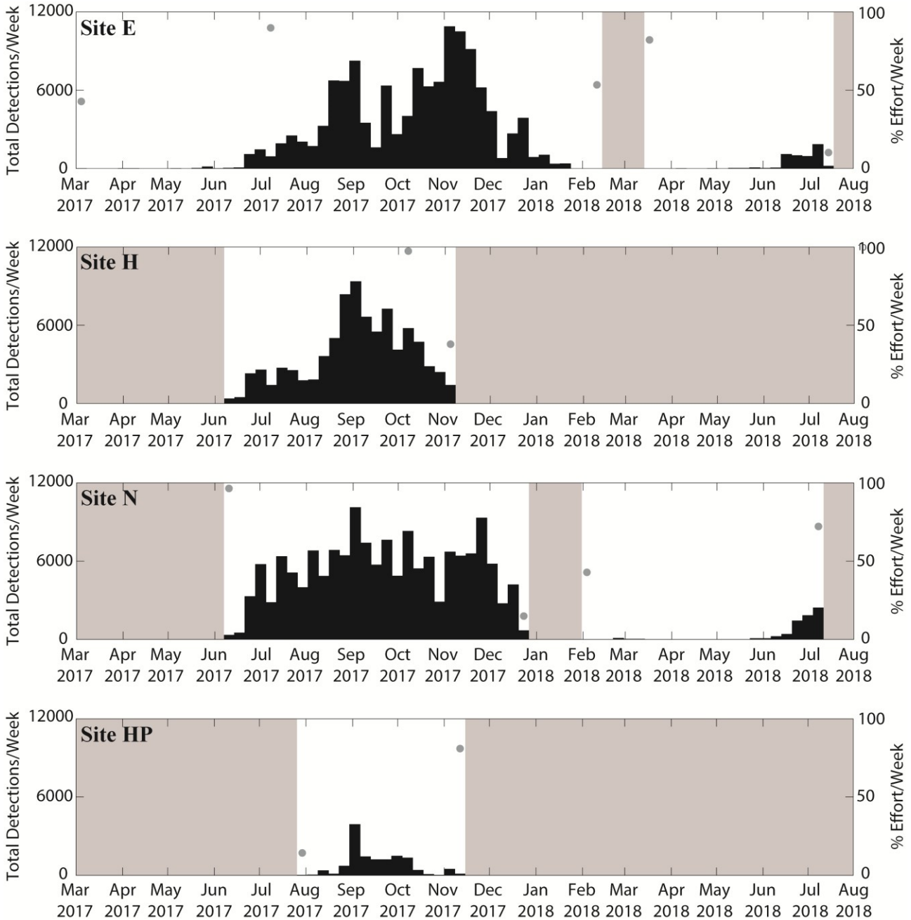
Figure 13. Weekly presence of NE Pacific blue whale B calls between March 2017 and July 2018 at sites E, H, N, and HP. Gray dots represent percent of effort per week in weeks with less than 100% recording effort, and gray shading represents percent periods with no recording effort. Where gray dots or shading are absent, full recording effort occurred for the entire week.
