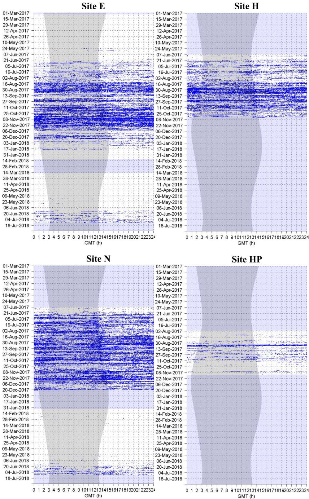
Figure 14. Diel presence of NE Pacific blue whale B calls, indicated by blue dots, in one-minute bins at sites E, H, N, and HP. Gray vertical shading denotes nighttime and light purple horizontal shading denotes absence of acoustic data.
