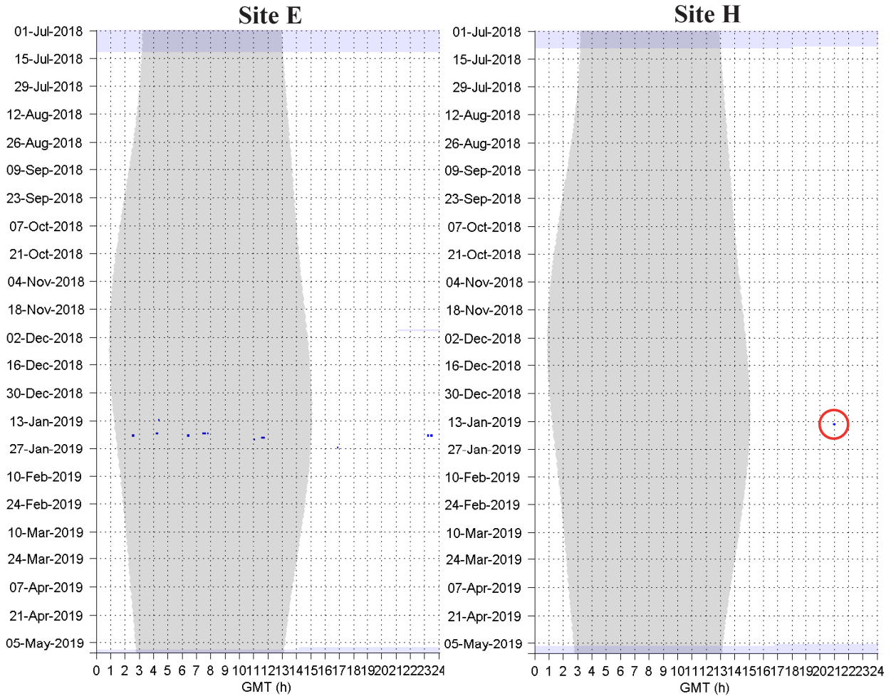
Figure 20. BW35 FM pulses, indicated by blue dots, in five-minute bins at sites E, H, and N. There were no detections at sites N. Gray vertical shading denotes nighttime and light purple horizontal shading denotes absence of acoustic data. Red circle highlights only time where detections occurred at site H.
