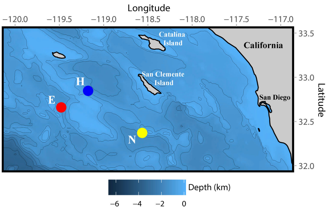
Figure 1. Locations of High-frequency Acoustic Recording Package (HARP) deployment sites E, H, and N (circles) in the SOCAL study area from July 2018 through May 2019.
