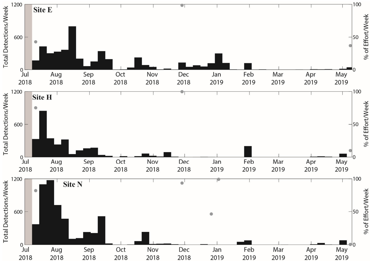
Figure 14. Weekly presence of blue whale D calls between July 2018 and May 2019 at sites E, H, and N. Gray dots represent percent of effort per week in weeks with less than 100% recording effort, and gray shading represents periods with no recording effort. Where gray dots or shading are absent, full recording effort occurred for the entire week.
