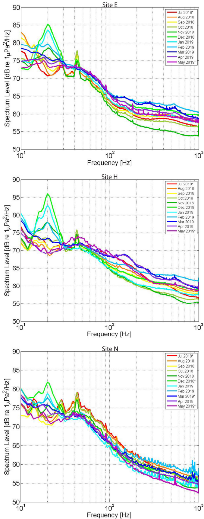
Figure 11. Monthly averages of sound spectrum levels at sites E, H, and N.
