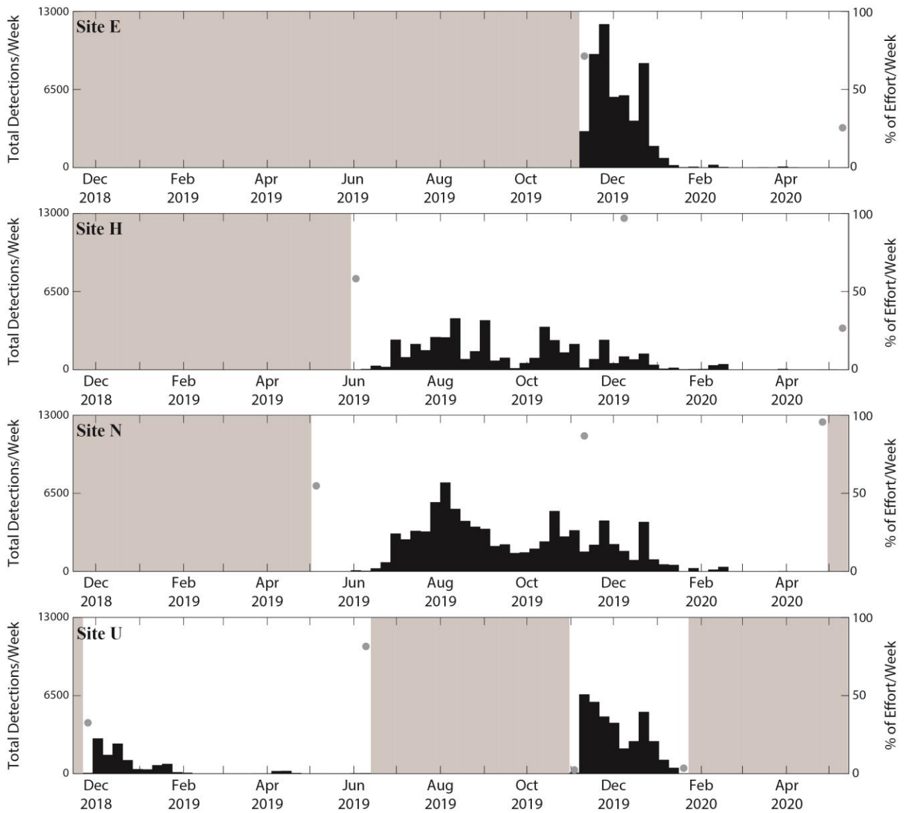
Figure 11. Weekly presence of NE Pacific blue whale B calls between November 2018 and May 2020 at sites E, H, N, and U. Gray dots represent percent of effort per week in weeks with less than 100% recording effort, and gray shading represents periods with no recording effort. Where gray dots or shading are absent, full recording effort occurred for the entire week. Analysis of data from December 2018 to May 2019 for sites E, H, and N was completed during a previous monitoring period (Rice et al. , 2020).
