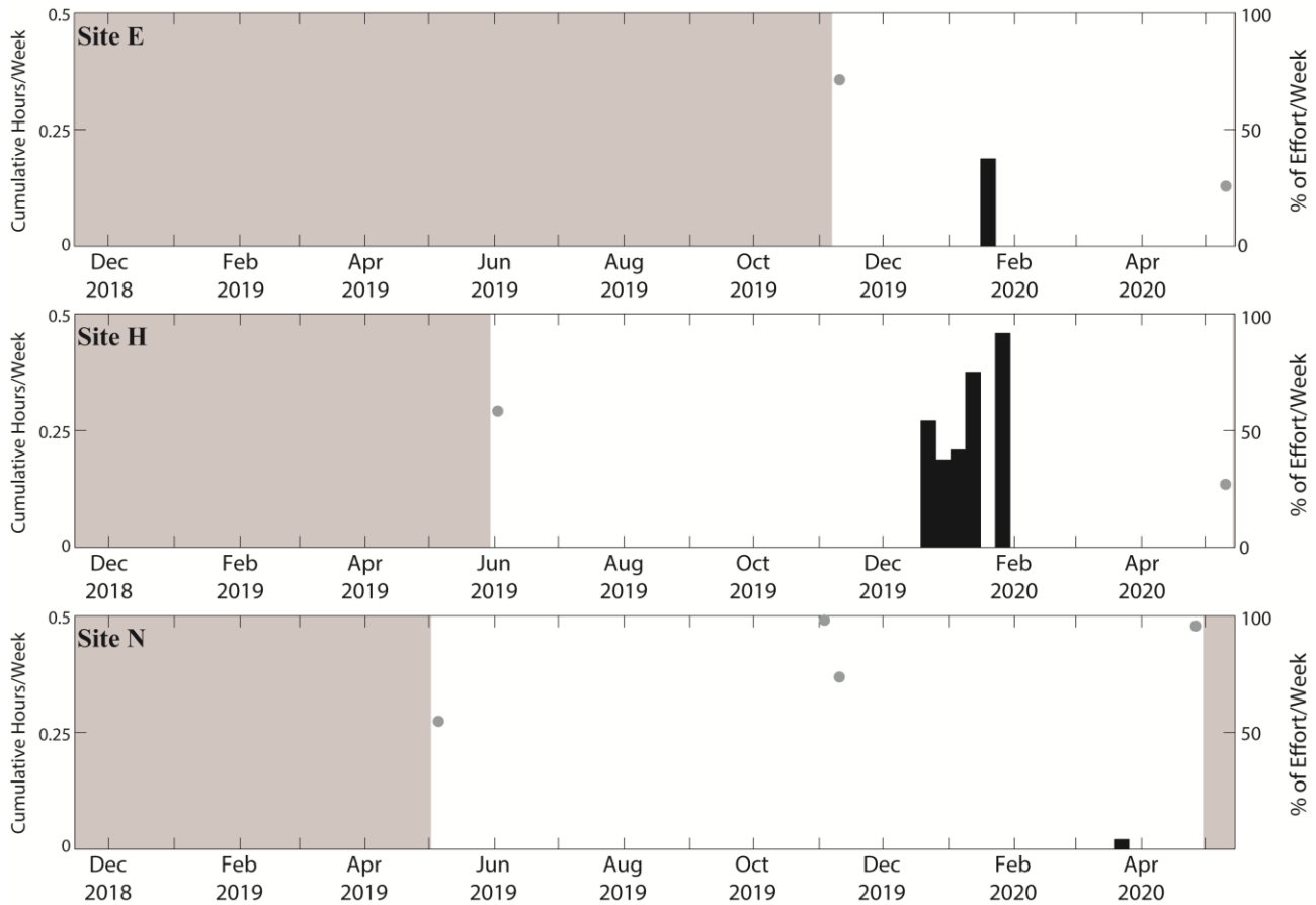
Figure 16. Weekly presence of BW37V FM pulses between November 2018 and May 2020 at sites E, H, and N.
