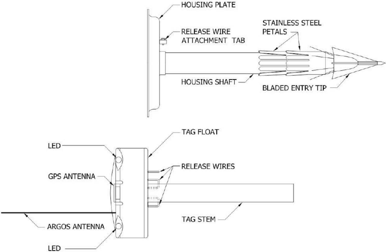
Figure 2. Schematic diagram of the recoverable Wildlife Computers MK10 Advanced Dive Behavior (ADB) tag (bottom) with the OSU-designed housing (top). The housing shaft is designed for implantation beneath the whale's skin while the plate and tag float sit atop the whale's back.
