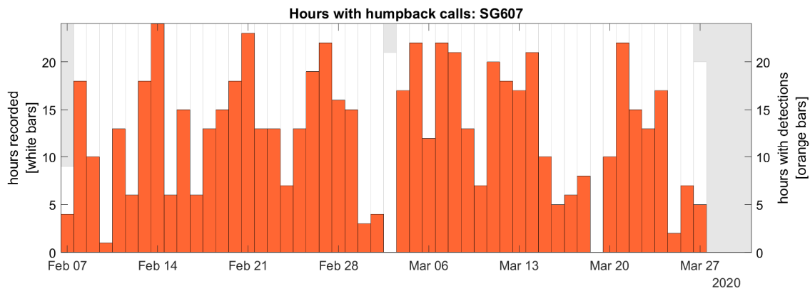
Figure 14. Number of hours per day with detections of humpback whales on the abyssal glider (SG607). Gray background indicates a period of no data.
