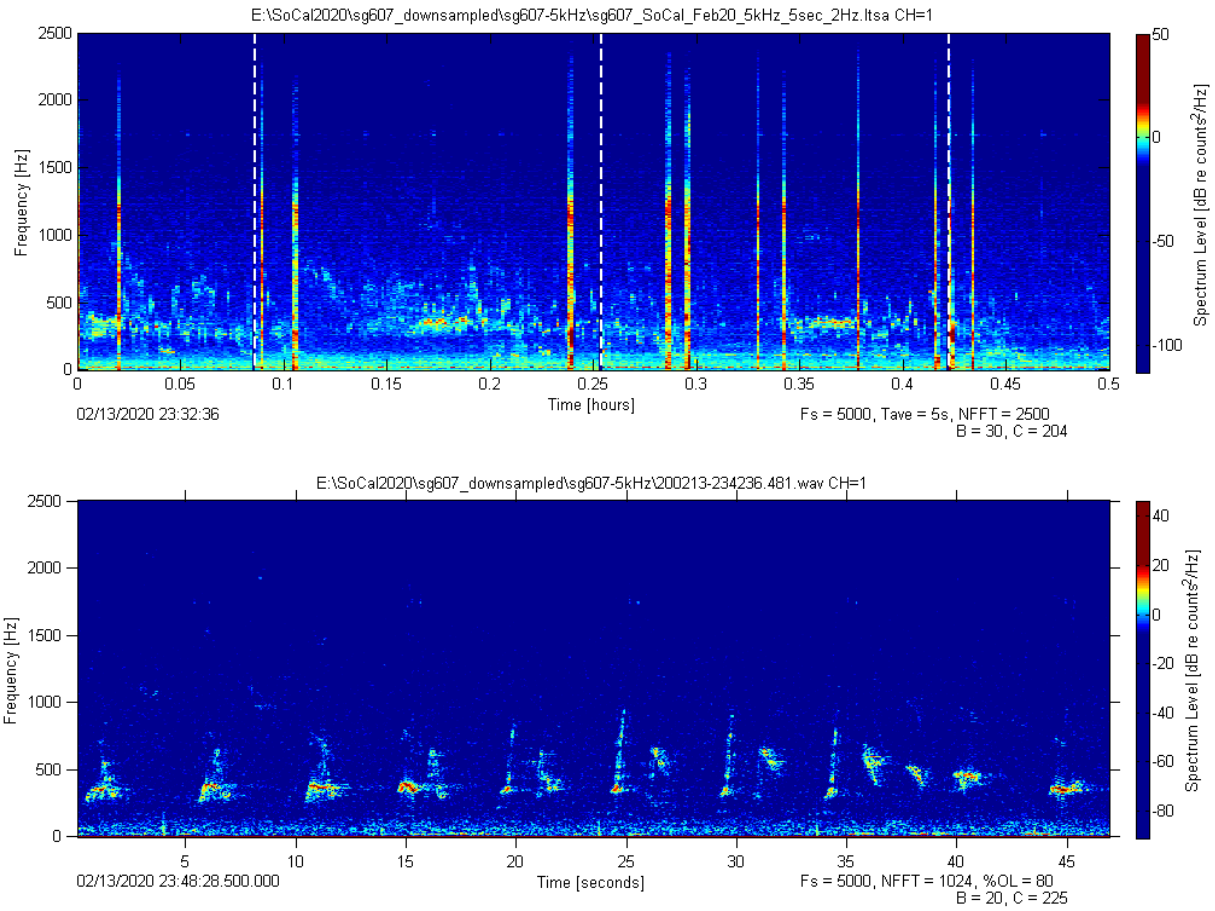
Figure F-3. Example of an LTS of humpback vocalizations graded as a “5”, on a scale of 1-5.
