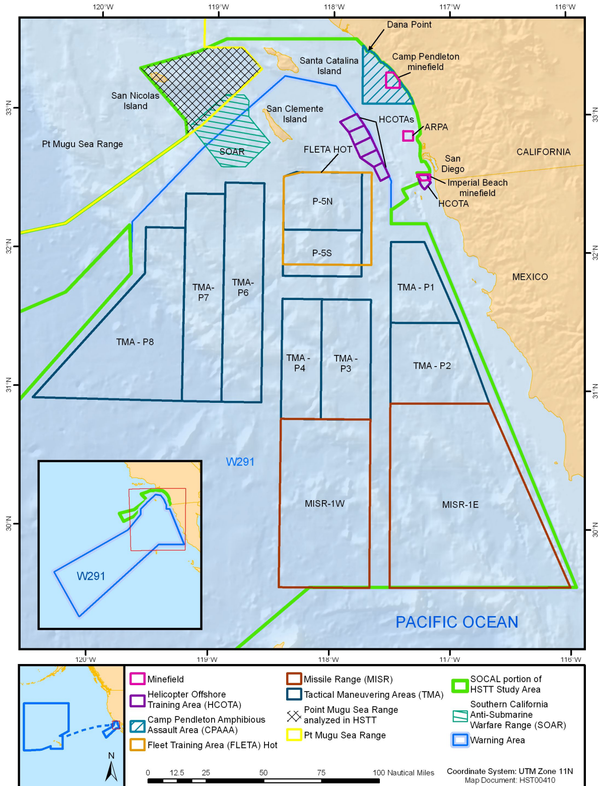
Figure 1. Map of the Southern California (SOCAL) Range Complex, a portion of the Hawaii-Southern California Testing and Training (HSTT) Study Area. SOAR, the region west of San Clemente Island, is part of SCORE and largely overlaps with it. Source: Department of the Navy (DoN) (2018).
