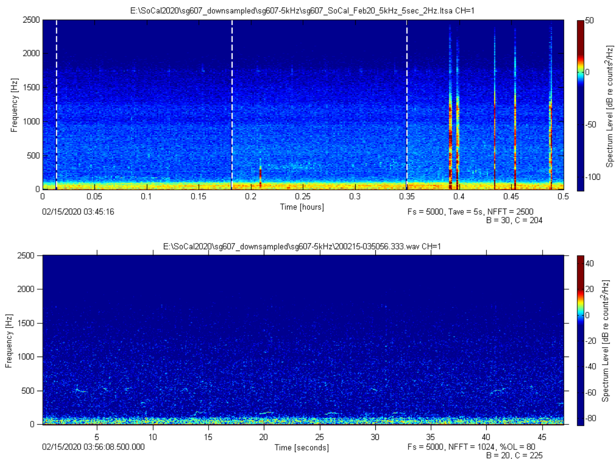
Figure F-1. Example of an LTSAs of humpback vocalizations graded as a “1”, on a scale of 1-5.
