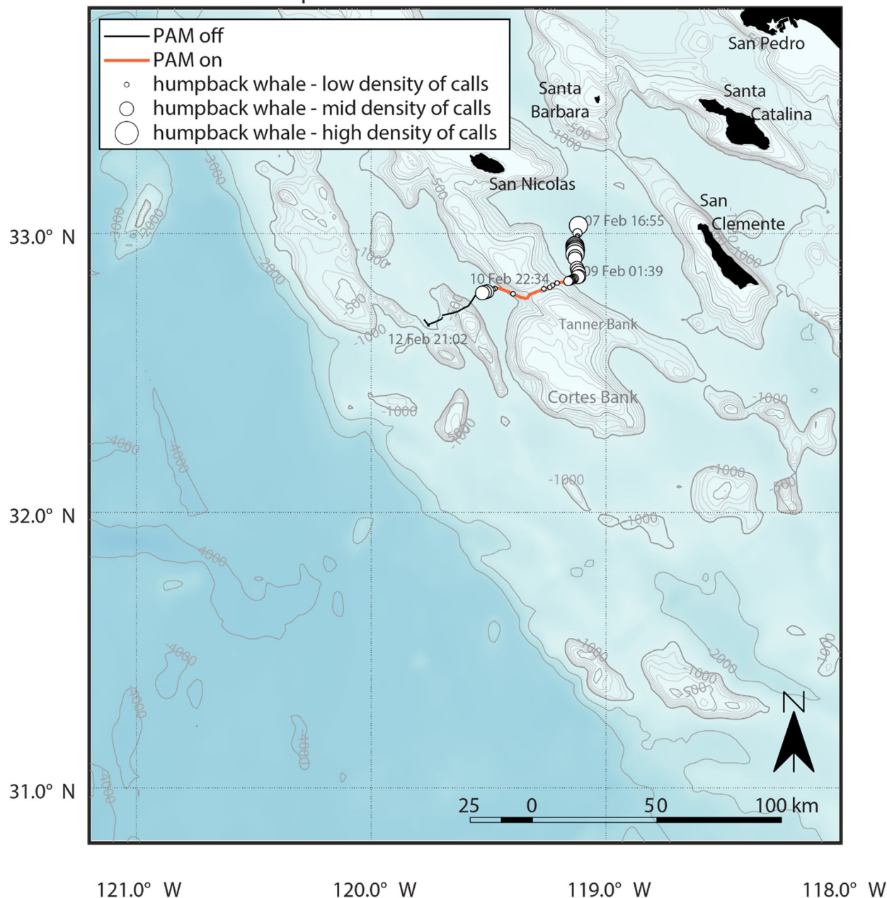
Figure 17. Shelf glider (SG639) track (orange when recording system was on) and locations of the glider when humpback whale sounds were present (white circles). Circle size is scaled to the estimated density of detections (qualitative score from 1 to 5; see Section 2.4 and Appendix F).
