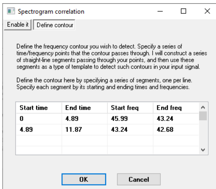
Figure A-1. Spectrogram correlation kernel parameters in Ishmael for the blue whale detector. The contour width was 2 Hz.
