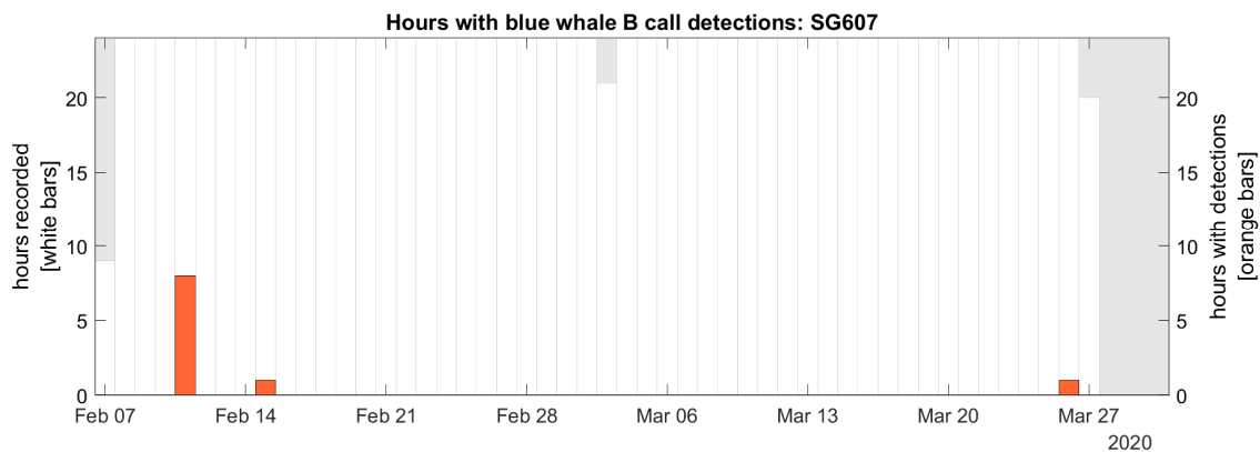
Figure 6. Number of hours per day containing detections of blue whale B calls on the abyssal glider. Gray background indicates a period of no data.
