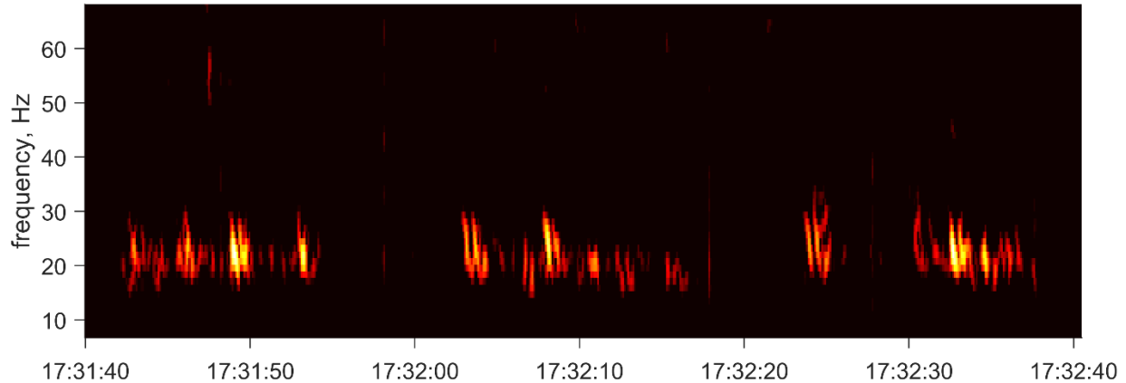
Figure 8. Example pulses from several fin whales recorded on 8 February 2020 on the abyssal glider. (Spectrogram parameters: frame length 0.41 s, FFT size 0.82 s, overlap 75%, Hamming window)
