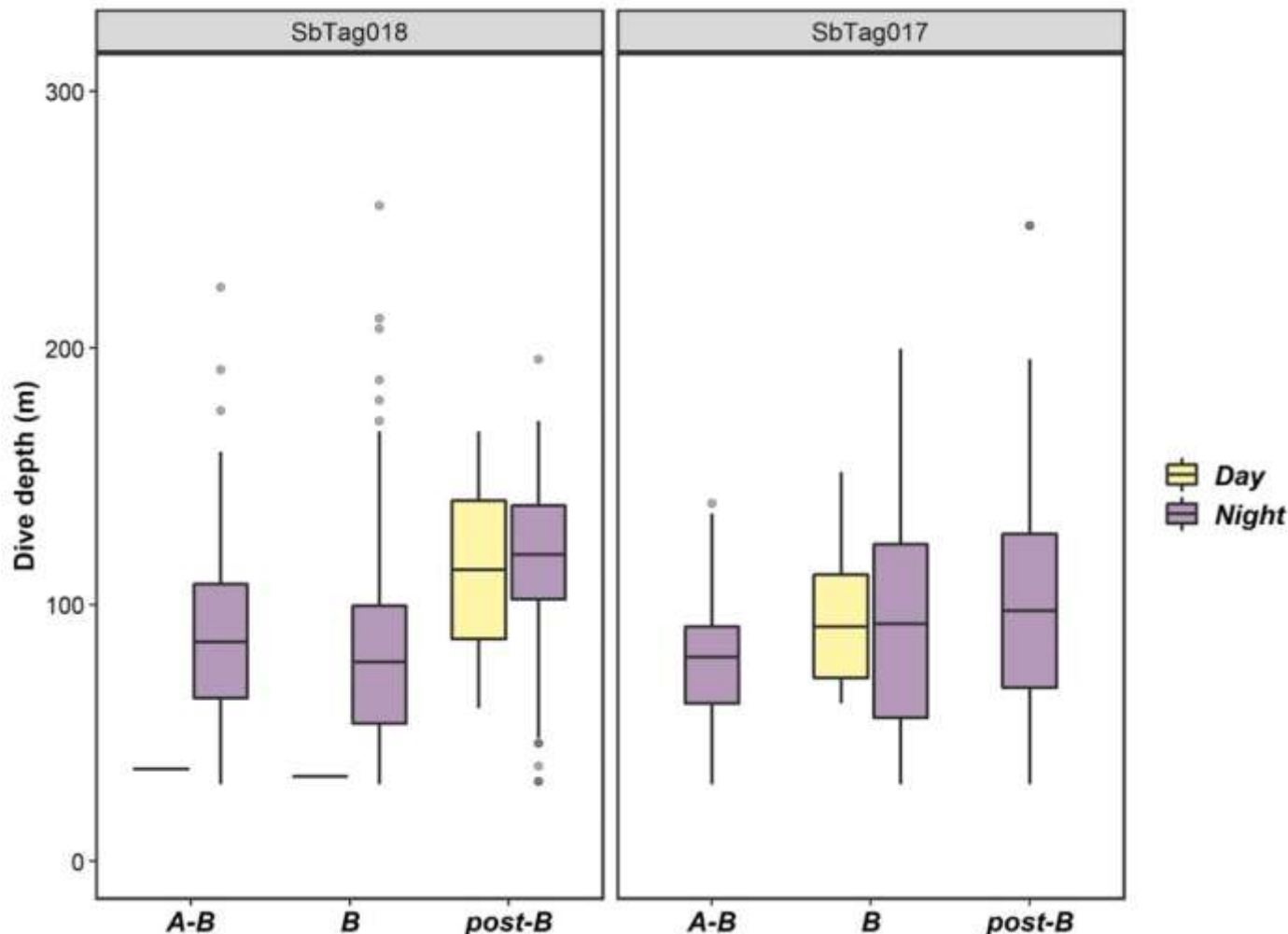
Figure 3.3.2-1. Distribution of dive depths by exposure/SCC phase by day/night, for each rough-toothed dolphin with sufficient dive and surfacing data coverage. Note the relatively lack of day-time dives reflects lower day-time dive rates for rough-toothed dolphins (Shaff and Baird, 2021). Lower and upper hinges correspond to the first and third quartiles (25 th and 75 th percentiles) and the upper and lower whiskers extend from the hinges to +/- 1.5*IQR (interquartile range), respectively. The horizontal line within each box represents the median value, and outliers are shown as gray points.
