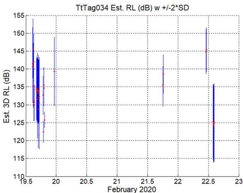
Figure 3.2.2-19. TtTag034 estimated RLs (red points) with +/- 2*SD whiskers over a 3.5-day period (GMT). Crawl data used for these RL estimates was re-routed around land.
