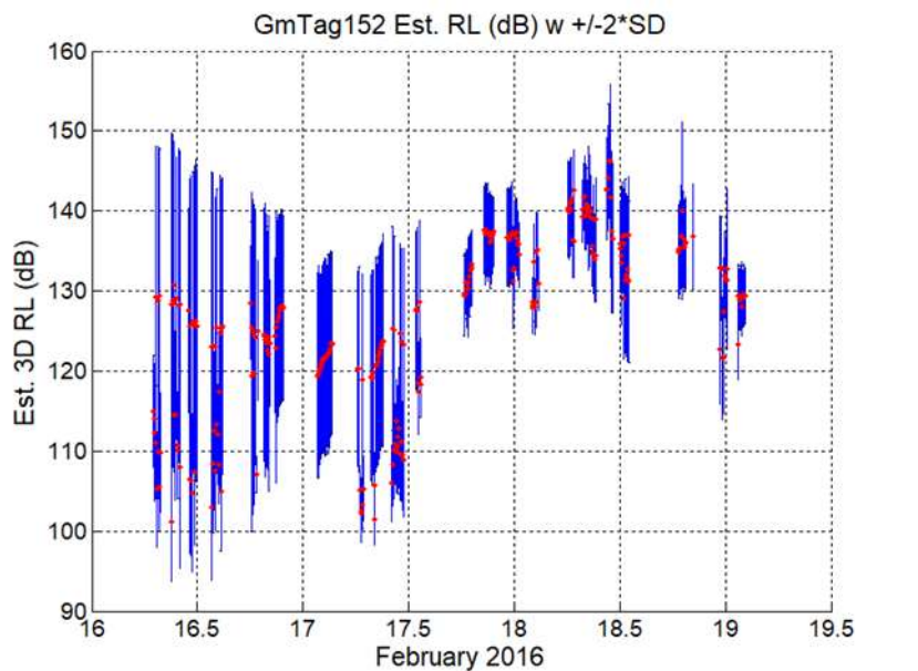
Figure 3.2.2-10. Estimated 3D RLs (red points) with \pm 2*SD whiskers for GmTag152 over a 3.5-half day period (X-axis scale in days GMT).
