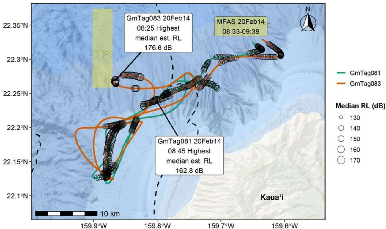
Figure 3.3.1-3. Movements of GmTag081 and GmTag083 during Phase B (MFAS use) of the Feb 2014 SCC event, highlighting the relationship between whale proximity to source and RLs (RL). Crawl tracks are colored by tag ID (only Phase B shown); see text for description of phases. Median estimated RLs are plotted as open circles, with the size of the circle scaled to RL level. Shaded box represents area of ship activity during blocks of MFAS use (for time periods as specified), and corresponding colored diamond point represents the mean ship location for that time period. The dashed black line represents the PMRF boundary.
