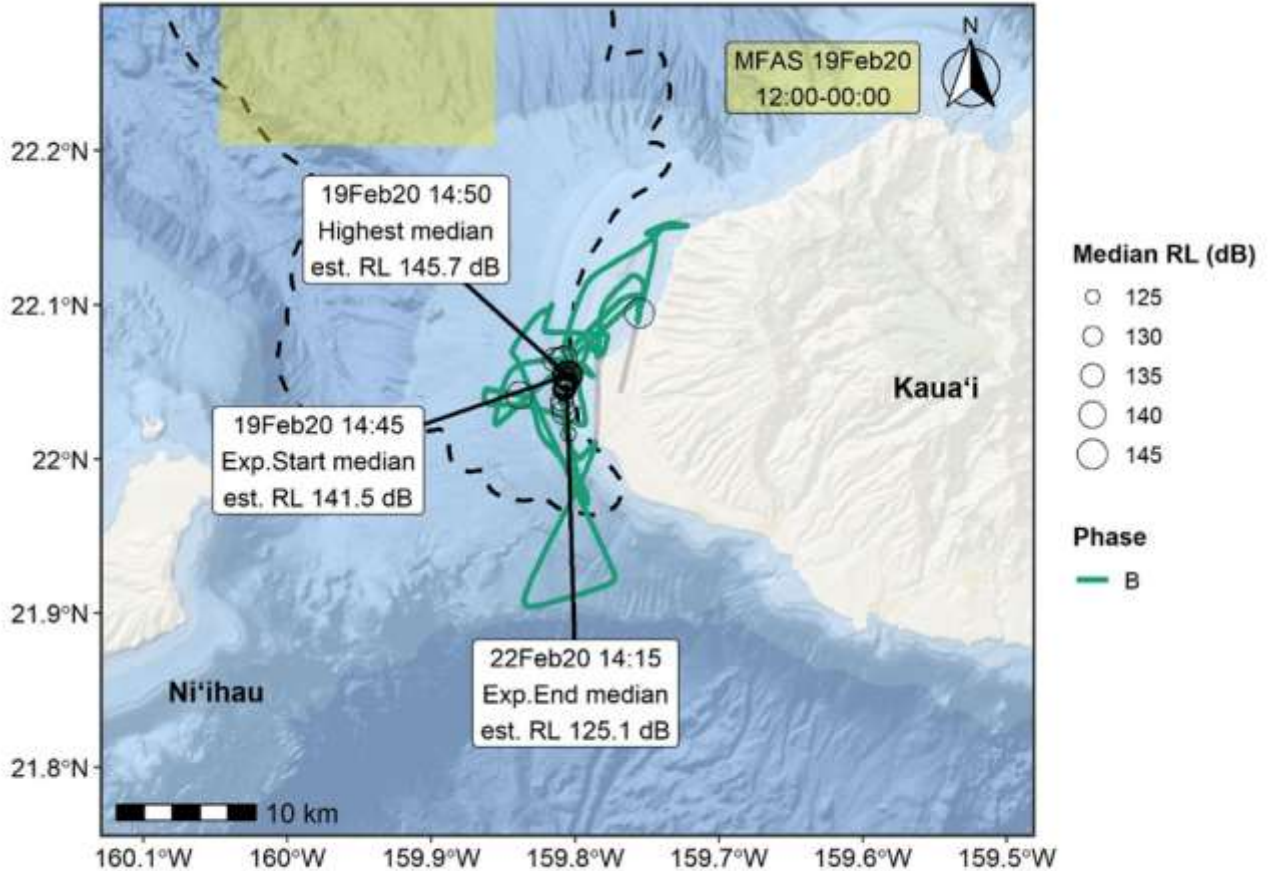
Figure 3.3.2-5. Movements of TtTag034 during Phase B of the February 2020 SCC. Gray-shaded tracks show the original crawl track prior to re-routing around land. Median estimated RLs (RL) are plotted as open circles, with the size of the circle scaled to RL level. The shaded box represents the southernmost area of ship activity for the time period specified (see Figure 3.3.2-4 for more details on ship activity areas). The dashed black line represents the PMRF boundary.
