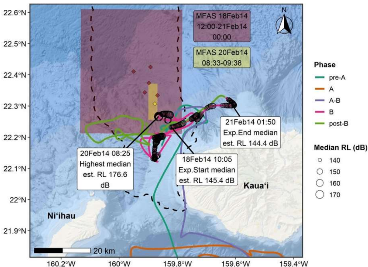
Figure 3.3.1-2. Movements of GmTag083 during the Feb 2014 SCC event. Crawl tracks are colored by phase; see text for description of phases. Median estimated RLs (RL) are plotted as open circles, with the size of the circle scaled to RL level. Shaded boxes represent area of ship activity during blocks of MFAS use (for time periods as specified), and corresponding colored diamond points represent the mean ship location for that time period. For the red-shaded box, the five mean ship position points correspond to mean positions at 12-hour intervals over that time period. The dashed black line represents the PMRF boundary.
