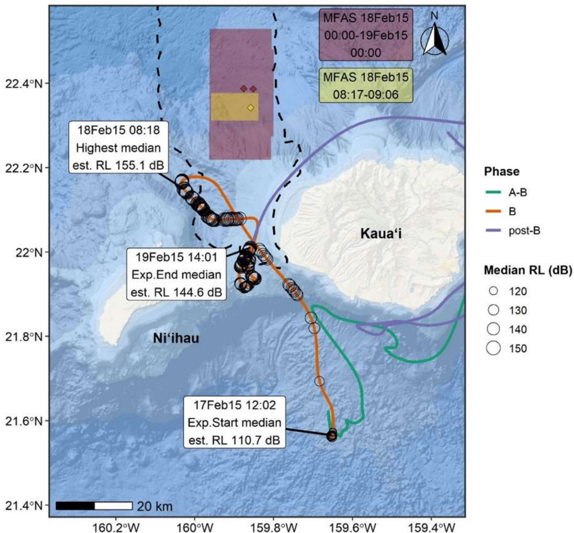
Figure 3.3.2-3. Movements of SbTag015 during the February 2015 SCC event. Crawl tracks are colored by phase; see text for description of phases. Note: only three days of data post-Phase B are plotted, and tracks before Phase A and during Phase A are not shown. Median estimated RLs (RL) are plotted as open circles, with the size of the circle scaled to RL level. Shaded boxes represent area of ship activity (for time periods as specified), and corresponding colored diamond points represent the mean ship position for that time period. For the red-shaded box, the two mean ship position points (red diamonds) correspond to mean positions at 12-hour intervals over that time period. The dashed black line represents the PMRF boundary.
