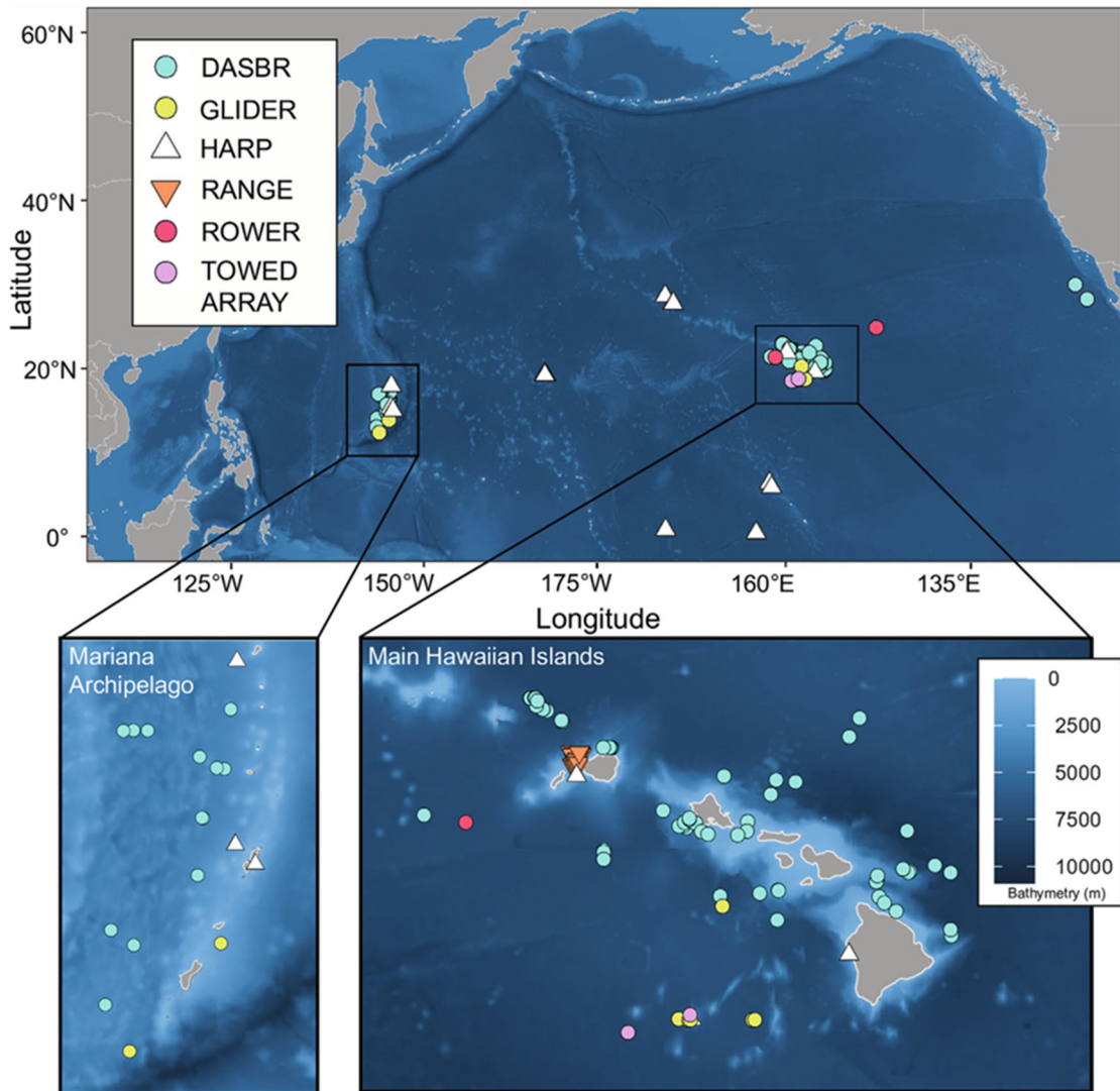
Figure 19. Cross Seamount beaked whale distribution across the North Pacific Ocean. PMRF data are shown as orange triangles. Used with permission from McCullough et al. (2023).
