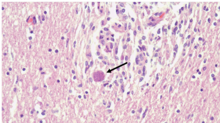
Figure 3. Toxoplasma cyst (arrow) evident upon histopathology in the brain of the stranded bottlenose dolphin.
