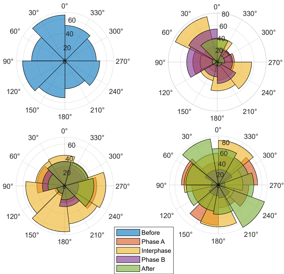
Figure 16. Top left: Track bearing values between 5-minute crawl-modeled track steps, with all of MdTag017 being baseline data, while the data for the other three whales is broken down by baseline/before, during, and after exposure periods. Top right: MdTag020. Bottom left: MdTag021. Bottom right: MdTag022.
