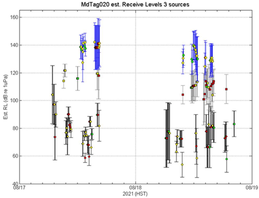
Figure 7. Estimated received levels for hull-mounted MFAS (blue) and helicopter-dipping (grey) and sonobuoy (black) MFAS for MdTag020 provided as maximum median +/- 2 standard deviations in 5 minute bins. The relative amount of sonar activity in each bin is indicated as a stoplight color coded symbol with green for lowest activity, yellow for moderate, and red for higher activity.
