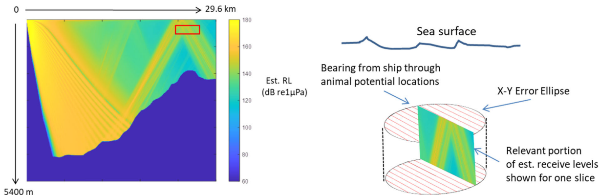
Figure 1. Left: Example of a single slice from ship MFAS source full depth maximum distance estimated received levels in units of dB re 1\mu\text{Pa} . Dark color indicates the seafloor, highlighting the steep angle limitation close to a source. The red insert box illustrates the potential location in this slice of the animal location using the 95% CI ellipse and depth information. Right: The same red box depicted as one of the radial slices from the MFAS source through the error ellipse of the whale position, demonstrating how RLs are estimated for animals during a dive.
