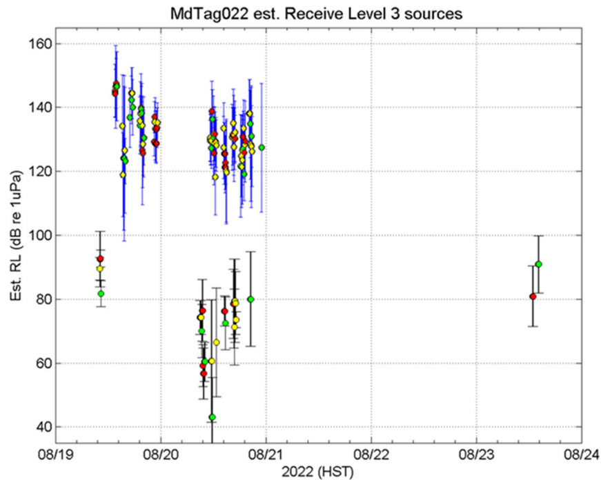
Figure 11. Estimated received levels for hull-mounted MFAS (blue) and sonobuoy MFAS (black) for MdTag022 provided as maximum median +/- 2 standard deviations in 5 min bins. The relative amount of sonar activity in each bin is indicated as a stoplight color coded symbol with green for lowest activity, yellow for moderate, and red for higher activity.
