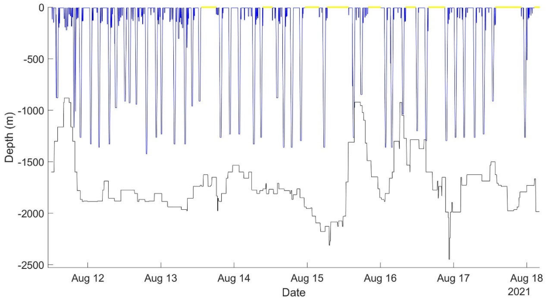
Figure 3. Dive profile for MdTag020 in blue plotted over the corresponding bathymetric depths in black at each 5-minute track position. Yellow bars indicate periods when there were no dive or surface data available.
