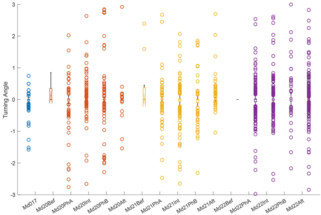
Figure 19. Track turning angle values between 5-minute crawl-modeled track steps, with all of MdTag017 being baseline data, while the data for the other three whales is broken down by baseline/before, during, and after exposure periods.
