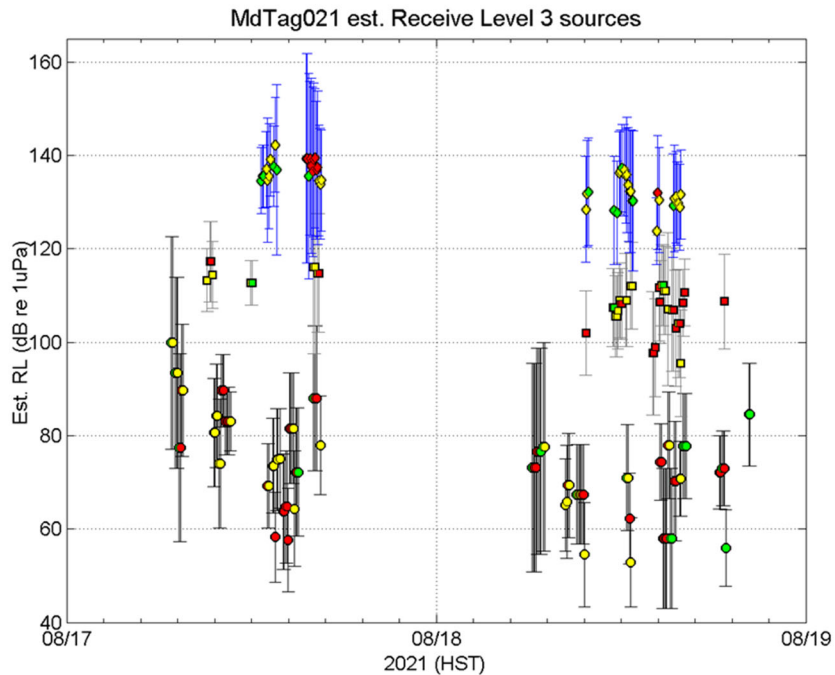
Figure 9. Estimated receive levels for hull-mounted MFAS (blue) and helicopter-dipping (gray) and sonobuoy (black) MFAS for MdTag021 provided as maximum median +/- 2 standard deviations in 5 min bins. The relative amount of sonar activity in each bin is indicated as a stoplight color coded symbol with green for lowest activity, yellow for moderate, and red for higher activity.
