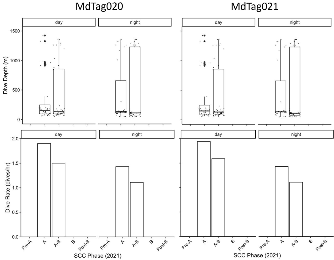
Figure 15. Top left: Boxplot showing dive depths of MdTag020 by SCC Phase and time of day. Bottom left: Barplot showing dive rates of MdTag020 by SCC Phase and time of day. Top right: Boxplot showing dive depths of MdTag021 by SCC Phase and time of day. Bottom right: Barplot showing dive rates of MdTag021 by SCC Phase and time of day.
