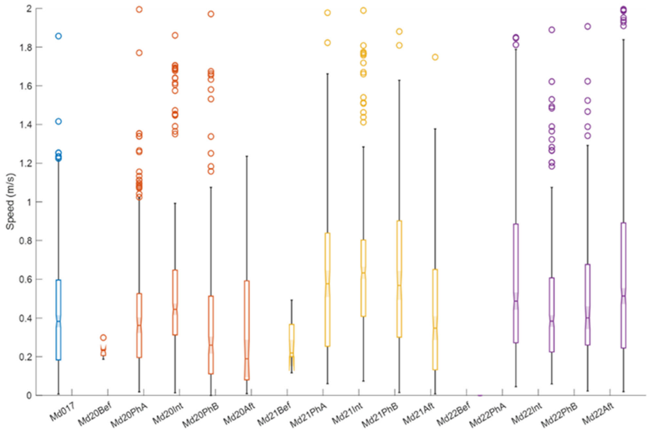
Figure 18. Track speed values between 5-minute crawl-modeled track steps, with all of MdTag017 being baseline data, while the data for the other three whales is broken down by baseline/before, during, and after exposure periods.
