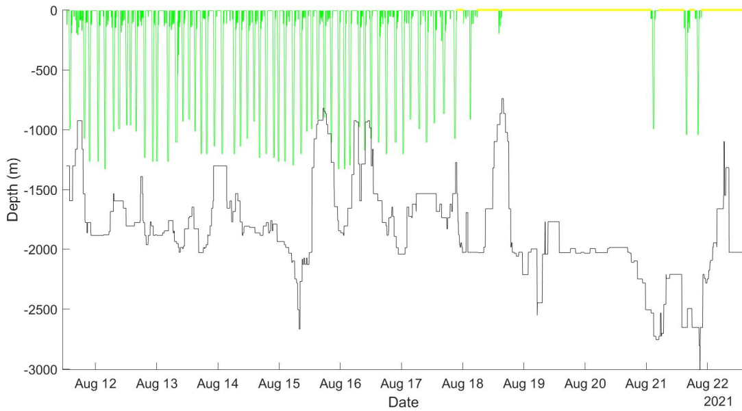
Figure 4. MdTag021 dive profile (in green) over the corresponding bathymetric depths in black throughout the track. Periods when there are no dive or surface data are highlighted in yellow.
