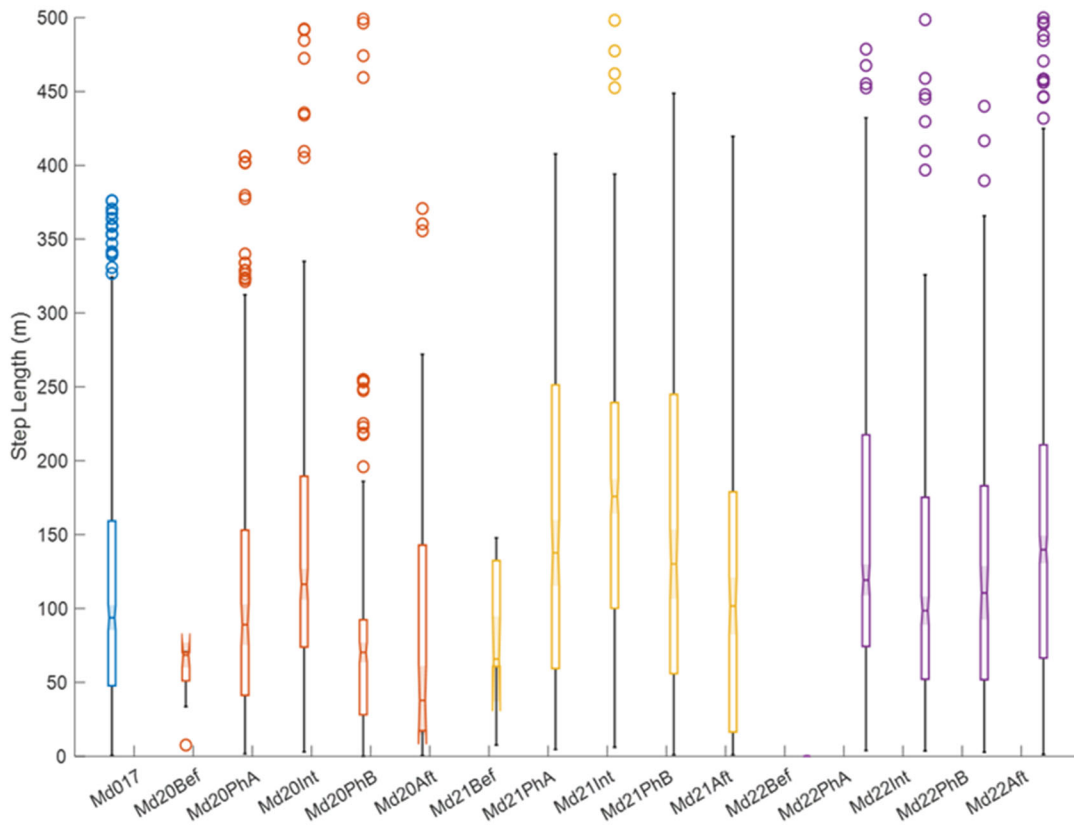
Figure 17. Track step length values between 5-minute crawl-modeled track steps, with all of MdTag017 being baseline data, while the data for the other three whales is broken down by baseline/before, during, and after exposure periods.
