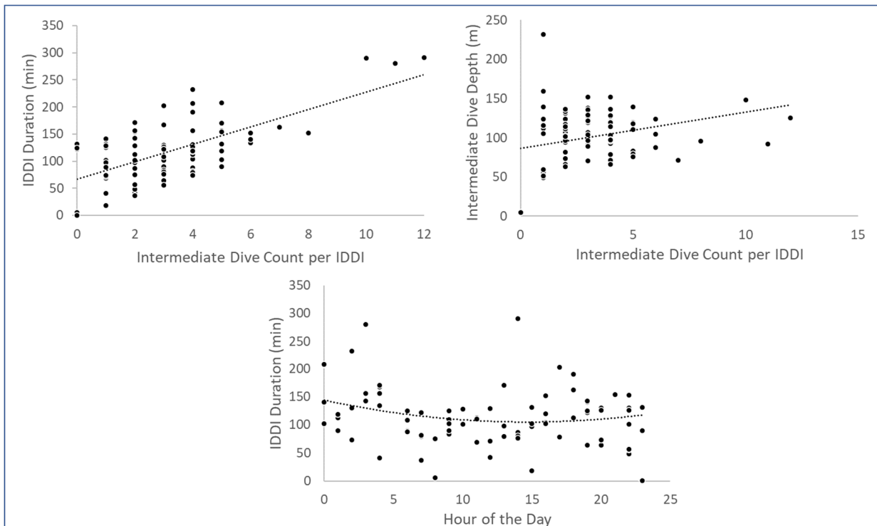
Figure 5. Top left: IDDI intermediate dive count compared to overall IDDI duration (minutes.). Top right: IDDI intermediate dive count compared to intermediate dive depth (m) and. Bottom: overall IDDI duration (min) compared to the hour of day.
