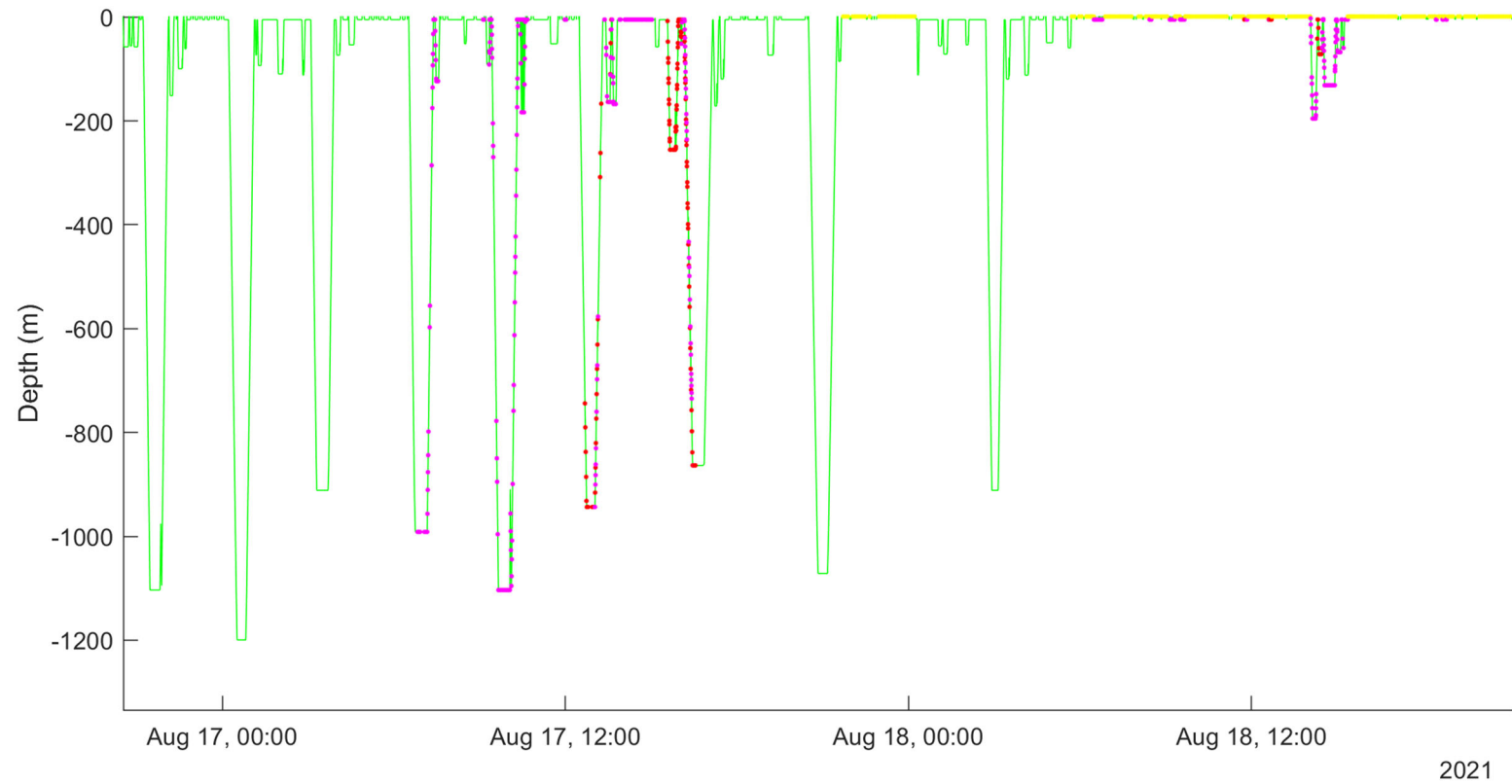
Figure 14. Dive record of MdTag021 starting August 16, 2021, at 21:00 HST through August 18, 2021, at 23:00 HST.
