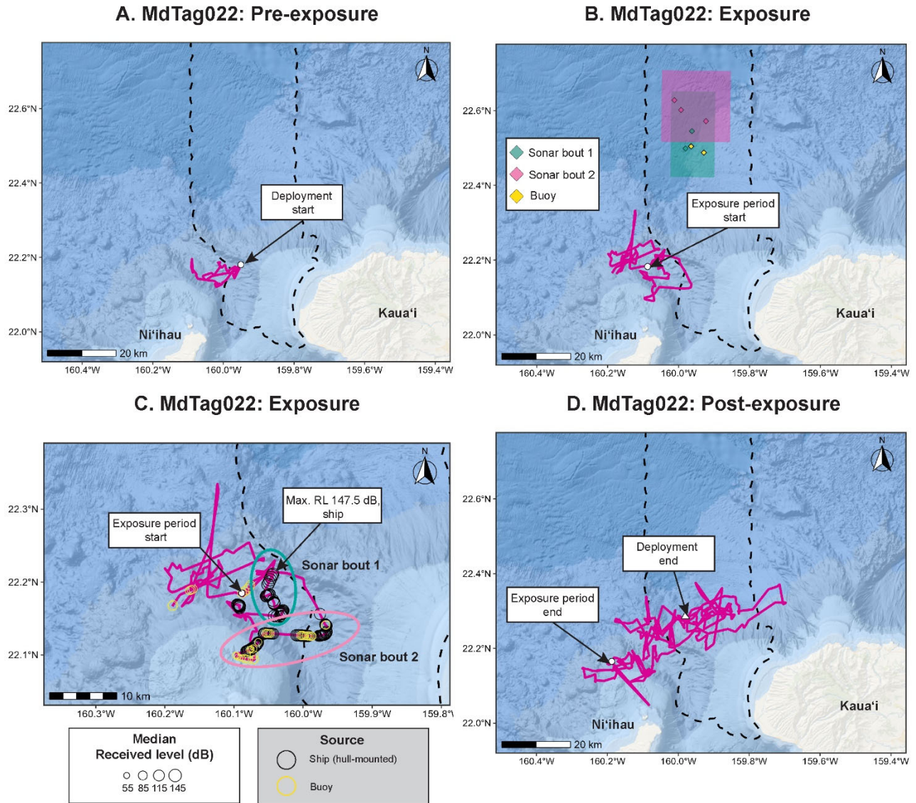
Figure 12. Movements of MdTag022 prior to, during, and after exposure periods, with corresponding median received levels (ERL) shown during the exposure period (panel C).
