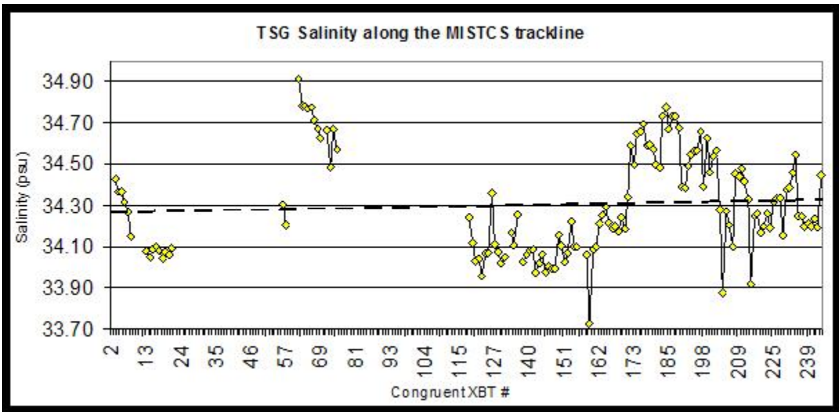
Figure 3-23. TSG Salinity along the MISTCS Trackline
