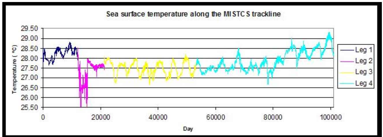
Figure 3-22. TSG Temperature and Associated Trendline along the MISTCS Trackline
