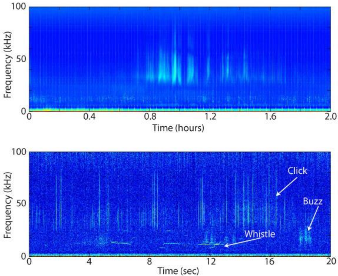
Figure 19. LTSA (top) and spectrogram (bottom) demonstrating the odontocete signal types.
