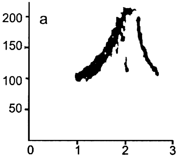
Figure 15. Example of North Pacific right whale “up-call” from McDonald & Moore 2002.
