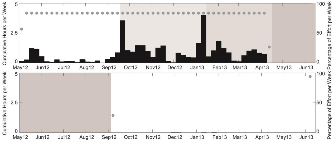
Figure 63. Weekly presence of unidentified porpoise echolocation clicks (black bars) at sites CA (top) and PT (bottom) between May 2012 and June 2013. No porpoise clicks were detected at site CB. Effort as described in Figure 46.
