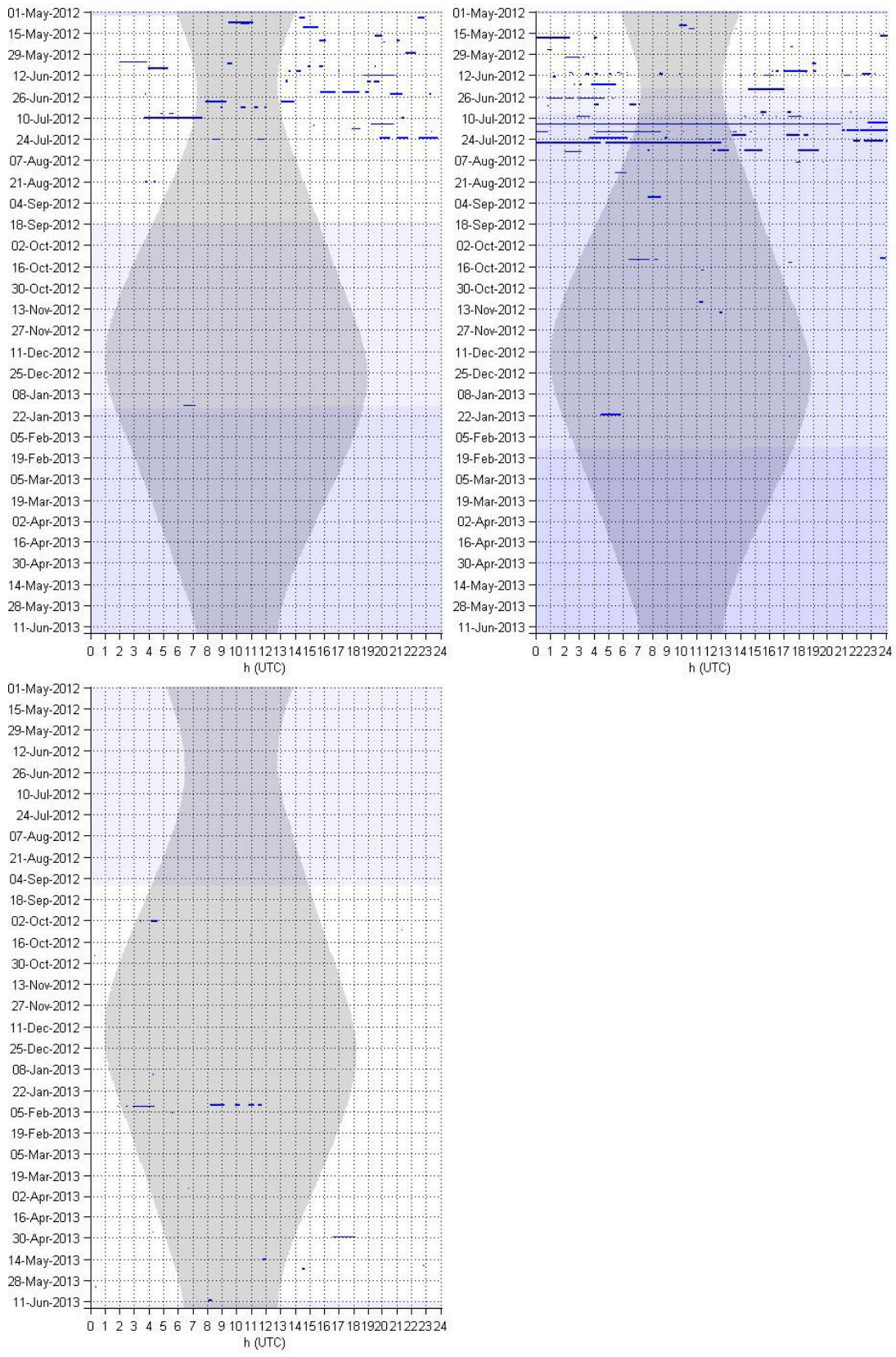
Figure 54. Killer whale whistles in one-minute bins at sites CA (top left), CB (top right), and PT (bottom). Shading is as described in Figure 38.
