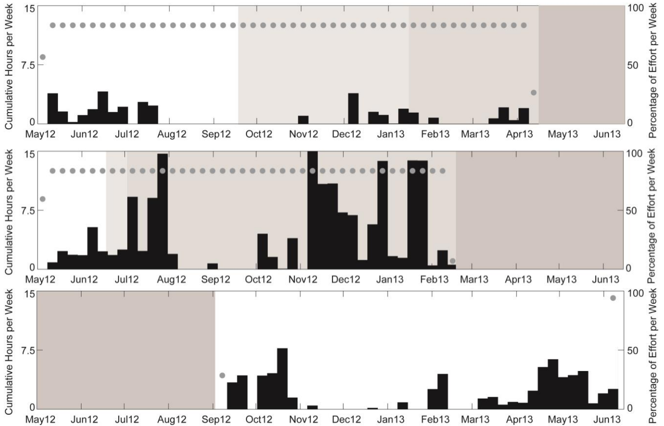
Figure 51. Weekly presence of killer whale clicks (black bars) at sites CA (top), CB (middle), and PT (bottom) between May 2012 and June 2013. Effort as described in Figure 46.
