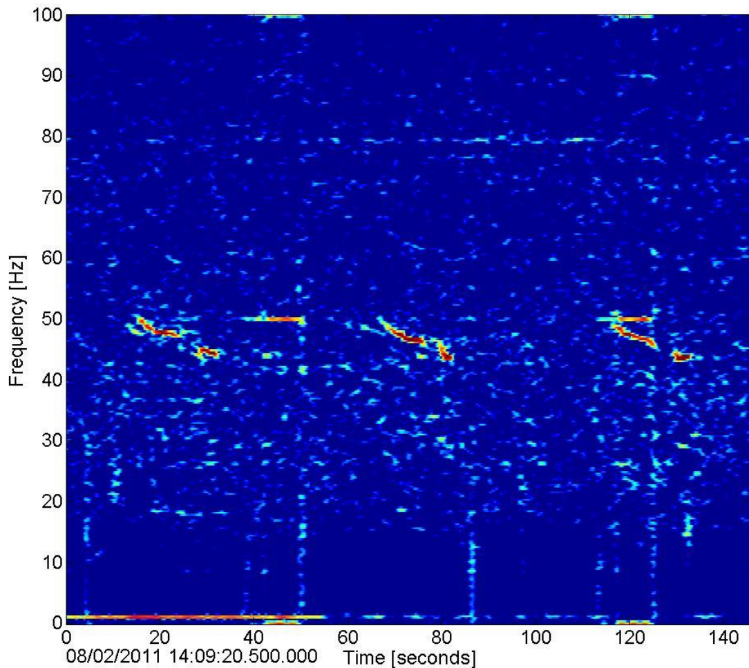
Figure 8. Spectrogram of three Northeast Pacific blue whale B calls (6,500-point FFT, 95% overlap, Hanning window) recorded at site CB. The third harmonic seen here is often the most energetic component in this call type. Pure tones at 50 Hz are related to electronic (disk) noise.
