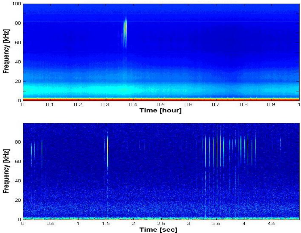
Figure 28. Example LTSA (top) and spectrogram (bottom), presumably produced by spectral aliasing of Dall's porpoise clicks (120 – 150 kHz frequency content).
