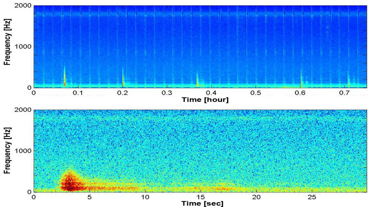
Figure 32. Five explosion events are shown at lower received levels (LTSA, top) and one example explosion (spectrogram, bottom). This explosion type shows a slower onset in comparison to the examples in Figure 31, suggesting a more distant source.
