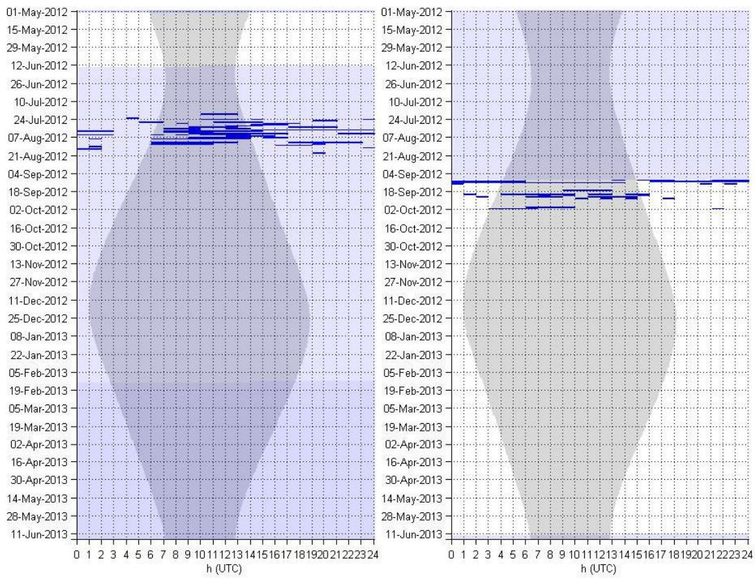
Figure 39. Central Pacific blue whale calls in hourly bins at sites CB (left) and PT (right). Shading is as described in Figure 38.
