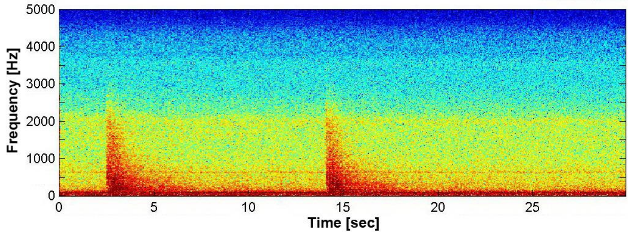
Figure 31. Two explosions are shown with rapid onset and extended reverberation.
