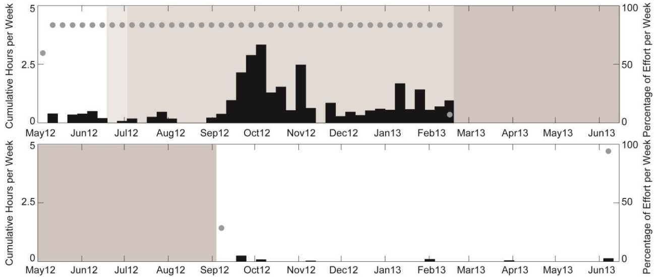
Figure 61. Weekly presence of Stejneger's beaked whale FM pulses (black bars) at sites CB (top) and PT (bottom) between May 2012 and June 2013. Effort as described in Figure 46.
