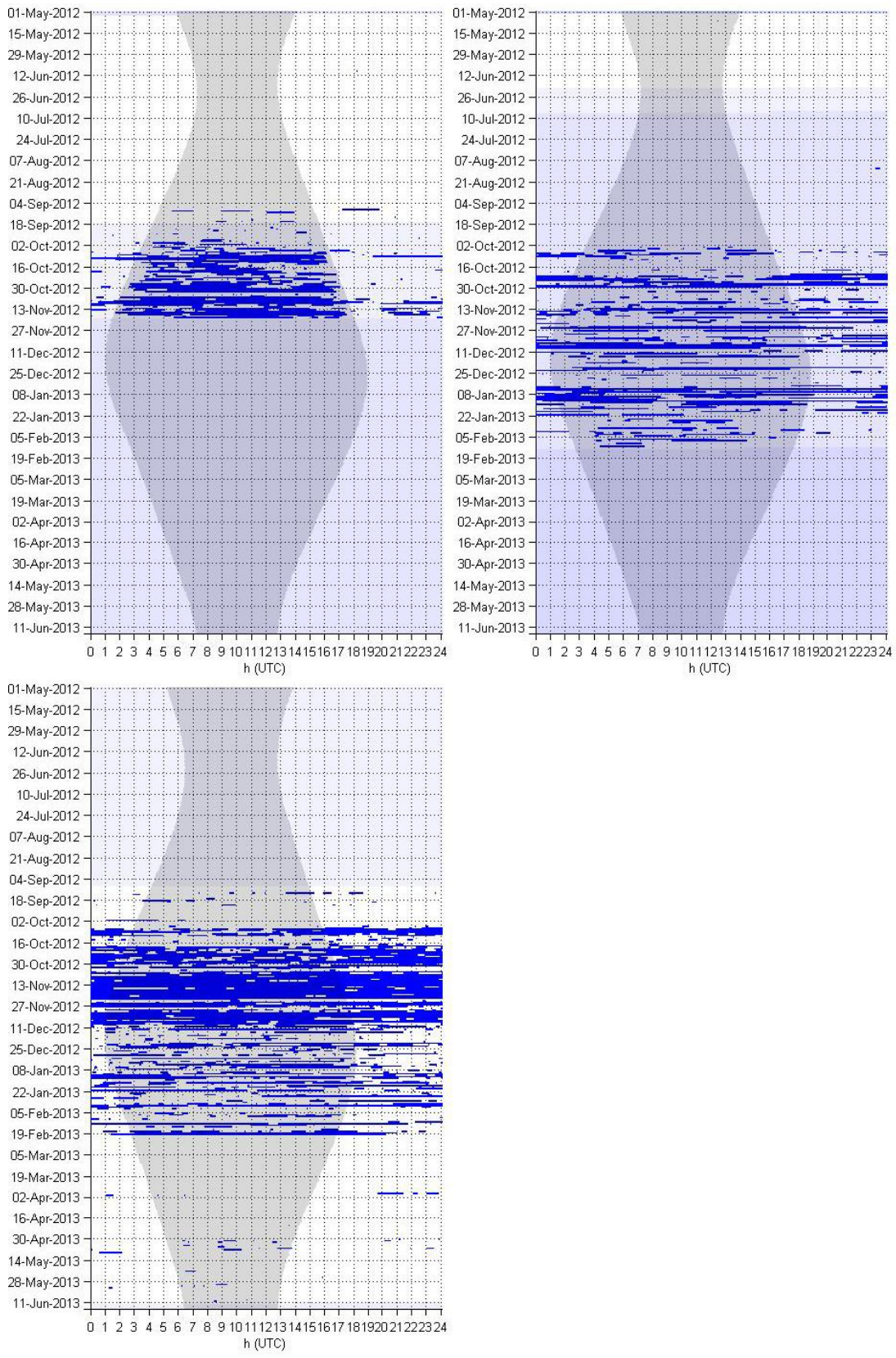
Figure 47. Humpback whale calls in one-minute bins at sites CA (top left), CB (top right), and PT (bottom). Shading is as described in Figure 38.
