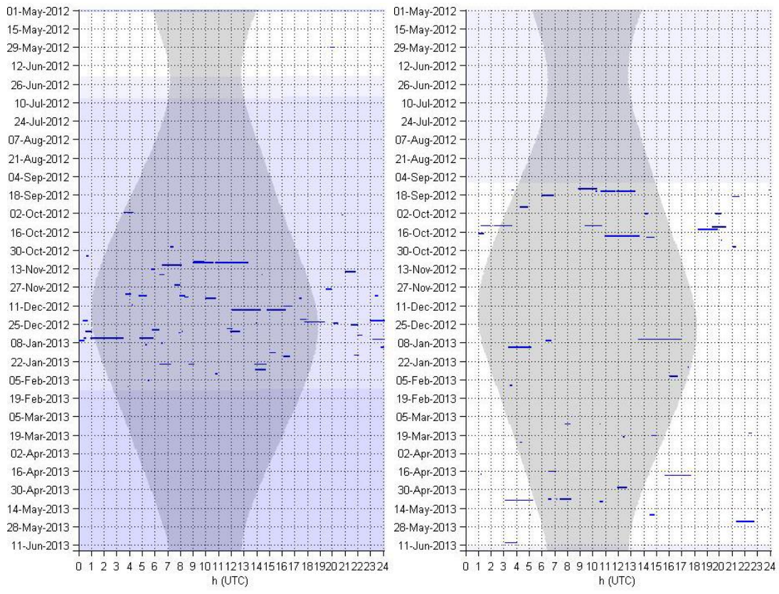
Figure 58. Baird's beaked whale echolocation signals in one-minute bins at sites CB (left) and PT (right). Shading is as described in Figure 38.
