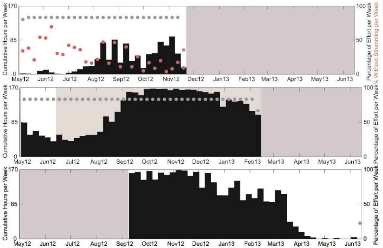
Figure 42. Weekly presence of fin whale 20 Hz calls (black bars) at sites CA (top), CB (middle), and PT (bottom) between May 2012 and June 2013. Effort as described in Figure 34.
