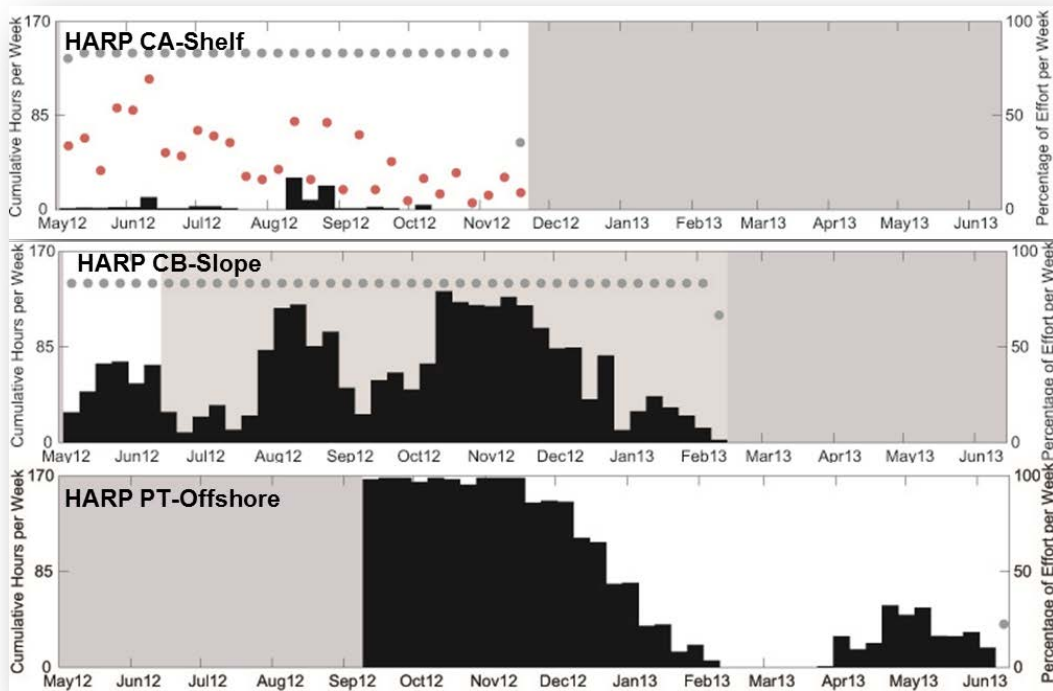
Figure 3. Weekly presence of all blue whale calls (black bars) at sites CA (top), CB (middle), and PT (bottom) between May 2012 and June 2013 (from Debich et al. 2013).
