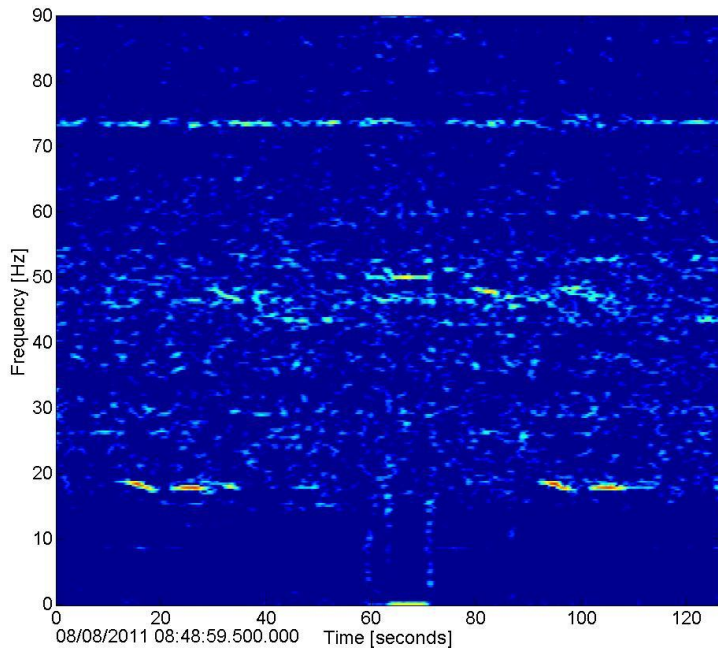
Figure 9. Spectrogram of two Central Pacific blue whale tonal calls (6,500-point FFT, 95% overlap, Hanning window) recorded at site CB.
