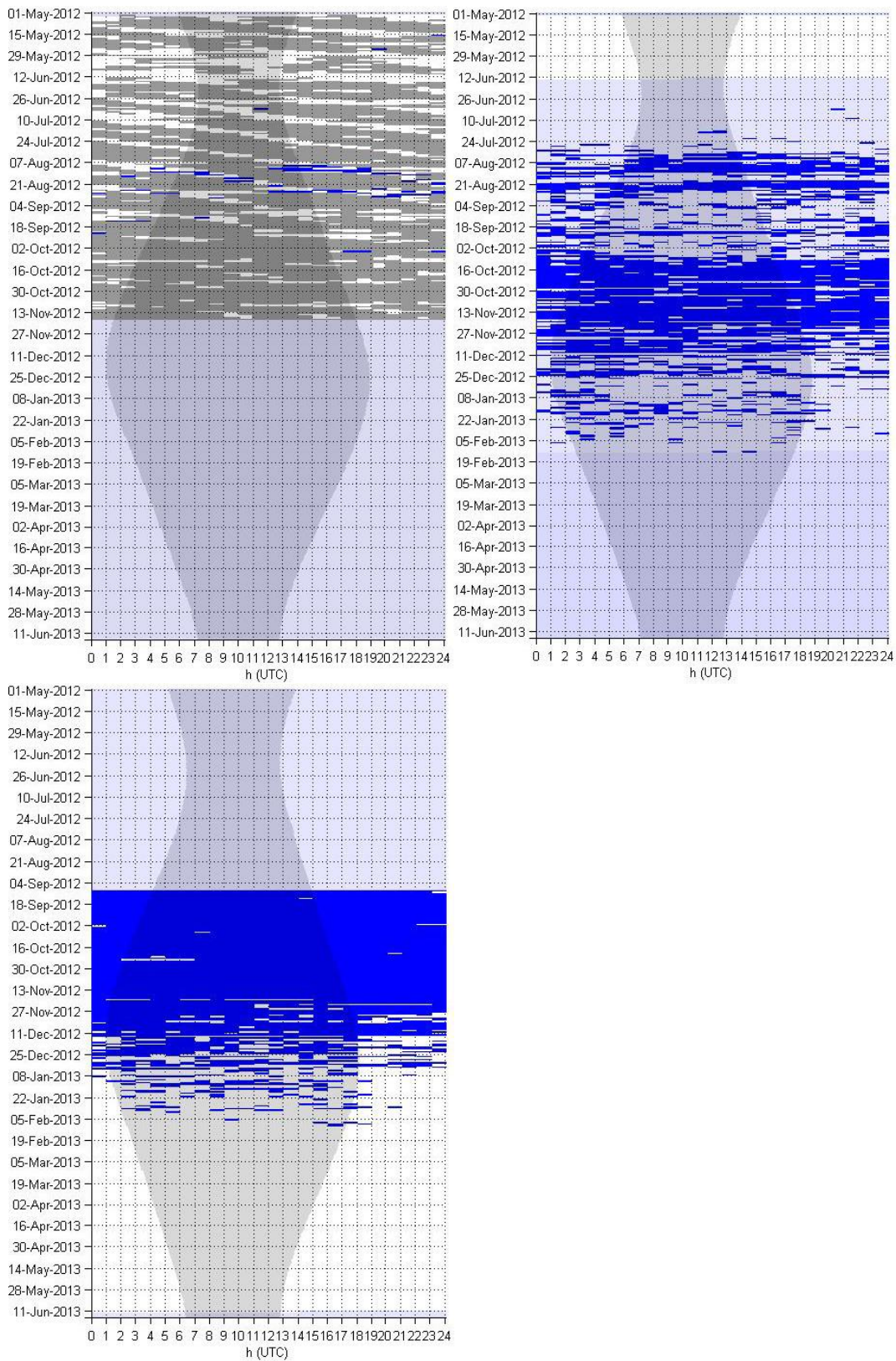
Figure 38. Blue whale B calls in hourly bins at sites CA (top left), CB (top right), and PT (bottom). Gray shading denotes nighttime and light purple shading denotes lower quality data and dark purple denotes lack of acoustic data. At site CA, dark gray shows periods of strumming causing masking.
