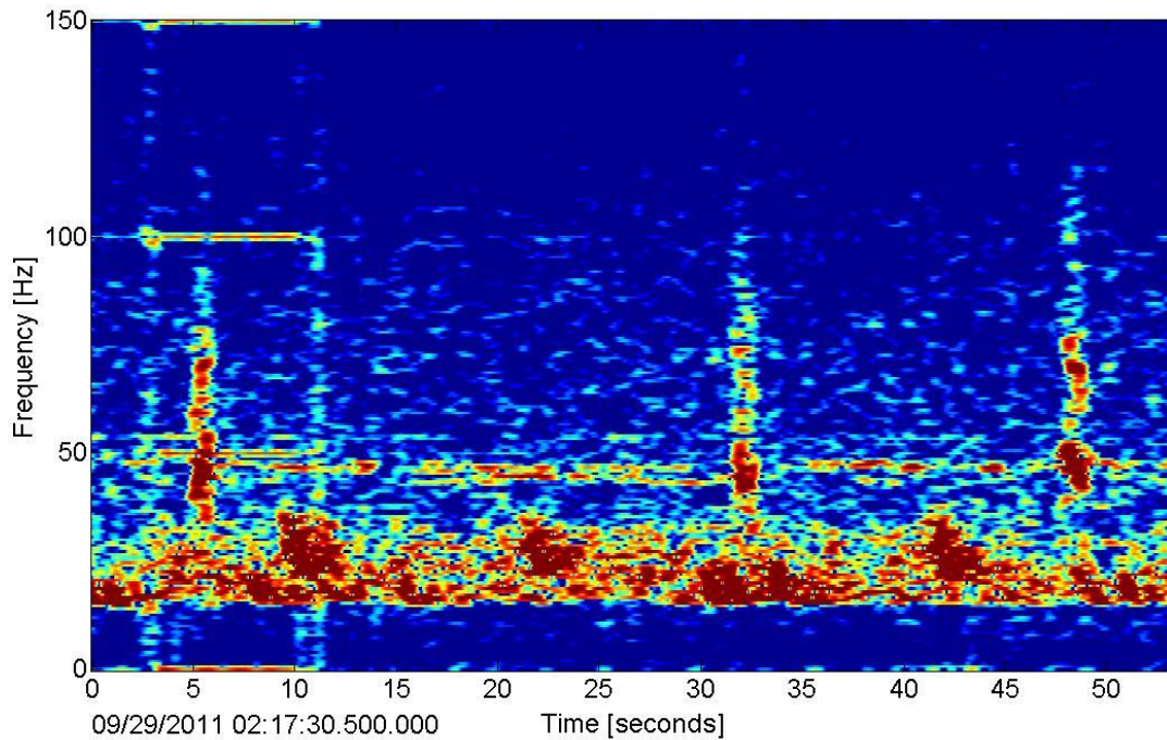
Figure 14. Spectrogram of gray whale M3 calls (3,000-point FFT, 99% overlap, Hanning window) recorded at site CB. Also note persistent “noise” in the fin whale 20 Hz band.
