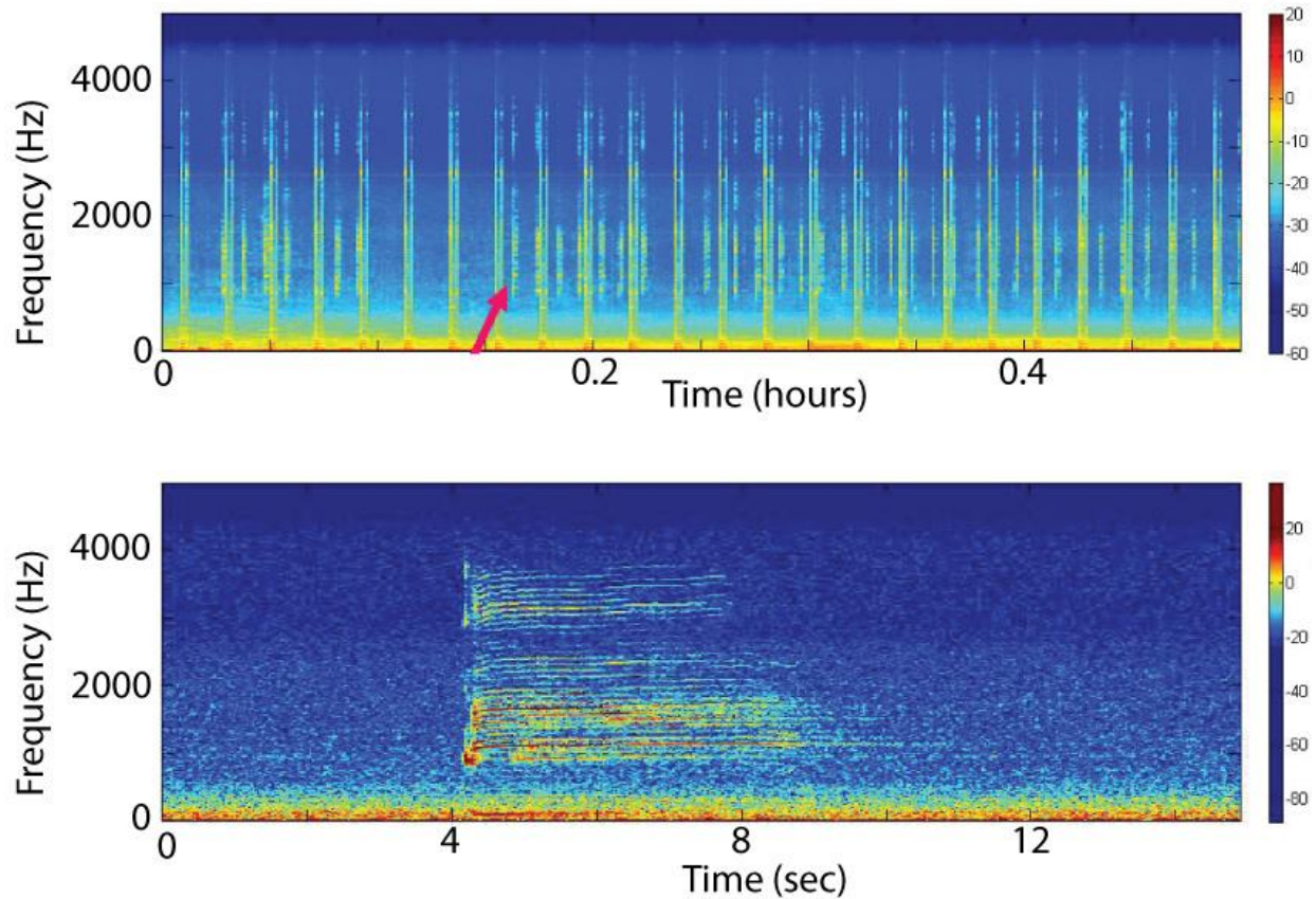
Figure 17. Minke whale boing in the LTSA (top) and spectrogram (bottom) from southern California.
