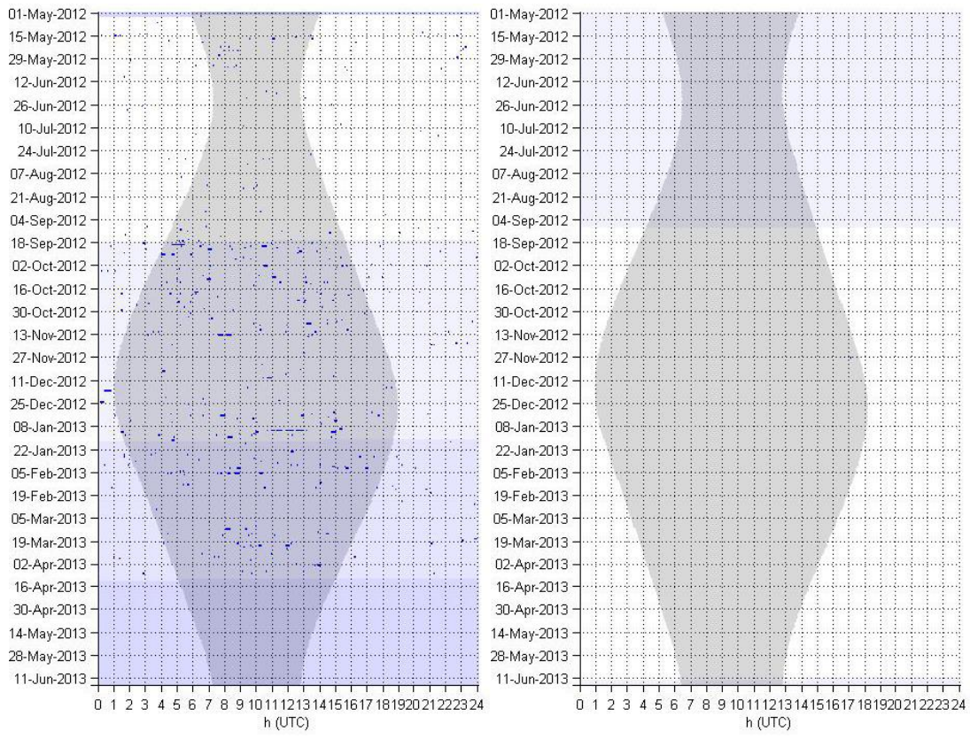
Figure 64. Unidentified porpoise echolocation clicks in one-minute bins at sites CA (left) and PT (right). Shading is as described in Figure 38.
