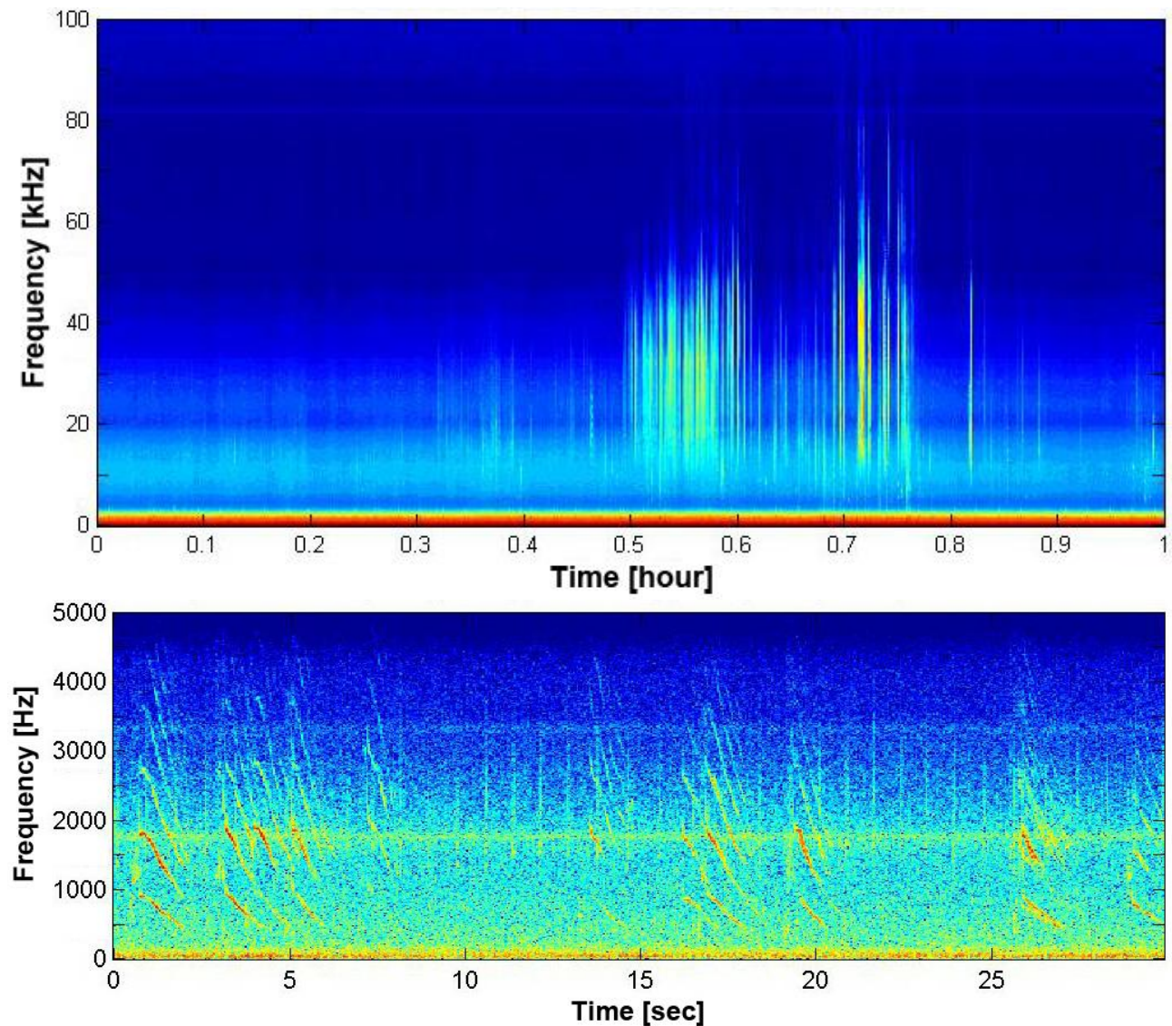
Figure 22. Killer whale echolocation clicks in the LTSA (top), whistles and pulsed calls in the spectrogram (bottom).
