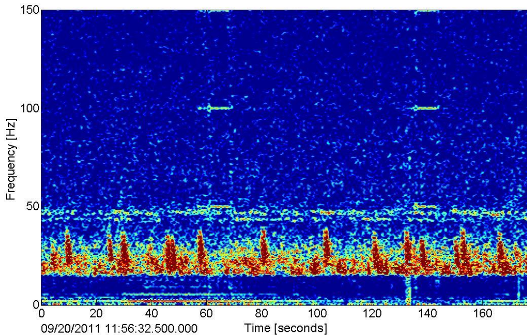
Figure 13. Spectrogram of fin whale 20 Hz nearby calls with additional energy in the “20 Hz band” resulting from more distant calls (4,000-point FFT, 99% overlap, Hanning window) recorded at site CB.
