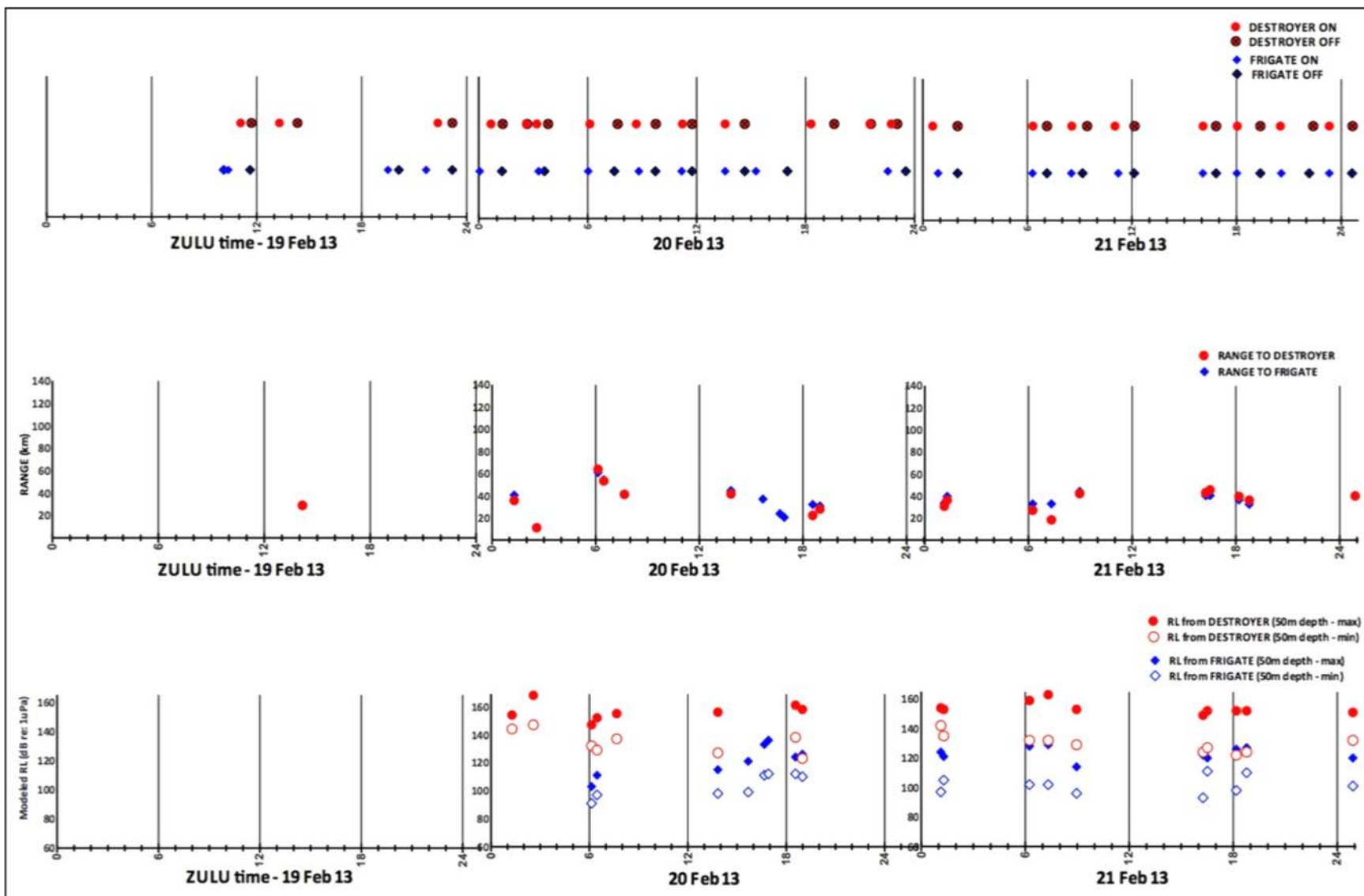
Figure 2. Timelines of sonar use (top), distance between tagged bottlenose dolphin (TtTag010) and vessels (middle), and modeled RLs (bottom). No RLs were calculated for 19 Feb 2013 due to long time intervals between MFAS pulses and locations from TtTag010.
